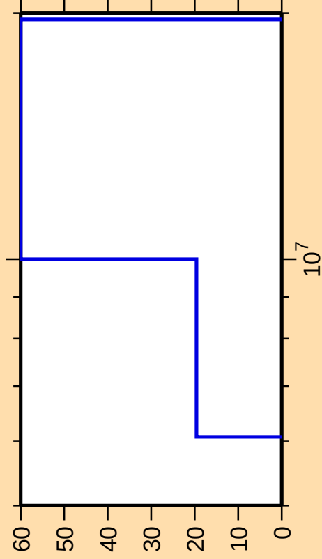
\Delta\sigma/\sigma vs. E for ^{56}\text{Fe}(n,n\alpha)
