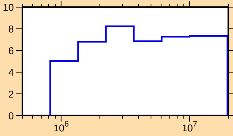
\Delta\sigma/\sigma vs. E for ^{56}\text{Fe}(\text{n,el.})
