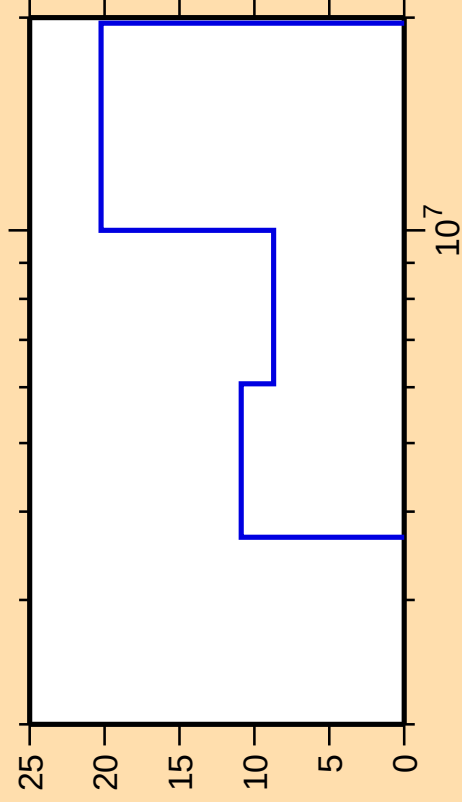
\Delta\sigma/\sigma vs. E for ^{56}\text{Fe}(\text{n},\text{ncont.})
