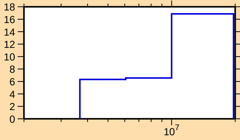
\Delta\sigma/\sigma vs. E for ^{56}\text{Fe}(\text{n},\text{inel.})
