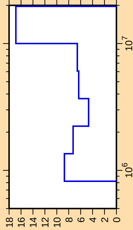
\Delta\sigma/\sigma vs. E for ^{56}\text{Fe}(\text{n,inel.})
