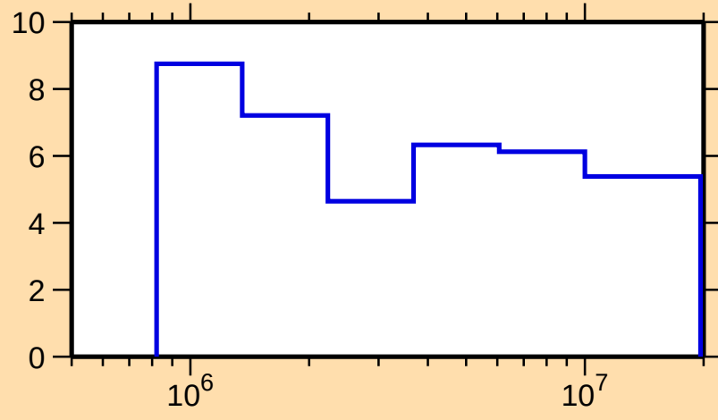
\Delta\sigma/\sigma vs. E for ^{56}\text{Fe}(\text{n,nonel.})
