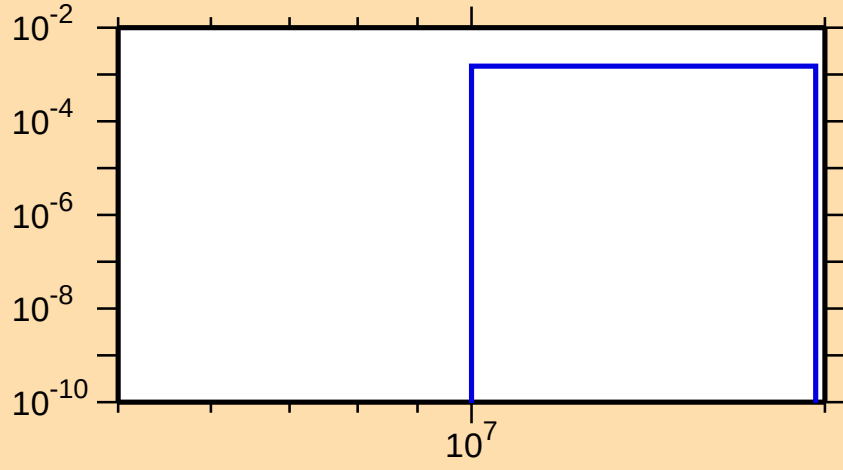
\sigma vs. E for ^{56}\text{Fe}(n,n\alpha)
