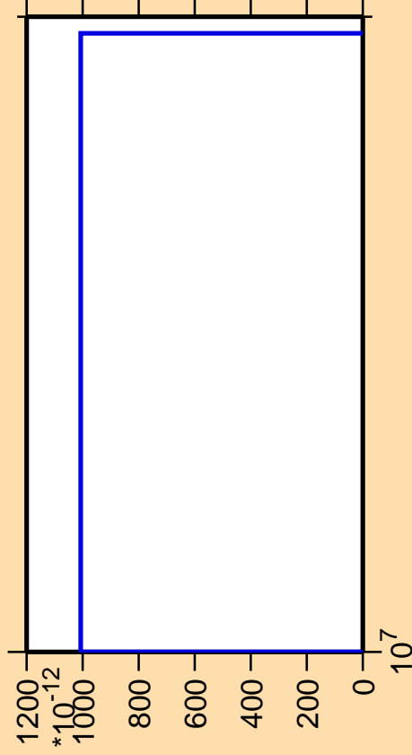
\Delta\sigma/\sigma vs. E for ^{58}\text{Fe}(n,pd)
