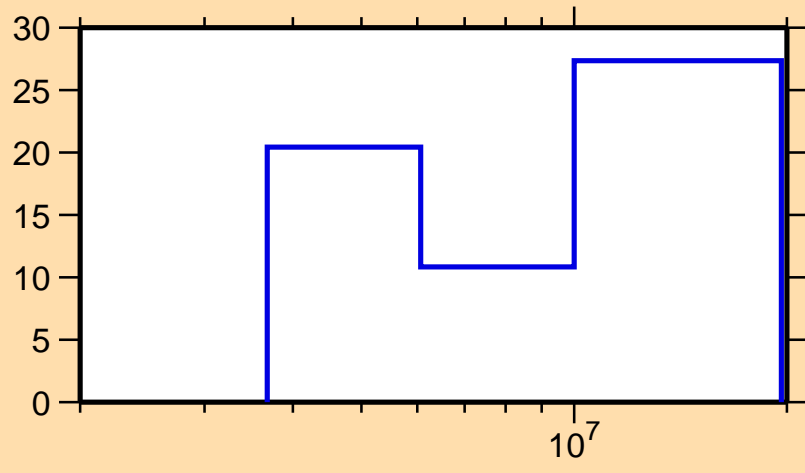
\Delta\sigma/\sigma vs. E for ^{58}\text{Fe}(n,ncont.)
