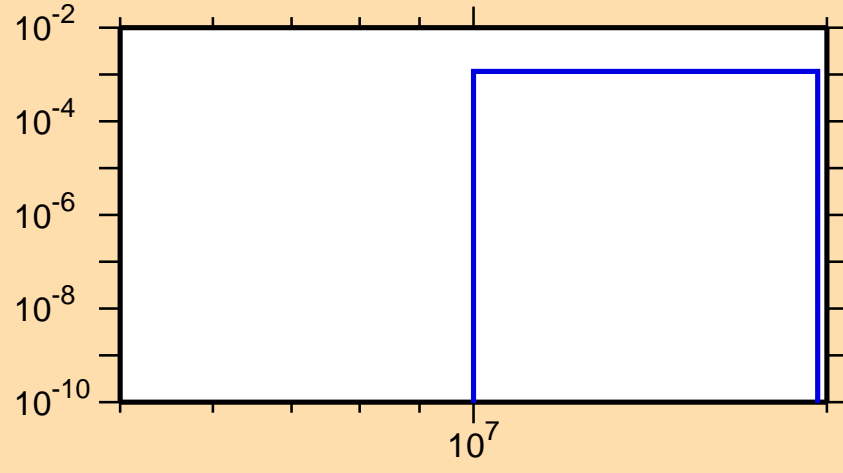
\sigma vs. E for ^{58}\text{Fe}(n,\alpha)
