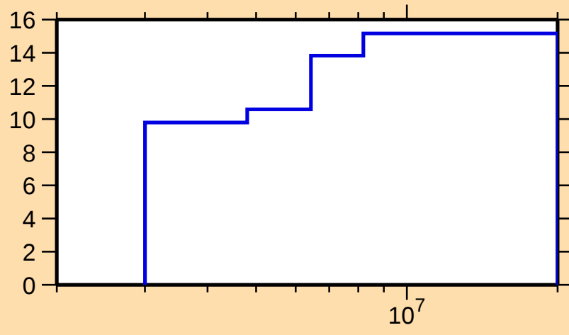
\Delta\sigma/\sigma vs. E for ^{58}\text{Fe}(\text{n},\text{el.})
