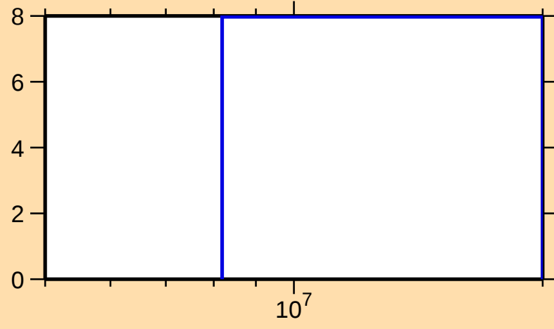
\Delta\sigma/\sigma vs. E for ^{58}\text{Fe}(n,\text{tot.})
