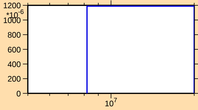
\sigma vs. E for ^{58}\text{Fe}(n,np)
