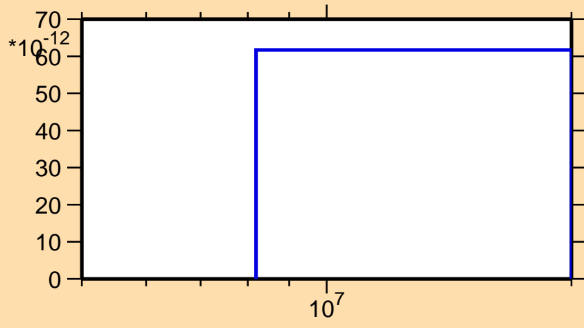
\sigma vs. E for ^{59}\text{Fe}(n,2n\alpha)
