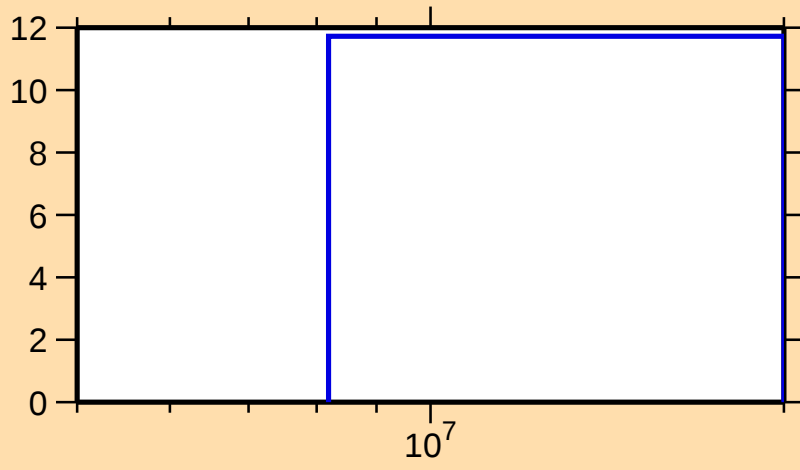
\Delta\sigma/\sigma vs. E for ^{60}\text{Fe}(n,2n)
