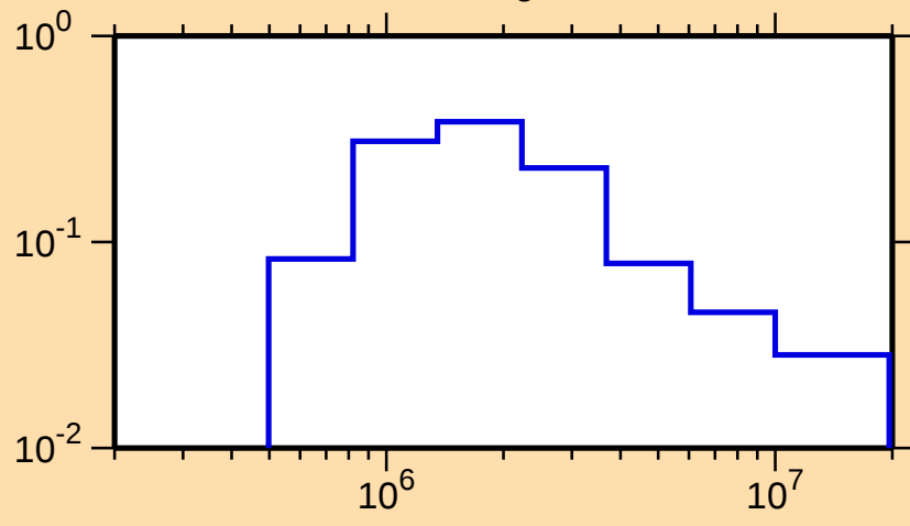
\sigma vs. E for ^{61}\text{Fe}(n,n_3)
