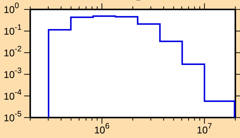
\sigma vs. E for ^{61}\text{Fe}(n,n_2)
