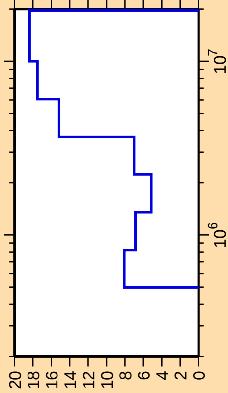
\Delta\sigma/\sigma vs. E for ^{61}\text{Fe}(n,n_3)
