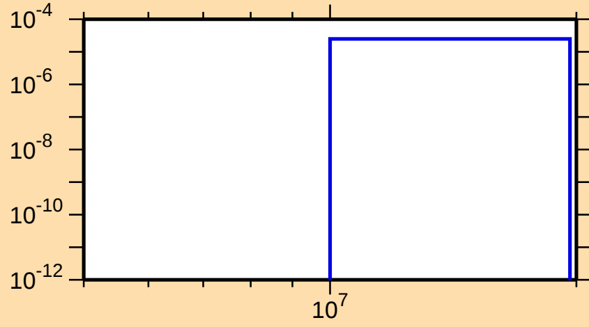
\sigma vs. E for ^{61}\text{Fe}(n,n\alpha)
