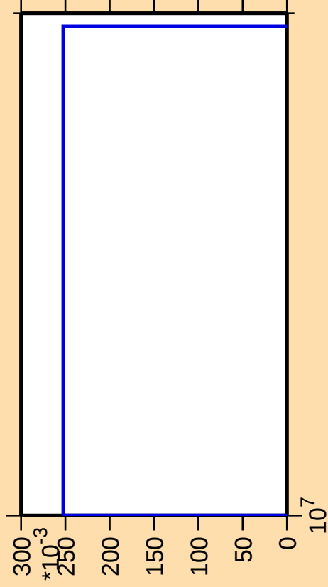
\Delta\sigma/\sigma vs. E for ^{61}\text{Fe}(n,\text{nt})
