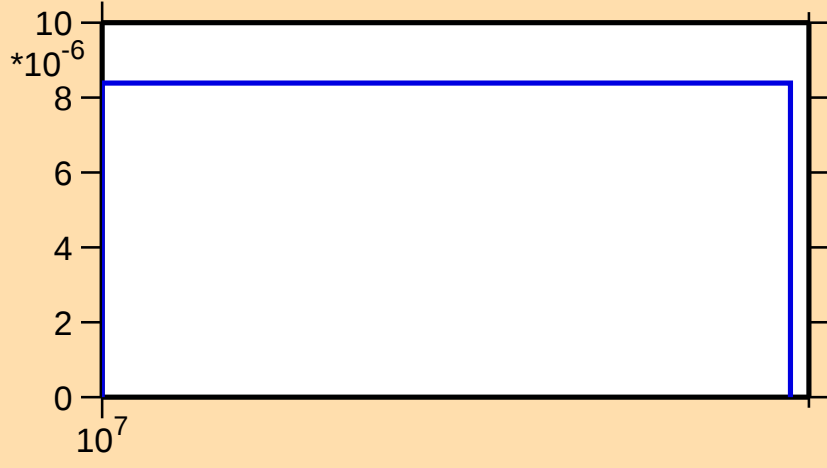
\sigma vs. E for ^{61}\text{Fe}(n,t)
