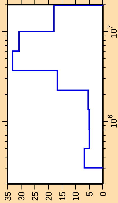
\Delta\sigma/\sigma vs. E for ^{61}\text{Fe}(n,n_2)
