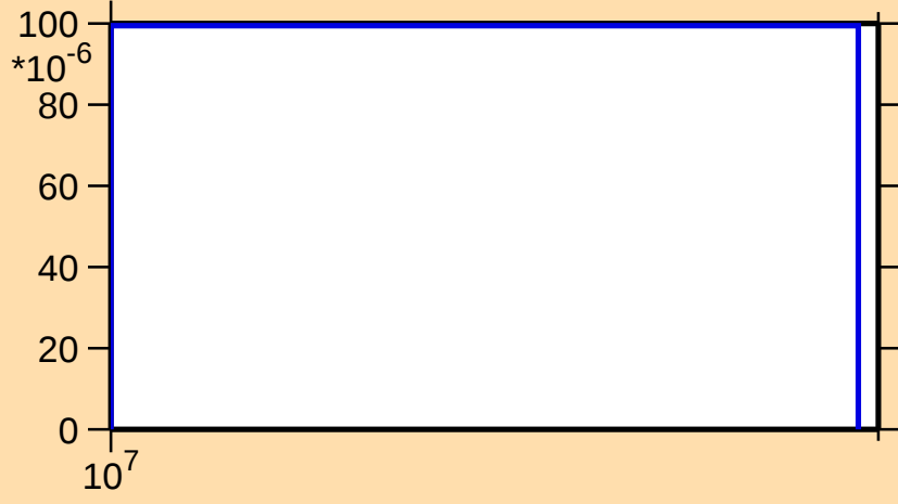
\sigma vs. E for ^{61}\text{Fe}(n,d)
