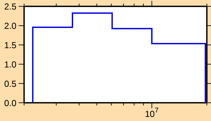
\Delta\sigma/\sigma vs. E for ^{61}\text{Fe}(n,n\text{oncl.})
