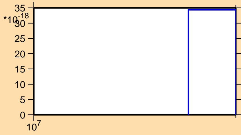
\sigma vs. E for ^{62}\text{Fe}(n,\text{nd})
