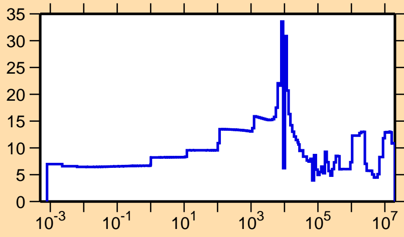
\Delta\sigma/\sigma vs. E for ^{62}\text{Fe}(n,\text{tot.})
