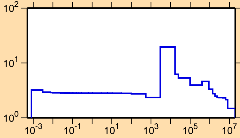
\sigma vs. E for ^{62}\text{Fe}(n,\text{el.})
