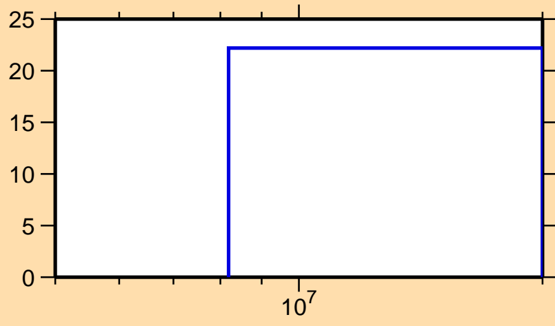
\Delta\sigma/\sigma vs. E for ^{62}\text{Fe}(n,el.)
