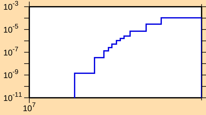
\sigma vs. E for ^{63}\text{Fe}(n,t)
