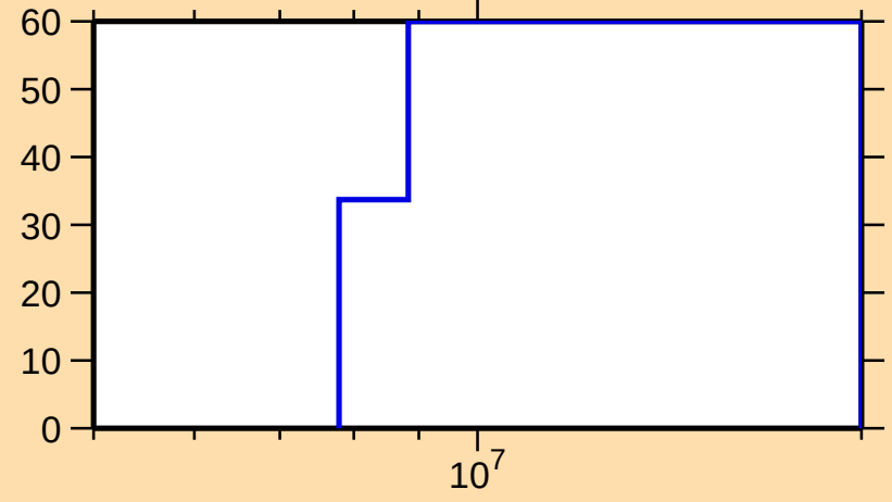
\Delta\sigma/\sigma vs. E for ^{63}\text{Fe}(n,p)
