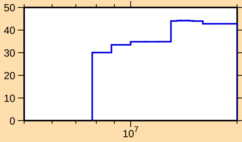
\Delta\sigma/\sigma vs. E for ^{63}\text{Fe}(n,\text{el.})
