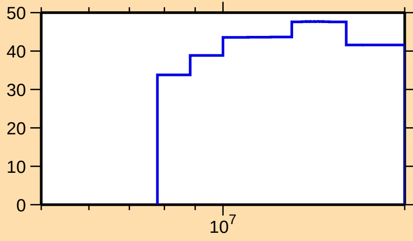
\Delta\sigma/\sigma vs. E for ^{63}\text{Fe}(n,n\text{cont.})
