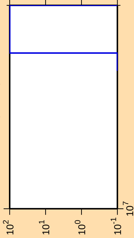
\Delta\sigma/\sigma vs. E for ^{63}\text{Fe}(n,2n\alpha)
