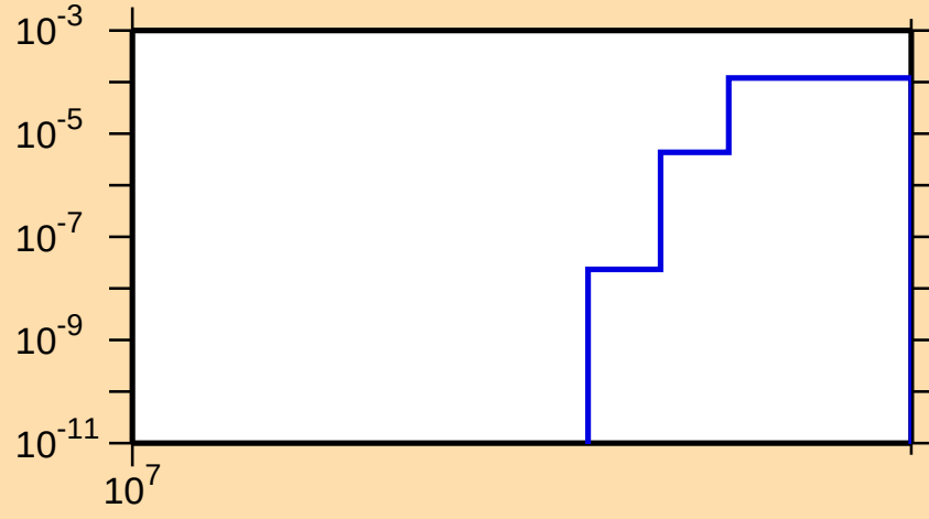
\sigma vs. E for ^{63}\text{Fe}(n,np)
