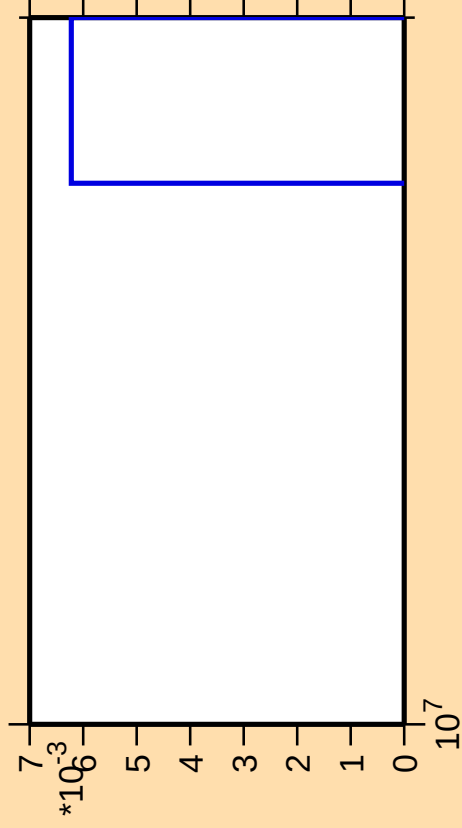
\Delta\sigma/\sigma vs. E for ^{63}\text{Fe}(n,2np)
