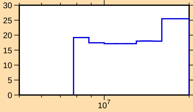
\Delta\sigma/\sigma vs. E for ^{63}\text{Fe}(n,\text{nonel.})
