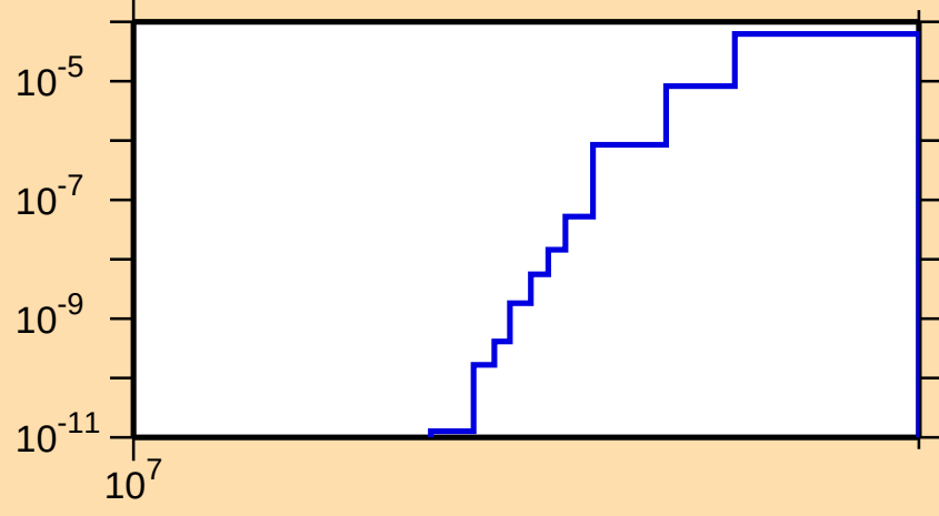
\sigma vs. E for ^{63}\text{Fe}(n,n\alpha)
