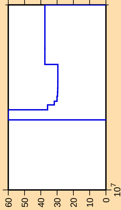
\Delta\sigma/\sigma vs. E for ^{63}\text{Fe}(n,3n)
