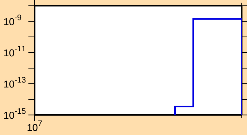
\sigma vs. E for ^{63}\text{Fe}(n,2n\alpha)
