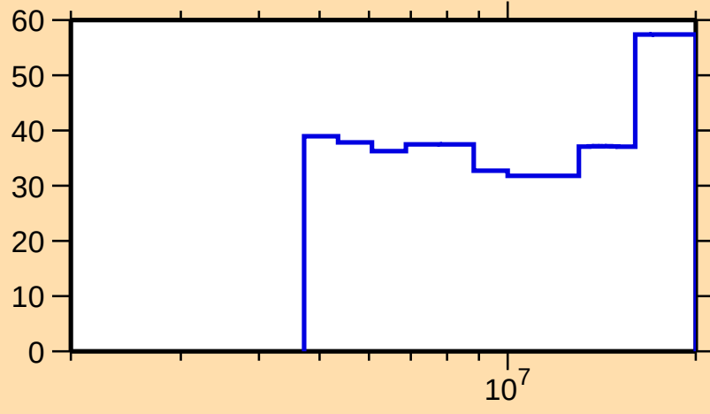
\Delta\sigma/\sigma vs. E for ^{63}\text{Fe}(n,2n)
