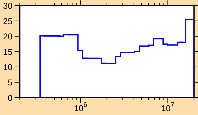
\Delta\sigma/\sigma vs. E for ^{63}\text{Fe}(n,\text{nonel.})
