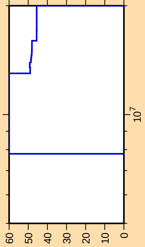
\Delta\sigma/\sigma vs. E for ^{63}\text{Fe}(n,\alpha)
