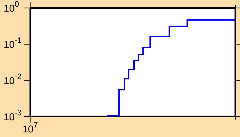
\sigma vs. E for ^{63}\text{Fe}(n,3n)
