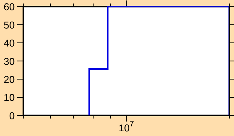
\Delta\sigma/\sigma vs. E for ^{63}\text{Fe}(n,\text{inel.})
