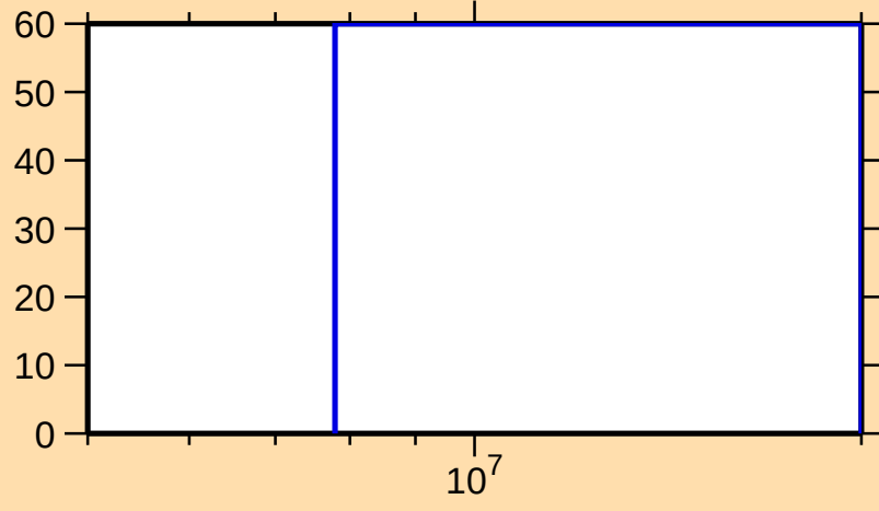
\Delta\sigma/\sigma vs. E for ^{63}\text{Fe}(n,n_1)
