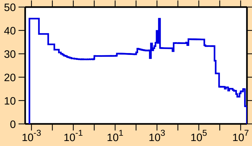
\Delta\sigma/\sigma vs. E for ^{63}\text{Fe}(n,\text{tot.})
