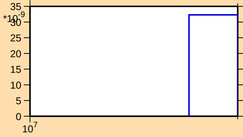
\sigma vs. E for ^{63}\text{Fe}(n,\text{nd})
