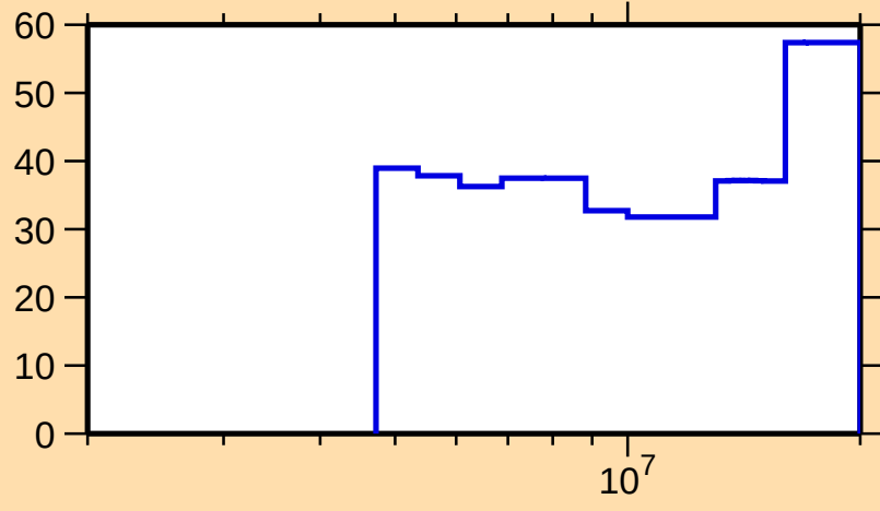
\Delta\sigma/\sigma vs. E for ^{63}\text{Fe}(n,2n)
