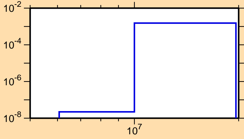
\sigma vs. E for ^{63}\text{Fe}(n,p)
