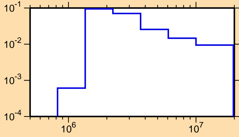
\sigma vs. E for ^{63}\text{Fe}(n,n_4)
