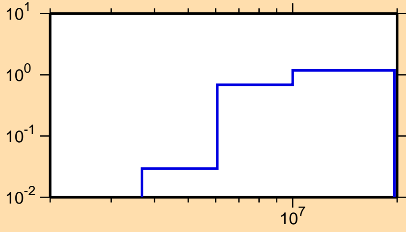
\sigma vs. E for ^{63}\text{Fe}(n,2n)
