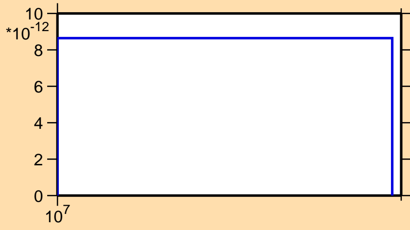
\sigma vs. E for ^{63}\text{Fe}(n,2n\alpha)
