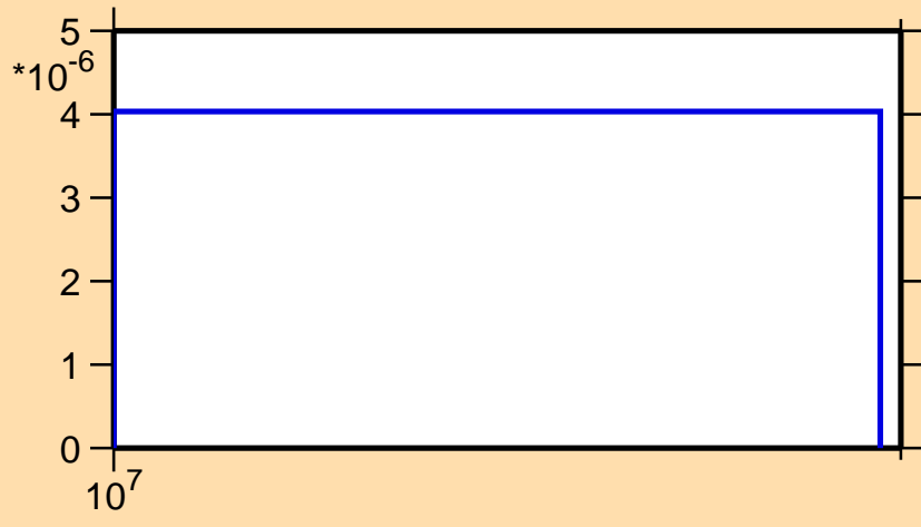
\sigma vs. E for ^{63}\text{Fe}(n,t)
