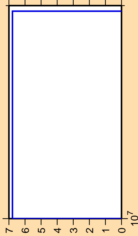
\Delta\sigma/\sigma vs. E for ^{63}\text{Fe}(n,nt)
