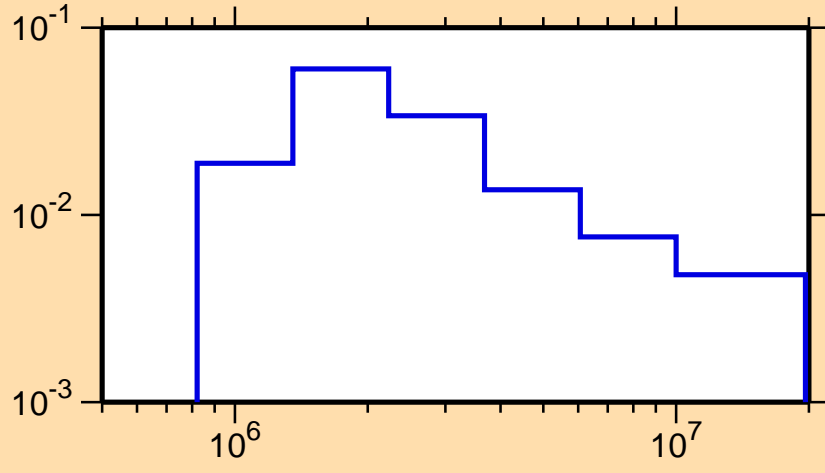
\sigma vs. E for ^{63}\text{Fe}(n,n_2)
