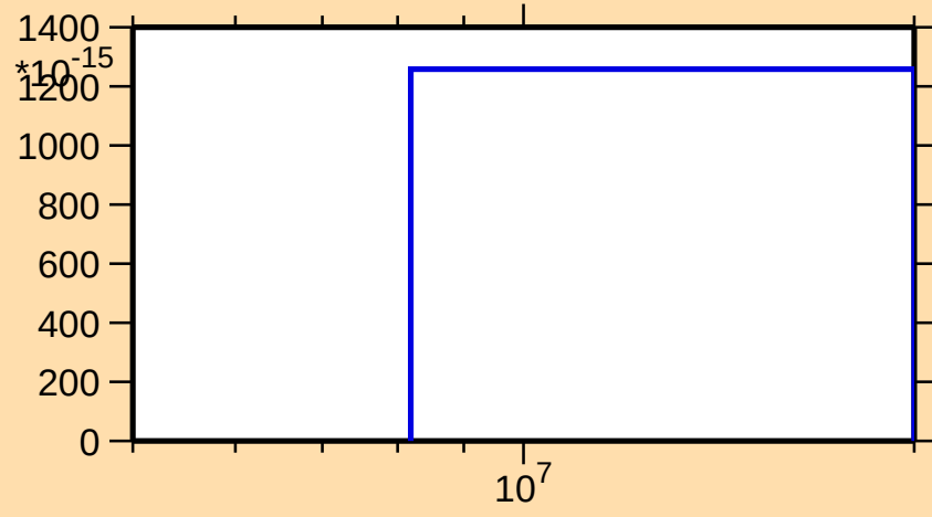
\sigma vs. E for ^{63}\text{Fe}(n,nt)
