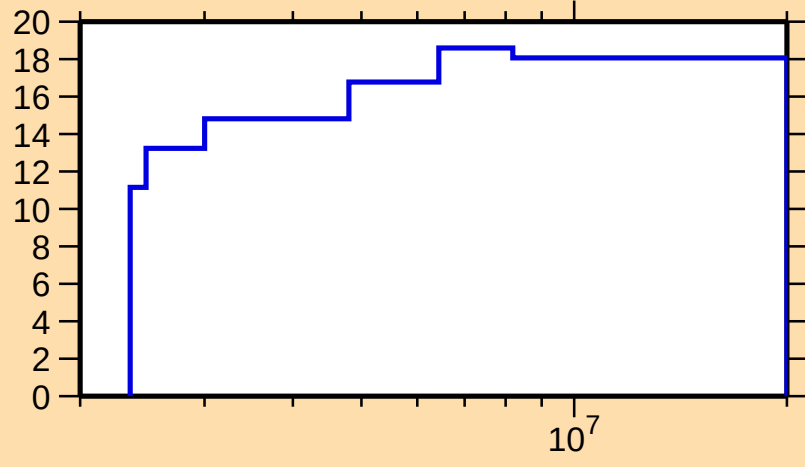
\Delta\sigma/\sigma vs. E for ^{63}\text{Fe}(n,n\text{onel.})
