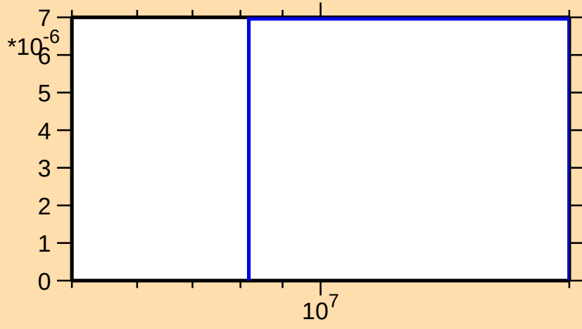
\sigma vs. E for ^{63}\text{Fe}(n,d)
