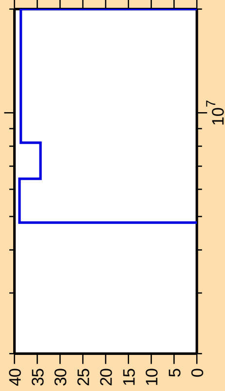
\Delta\sigma/\sigma vs. E for ^{63}\text{Fe}(n,n\text{cont.})
