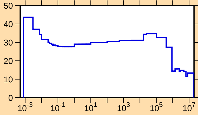
\Delta\sigma/\sigma vs. E for ^{63}\text{Fe}(n,\text{tot.})
