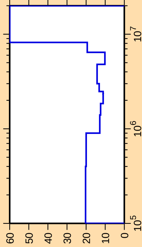
\Delta\sigma/\sigma vs. E for ^{63}\text{Fe}(n,\text{inel.})
