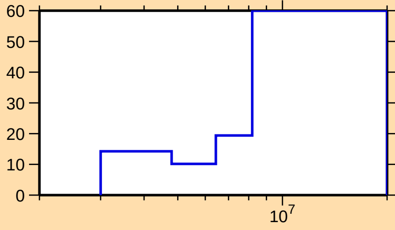
\Delta\sigma/\sigma vs. E for ^{63}\text{Fe}(n,\text{inel.})
