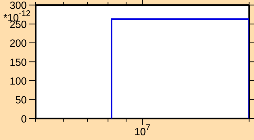
\sigma vs. E for ^{63}\text{Fe}(n,\text{nd})
