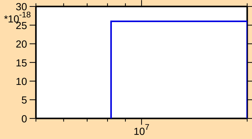
\sigma vs. E for ^{63}\text{Fe}(n,2np)
