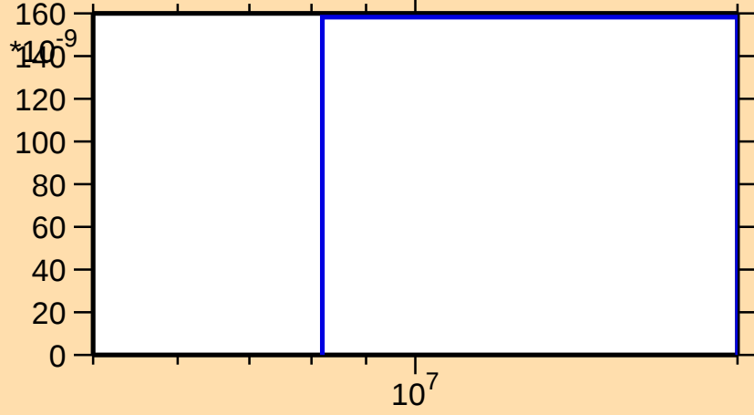
\sigma vs. E for ^{64}\text{Fe}(n,t)
