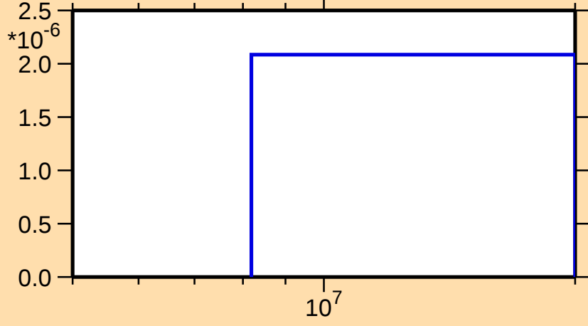
\sigma vs. E for ^{64}\text{Fe}(n,d)
