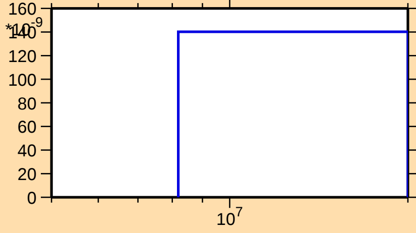
\sigma vs. E for ^{64}\text{Fe}(n,np)
