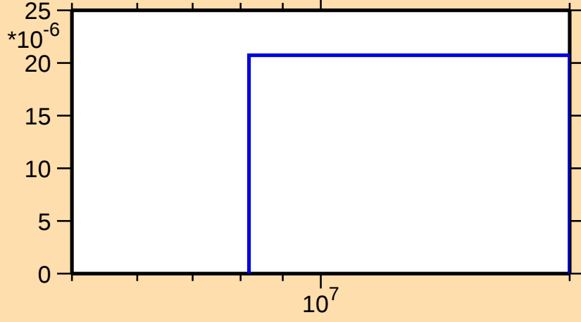
\sigma vs. E for ^{64}\text{Fe}(n,p)
