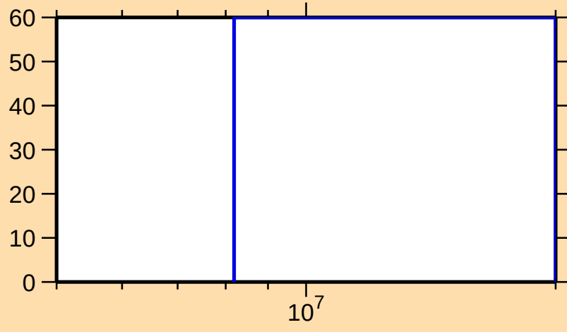
\Delta\sigma/\sigma vs. E for ^{65}\text{Fe}(\text{n,ncont.})
