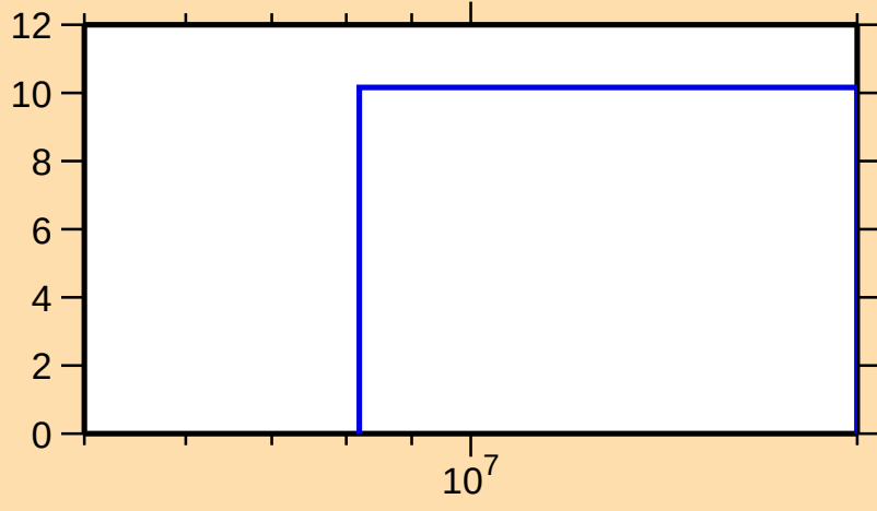
\Delta\sigma/\sigma vs. E for ^{65}\text{Fe}(n,2n)
