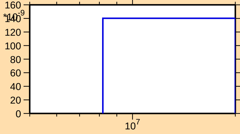
\sigma vs. E for ^{65}\text{Fe}(n,n\alpha)
