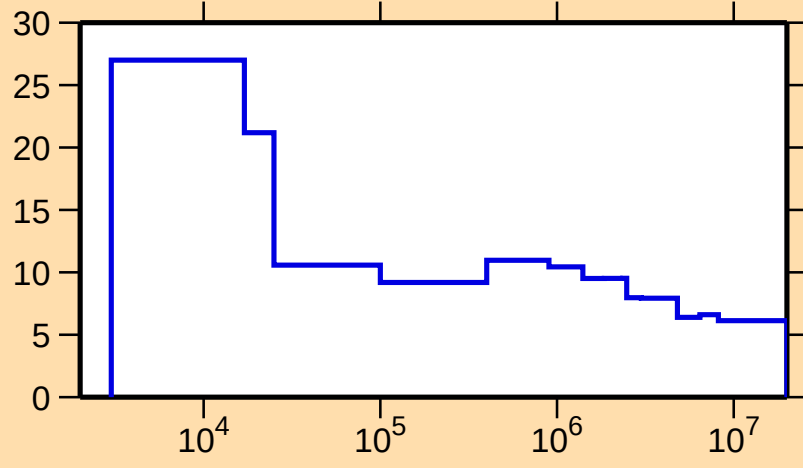
\Delta\sigma/\sigma vs. E for ^{65}\text{Fe}(\text{n,nonel.})
