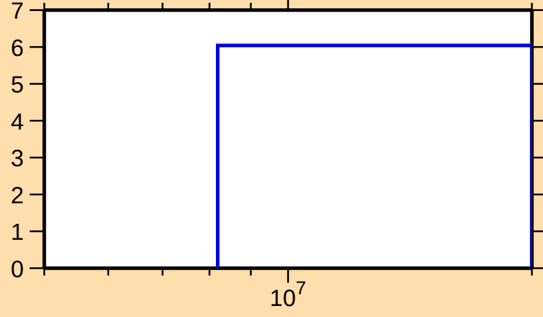
\Delta\sigma/\sigma vs. E for ^{65}\text{Fe}(\text{n,tot.})
