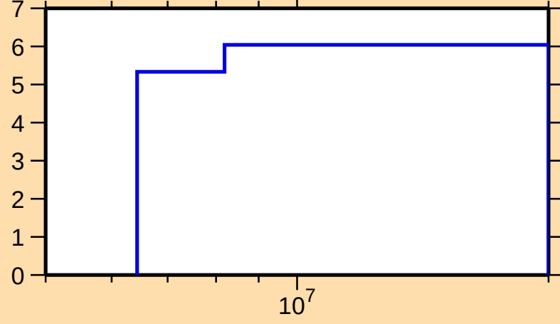
\Delta\sigma/\sigma vs. E for ^{65}\text{Fe}(n,\text{tot.})
