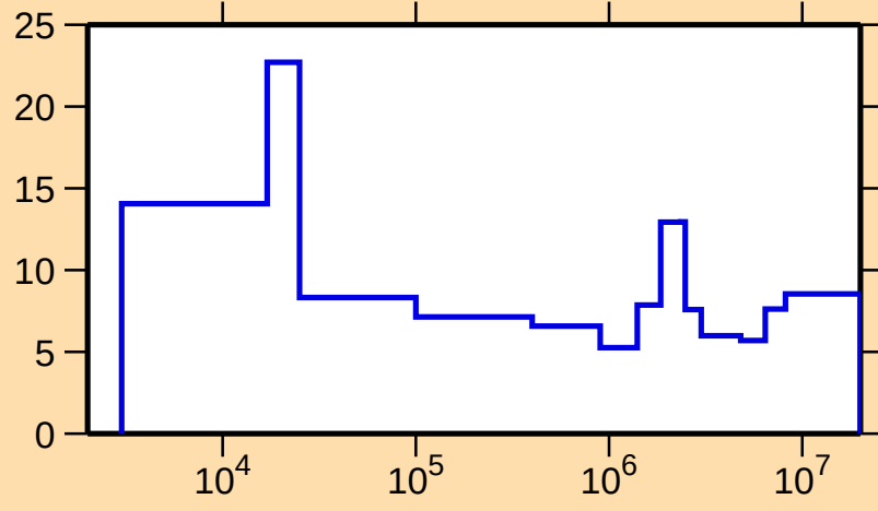
\Delta\sigma/\sigma vs. E for ^{65}\text{Fe}(\text{n,el.})
