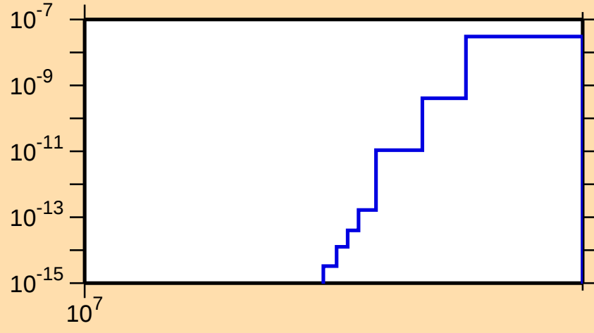
\sigma vs. E for ^{245}\text{Fm}(n,nt)
