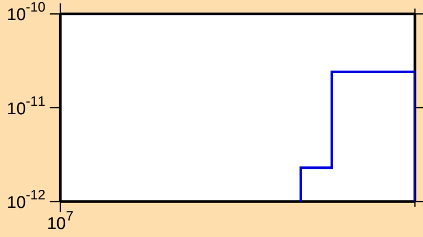
\sigma vs. E for ^{245}\text{Fm}(n,\text{pd})
