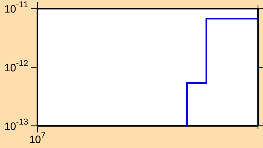
\sigma vs. E for ^{245}\text{Fm}(n,\text{pt})
