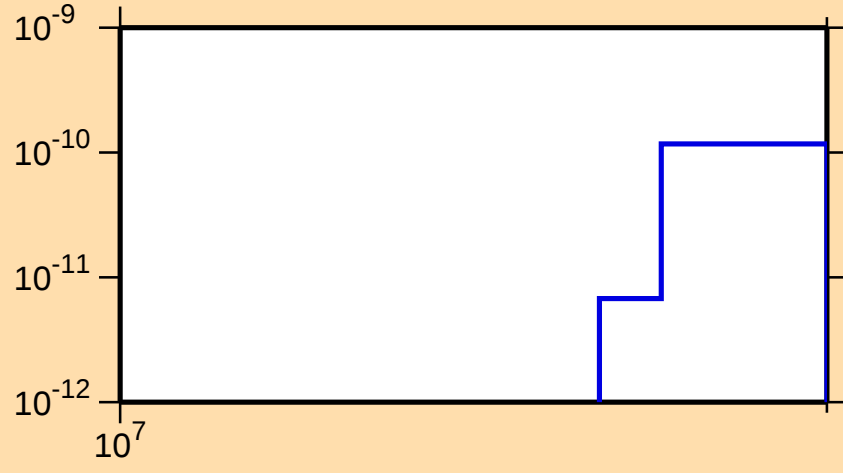
\sigma vs. E for ^{245}\text{Fm}(\text{mt } 34)
