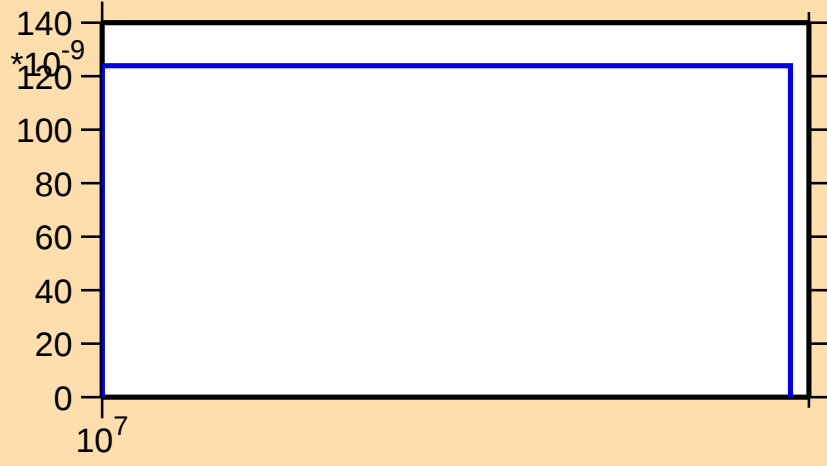
\sigma vs. E for ^{245}\text{Fm}(n,2np)
