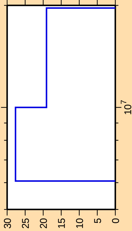
\Delta\sigma/\sigma vs. E for ^{245}\text{Fm}(n,f)
