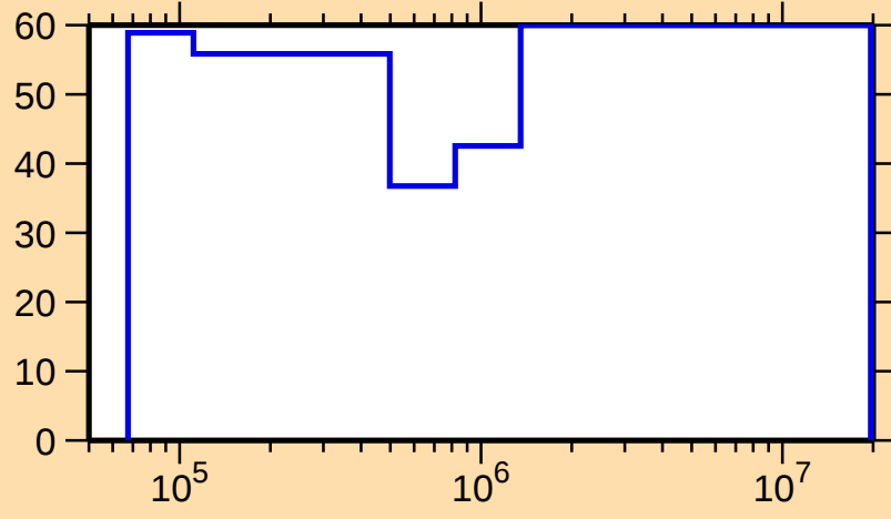
\Delta\sigma/\sigma vs. E for ^{245}\text{Fm}(n,n_1)
