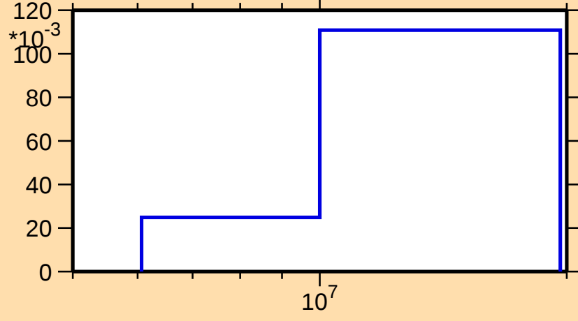
\sigma vs. E for ^{245}\text{Fm}(n,2n)
