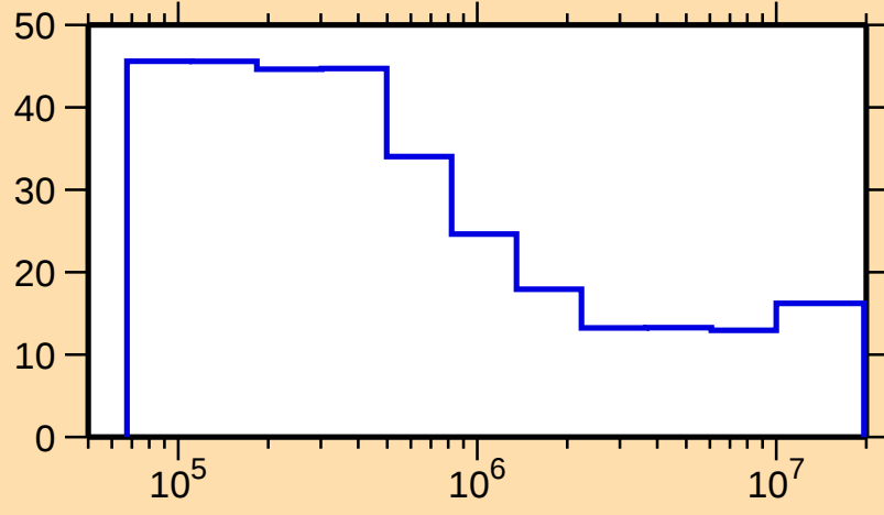
\Delta\sigma/\sigma vs. E for ^{245}\text{Fm}(n,n\text{onel.})
