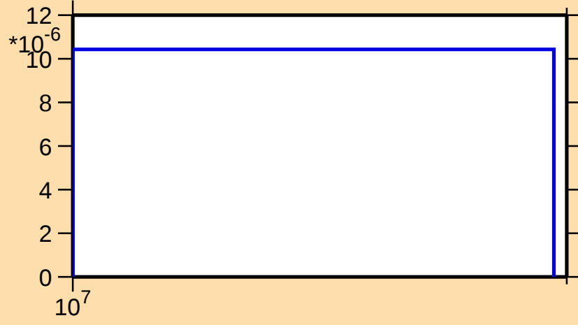
\sigma vs. E for ^{245}\text{Fm}(n,3n)
