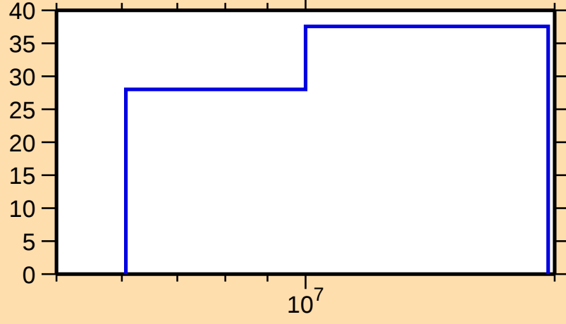
\Delta\sigma/\sigma vs. E for ^{245}\text{Fm}(n,\text{tot.})
