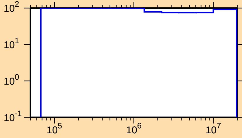
\Delta\sigma/\sigma vs. E for ^{245}\text{Fm}(n,n\text{cont.})
