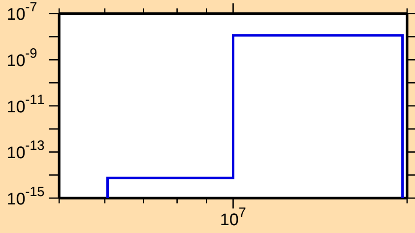
\sigma vs. E for ^{245}\text{Fm}(n,\text{He3})
