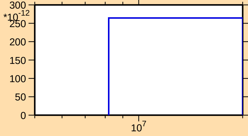
\sigma vs. E for ^{245}\text{Fm}(n,nt)
