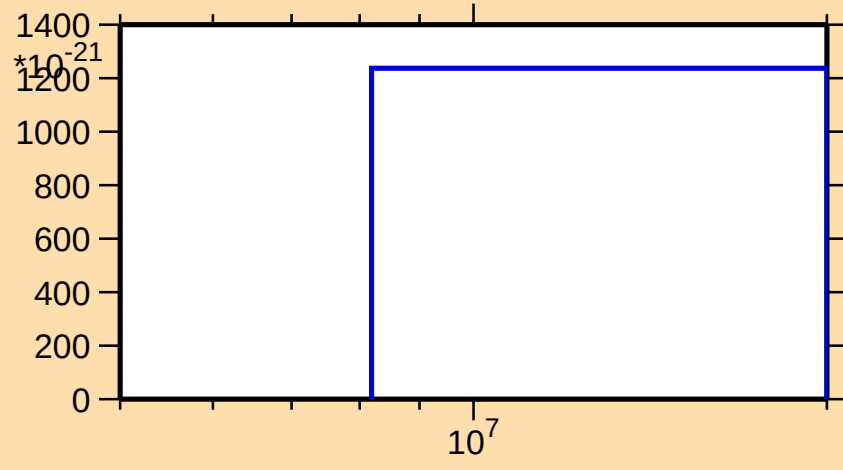
\sigma vs. E for ^{245}\text{Fm}(\text{mt } 42)
