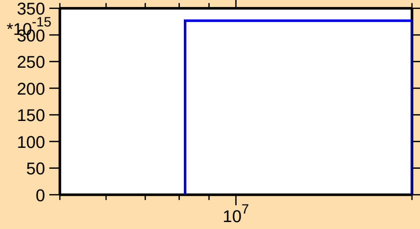
\sigma vs. E for ^{245}\text{Fm}(n,\text{pd})
