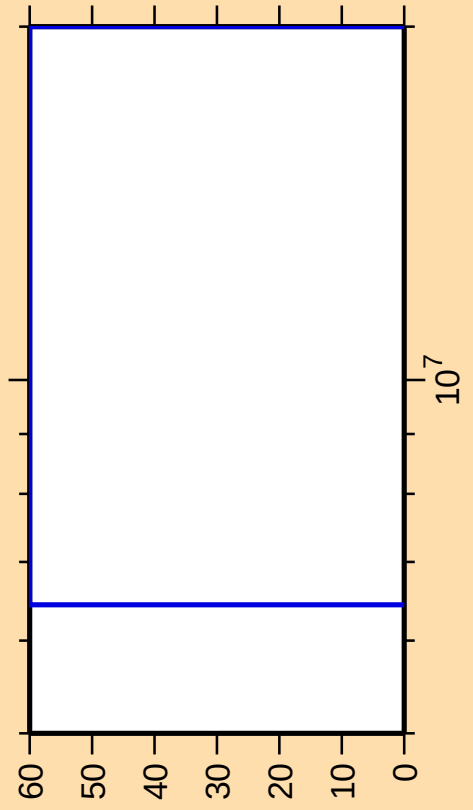
\Delta\sigma/\sigma vs. E for ^{245}\text{Fm}(n,2n)
