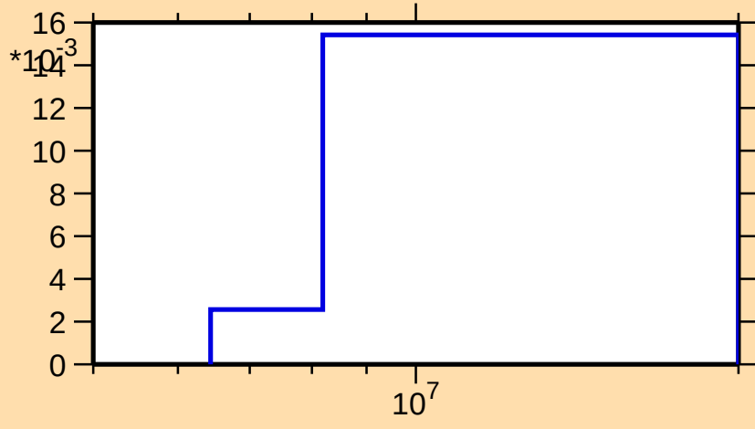
\sigma vs. E for ^{245}\text{Fm}(n,2n\alpha)
