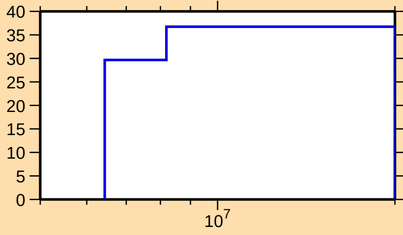
\Delta\sigma/\sigma vs. E for ^{245}\text{Fm}(n,\text{tot.})
