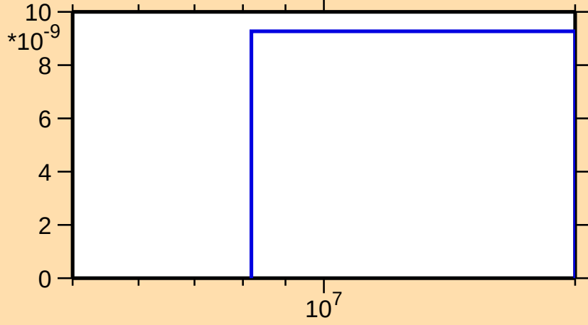
\sigma vs. E for ^{245}\text{Fm}(n,\text{He}3)
