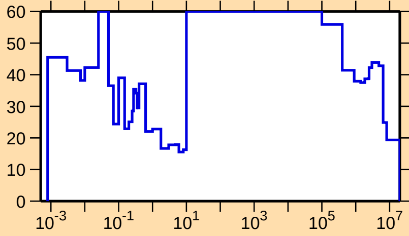
\Delta\sigma/\sigma vs. E for ^{245}\text{Fm}(n,f)
