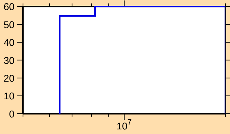
\Delta\sigma/\sigma vs. E for ^{245}\text{Fm}(n,\text{inel.})
