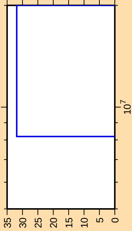
\Delta\sigma/\sigma vs. E for ^{245}\text{Fm}(\text{mt } 45)
