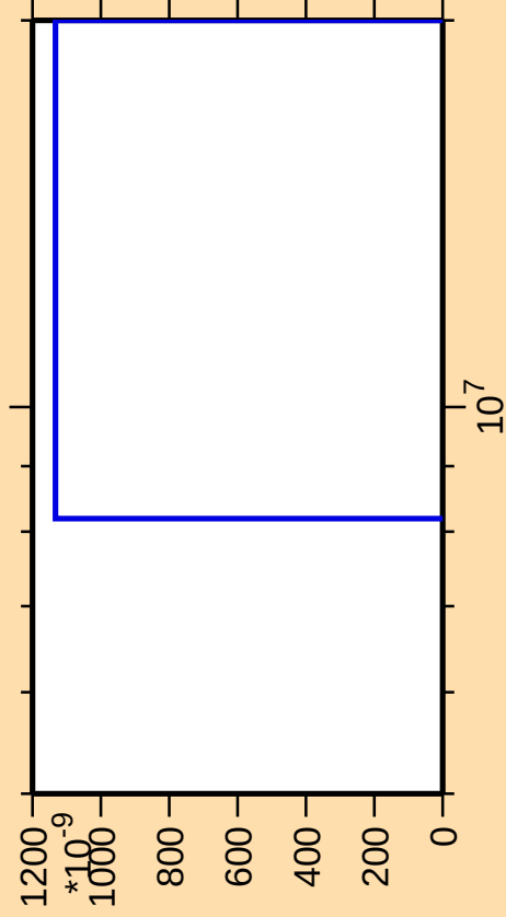
\Delta\sigma/\sigma vs. E for ^{245}\text{Fm}(\text{mt } 42)
