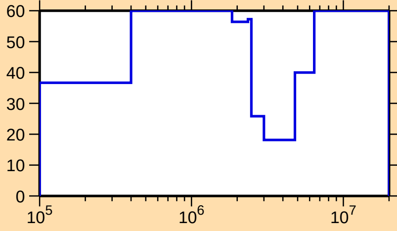
\Delta\sigma/\sigma vs. E for ^{245}\text{Fm}(n,\text{el.})
