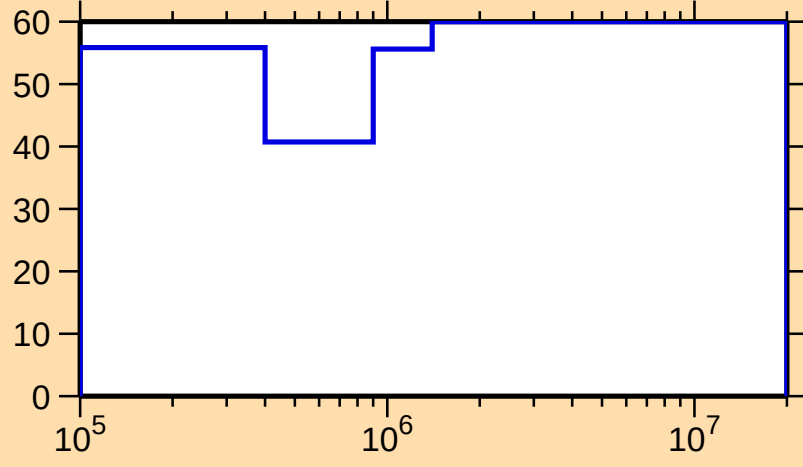
\Delta\sigma/\sigma vs. E for ^{245}\text{Fm}(n,n_1)
