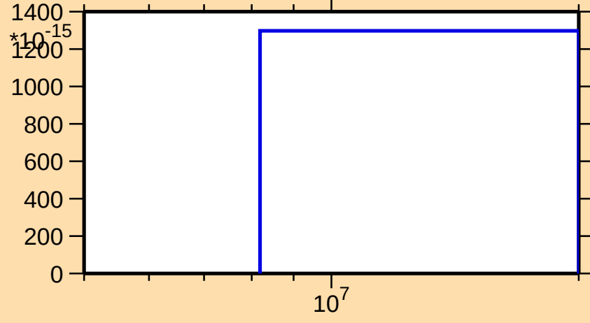
\sigma vs. E for ^{245}\text{Fm}(\text{mt } 34)
