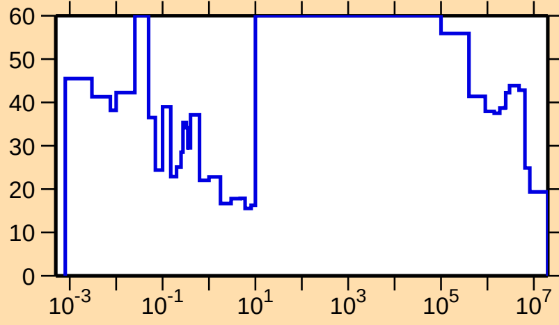
\Delta\sigma/\sigma vs. E for ^{245}\text{Fm}(n,f)
