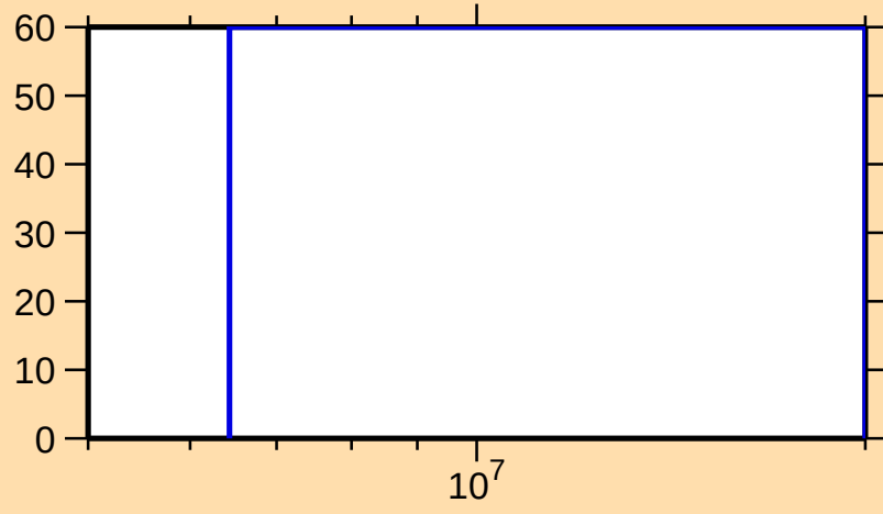
\Delta\sigma/\sigma vs. E for ^{245}\text{Fm}(n,2n)
