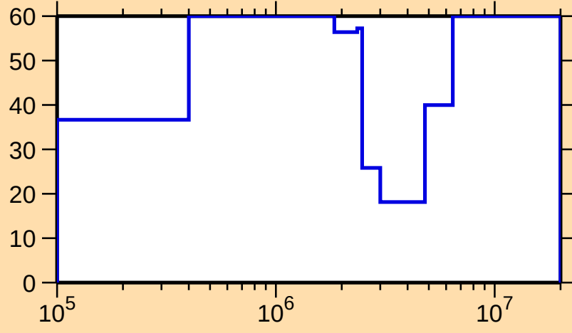
\Delta\sigma/\sigma vs. E for ^{245}\text{Fm}(n,\text{el.})
