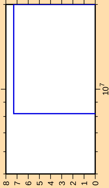
\Delta\sigma/\sigma vs. E for ^{245}\text{Fm}(\text{mt } 34)
