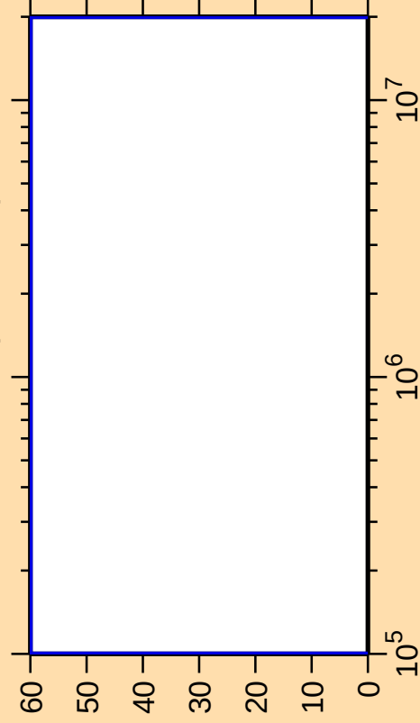
\Delta\sigma/\sigma vs. E for ^{245}\text{Fm}(n,n_{\text{cont}})
