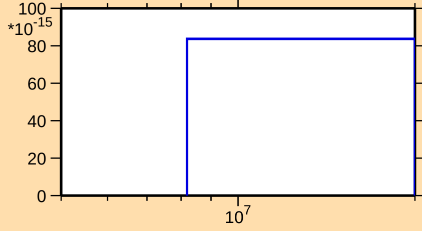
\sigma vs. E for ^{245}\text{Fm}(n,\text{pt})
