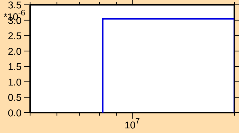
\sigma vs. E for ^{245}\text{Fm}(n,3n\alpha)
