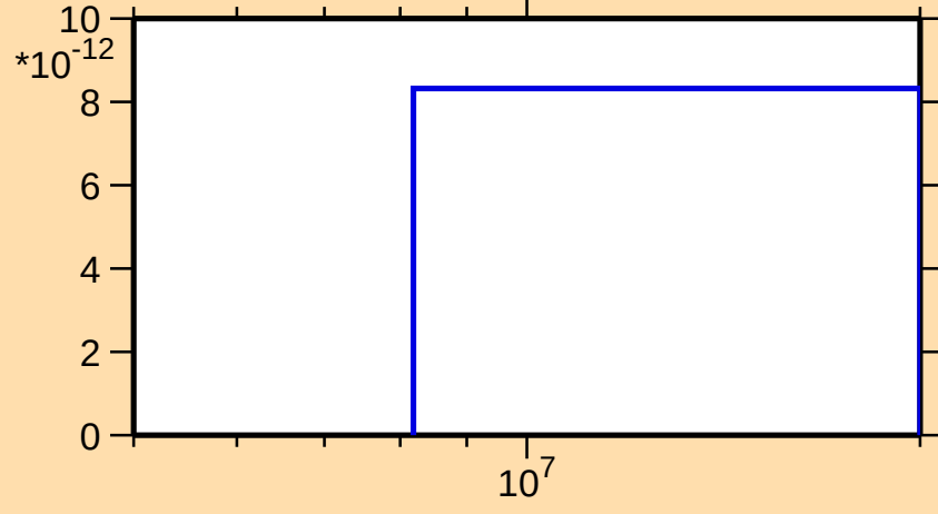
\sigma vs. E for ^{245}\text{Fm}(\text{mt } 45)
