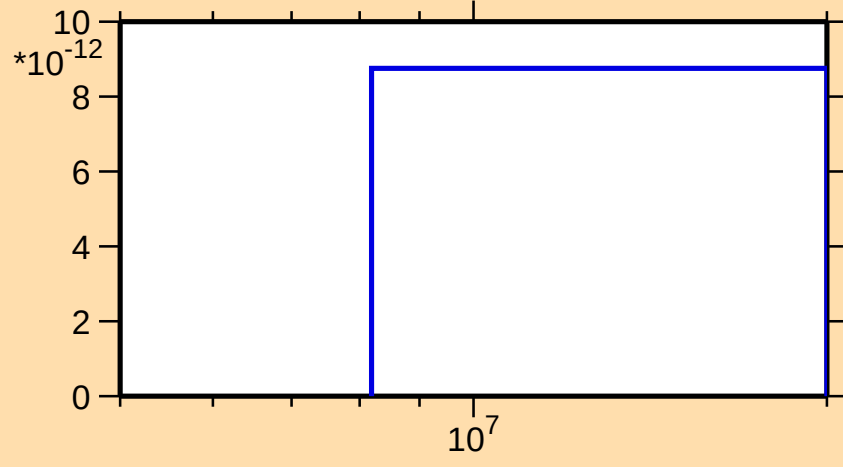
\sigma vs. E for ^{245}\text{Fm}(\text{mt117})
