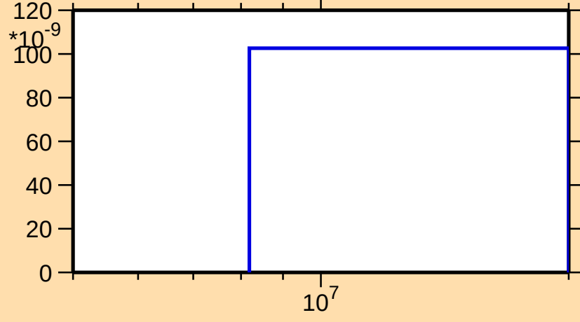
\sigma vs. E for ^{245}\text{Fm}(n,2np)
