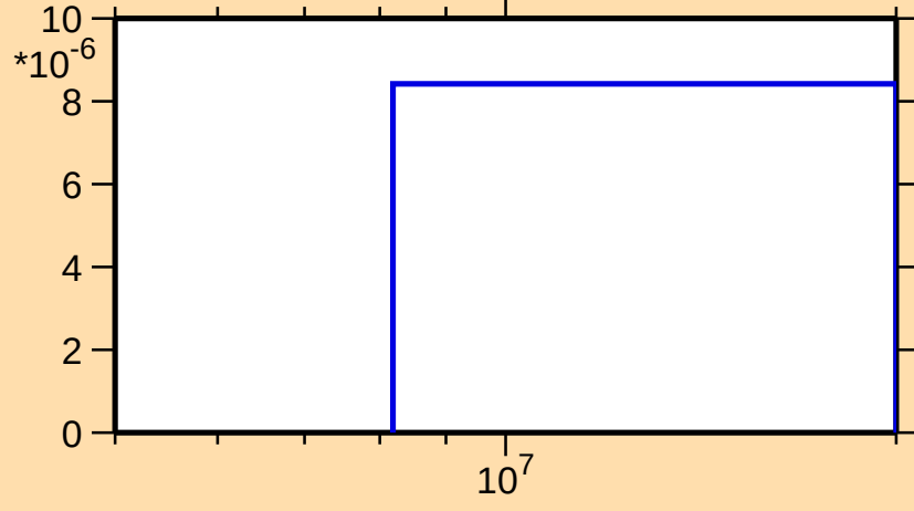
\sigma vs. E for ^{245}\text{Fm}(n,3n)
