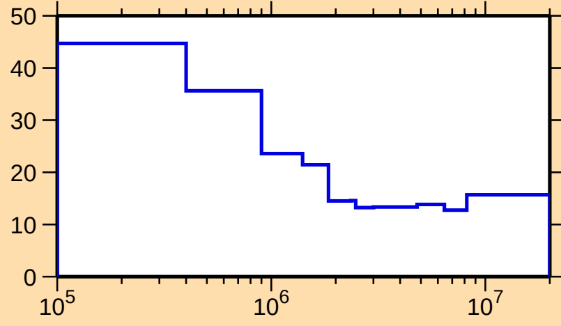
\Delta\sigma/\sigma vs. E for ^{245}\text{Fm}(n,\text{nonel.})
