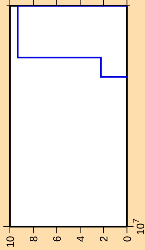
\Delta\sigma/\sigma vs. E for ^{248}\text{Fm}(\text{mt } 45)
