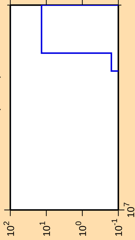
\Delta\sigma/\sigma vs. E for ^{248}\text{Fm}(\text{mt } 34)
