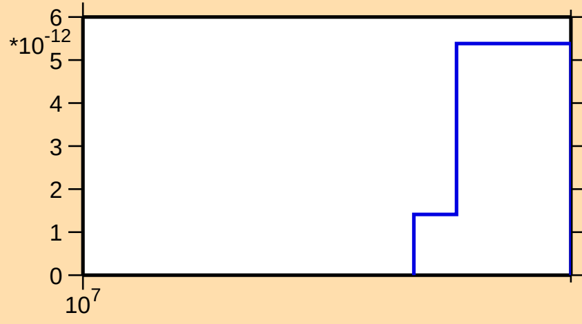
\sigma vs. E for ^{248}\text{Fm}(\text{mt117})
