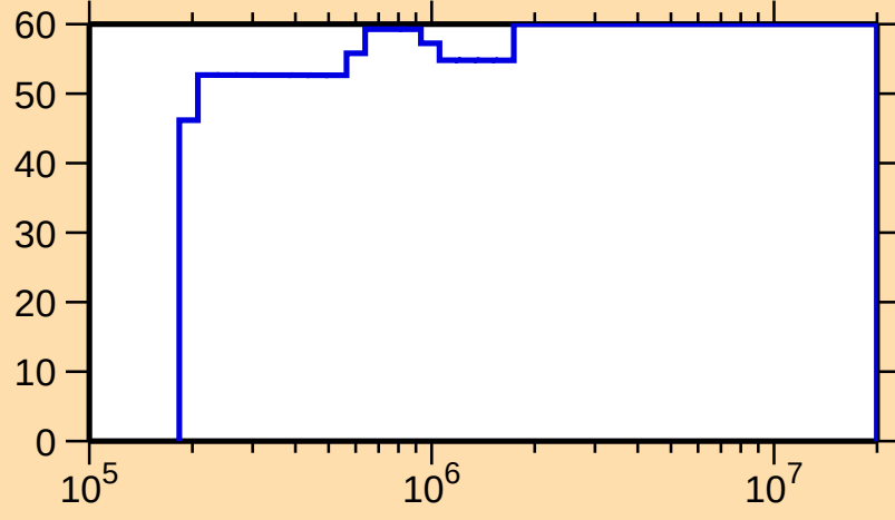
\Delta\sigma/\sigma vs. E for ^{248}\text{Fm}(n,\gamma)
