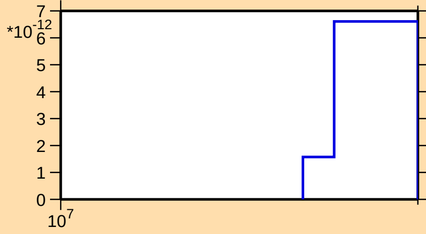
\sigma vs. E for ^{248}\text{Fm}(\text{mt } 45)
