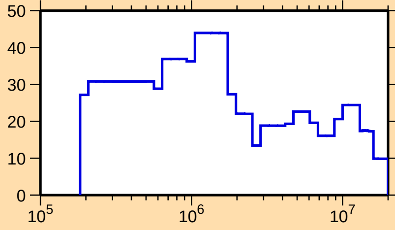
\Delta\sigma/\sigma vs. E for ^{248}\text{Fm}(n,\text{el.})
