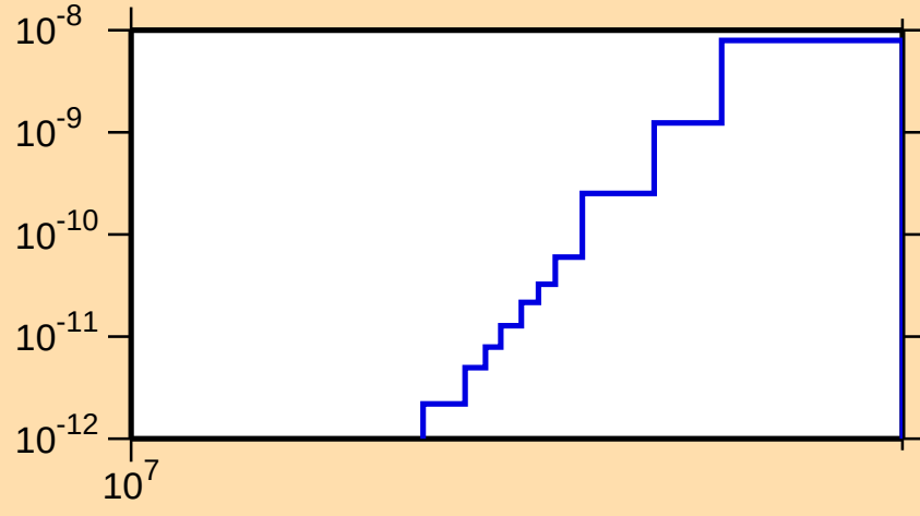
\sigma vs. E for ^{248}\text{Fm}(n,\text{He3})
