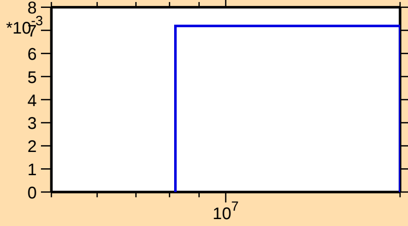
\sigma vs. E for ^{248}\text{Fm}(n,3n)
