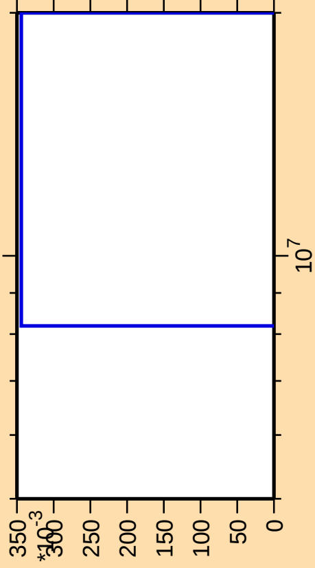
\Delta\sigma/\sigma vs. E for ^{248}\text{Fm}(\text{mt117})
