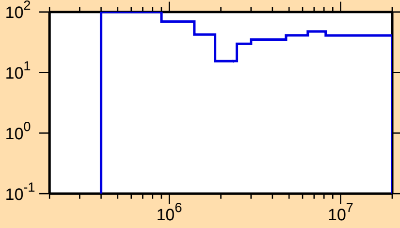
\Delta\sigma/\sigma vs. E for ^{248}\text{Fm}(n,n\text{cont.})
