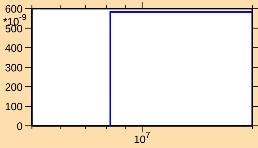
\sigma vs. E for ^{248}\text{Fm}(n,3n\alpha)
