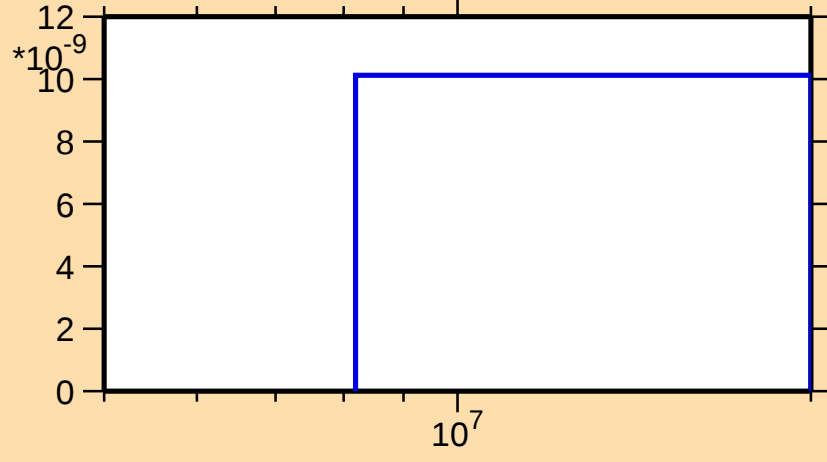
\sigma vs. E for ^{248}\text{Fm}(n,nd)
