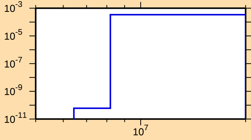
\sigma vs. E for ^{248}\text{Fm}(n,d)
