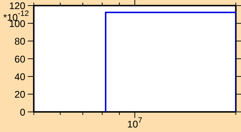
\sigma vs. E for ^{248}\text{Fm}(n,p\alpha)
