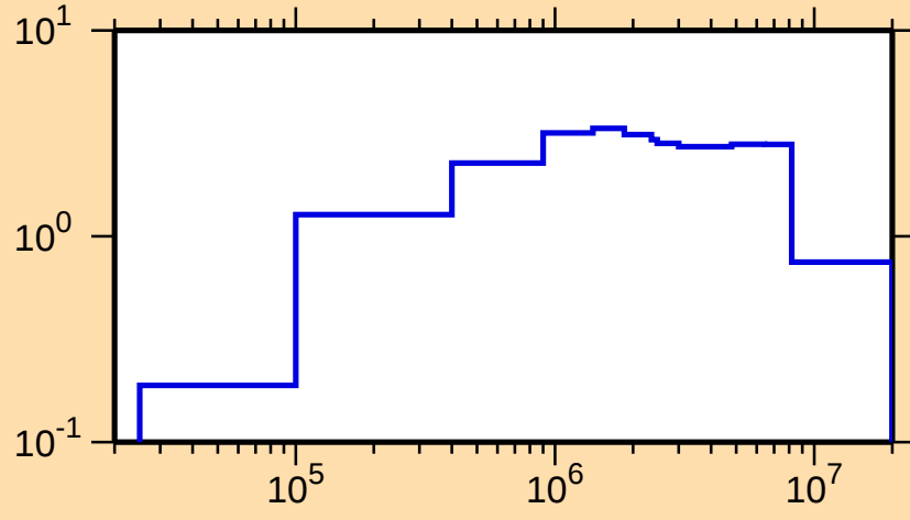
\sigma vs. E for ^{248}\text{Fm}(n,\text{inel.})
