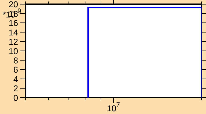
\sigma vs. E for ^{248}\text{Fm}(n,2np)
