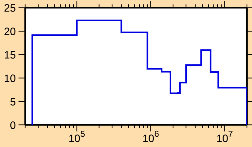
\Delta\sigma/\sigma vs. E for ^{248}\text{Fm}(n,\text{tot.})
