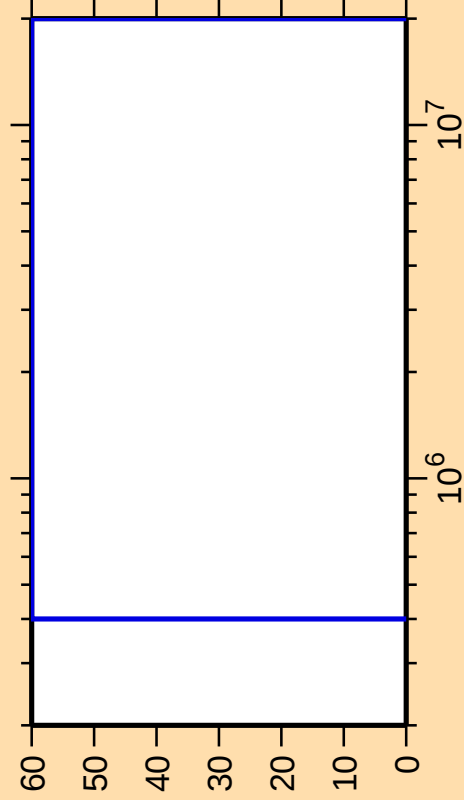
\Delta\sigma/\sigma vs. E for ^{248}\text{Fm}(n,p)
