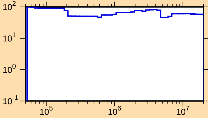
\Delta\sigma/\sigma vs. E for ^{249}\text{Fm}(n,n_1)
