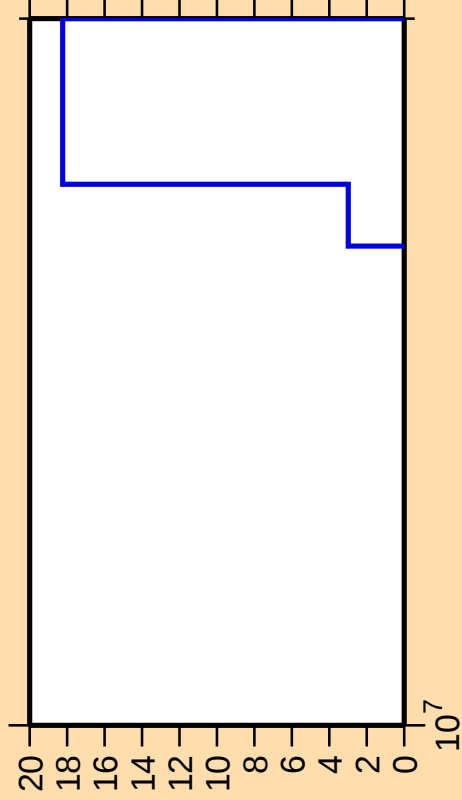
\Delta\sigma/\sigma vs. E for ^{249}\text{Fm}(\text{mt } 45)
