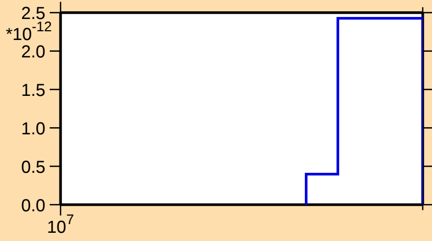
\sigma vs. E for ^{249}\text{Fm}(\text{mt } 45)
