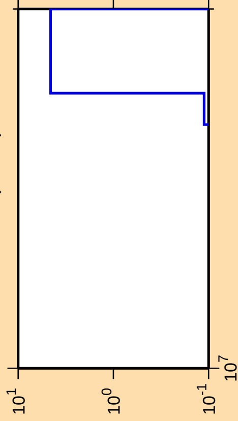
\Delta\sigma/\sigma vs. E for ^{249}\text{Fm}(\text{mt } 34)
