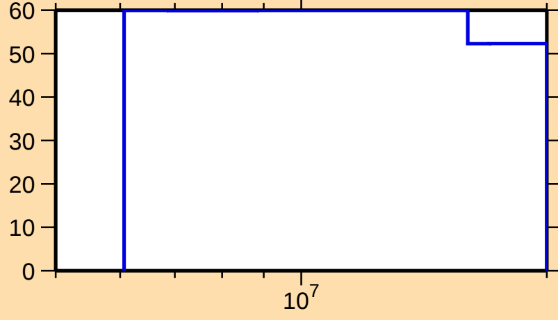
\Delta\sigma/\sigma vs. E for ^{249}\text{Fm}(n,2n)
