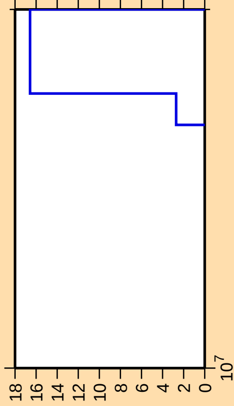
\Delta\sigma/\sigma vs. E for ^{249}\text{Fm}(\text{mt117})
