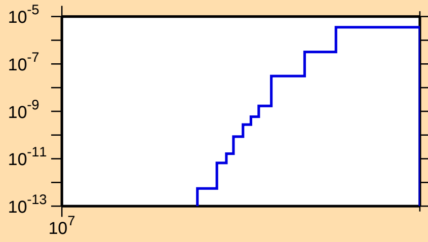
\sigma vs. E for ^{249}\text{Fm}(n,2np)
