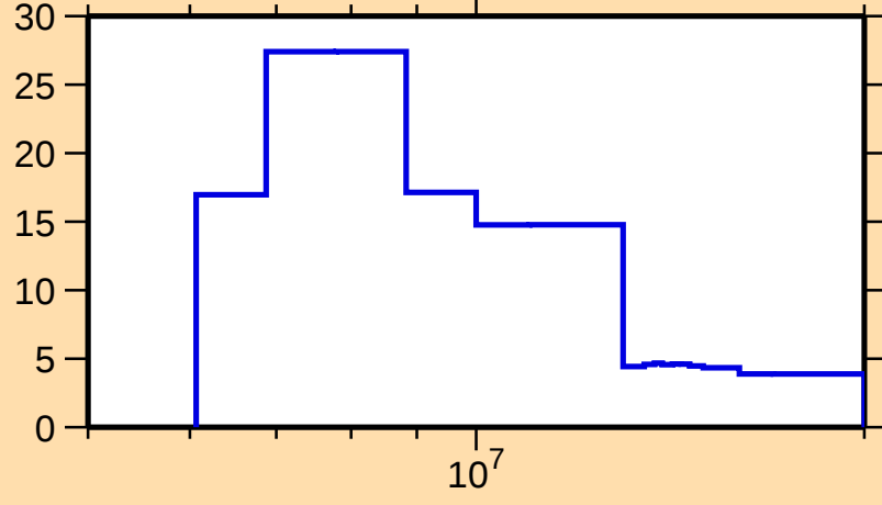
\Delta\sigma/\sigma vs. E for ^{249}\text{Fm}(n,\text{el.})
