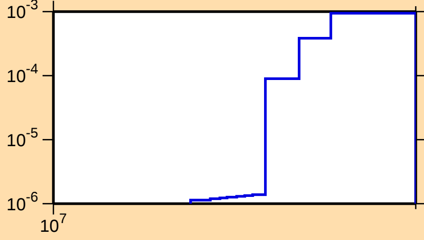
\sigma vs. E for ^{249}\text{Fm}(n,3n\alpha)
