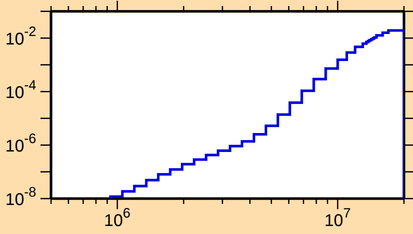
\sigma vs. E for ^{249}\text{Fm}(n,p)
