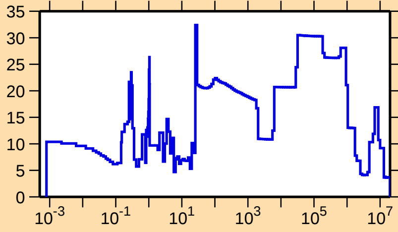
\Delta\sigma/\sigma vs. E for ^{249}\text{Fm}(n,\text{tot.})
