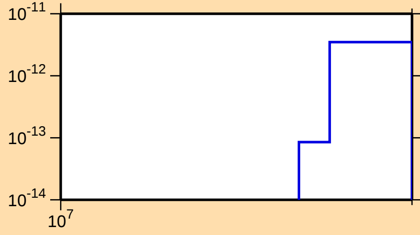
\sigma vs. E for ^{249}\text{Fm}(\text{mt } 34)
