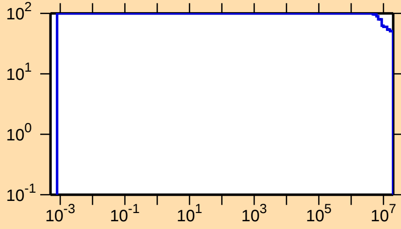
\Delta\sigma/\sigma vs. E for ^{249}\text{Fm}(n,p)
