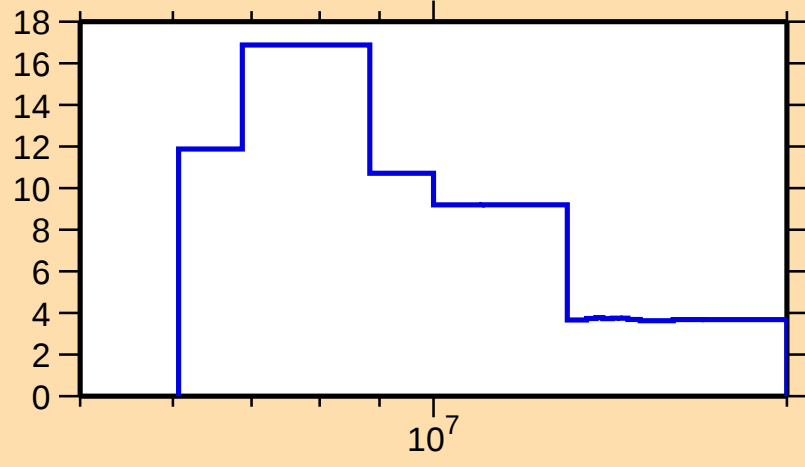
\Delta\sigma/\sigma vs. E for ^{249}\text{Fm}(n,\text{tot.})
