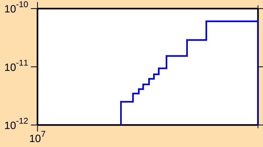
\sigma vs. E for ^{249}\text{Fm}(n,p\alpha)
