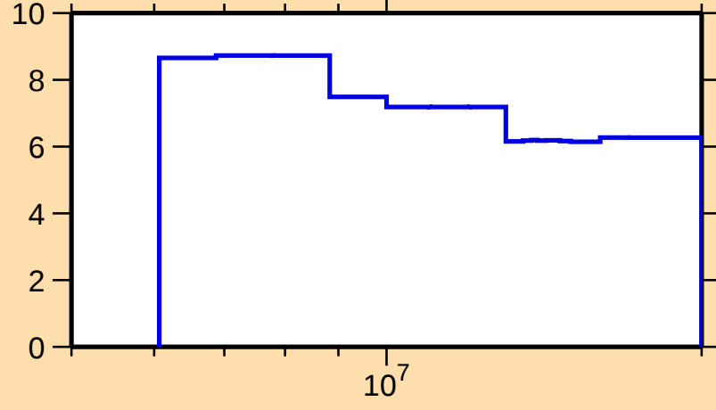
\Delta\sigma/\sigma vs. E for ^{249}\text{Fm}(n,\text{nonel.})
