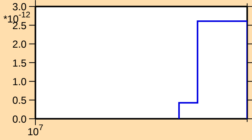
\sigma vs. E for ^{249}\text{Fm}(\text{mt117})
