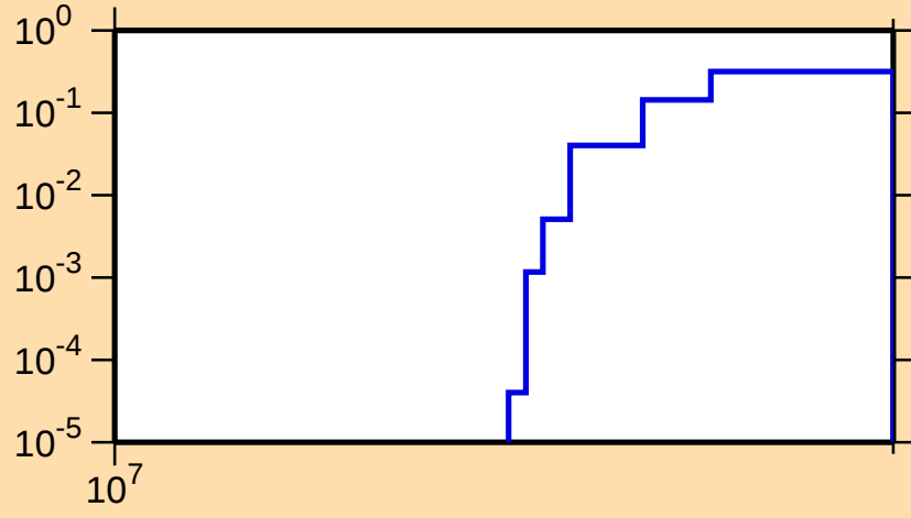
\sigma vs. E for ^{249}\text{Fm}(n,3n)
