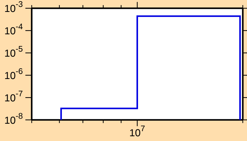
\sigma vs. E for ^{249}\text{Fm}(n,np)
