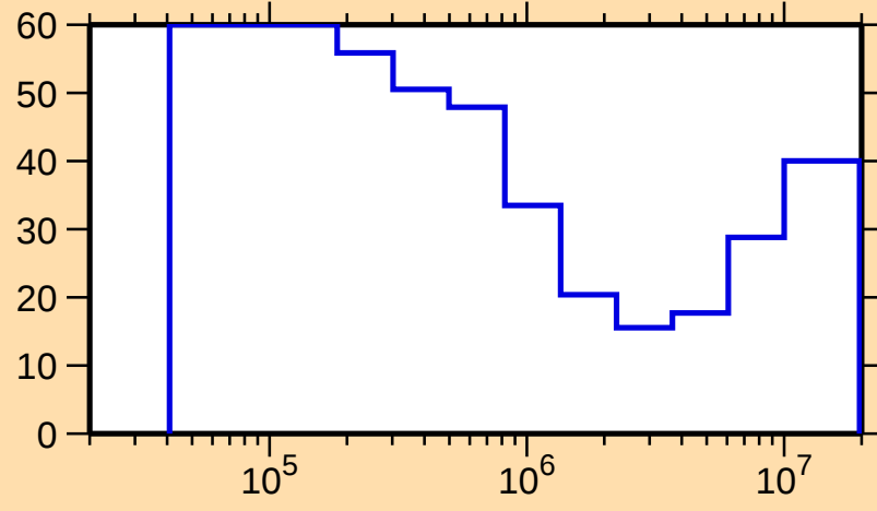
\Delta\sigma/\sigma vs. E for ^{249}\text{Fm}(n,\text{inel.})
