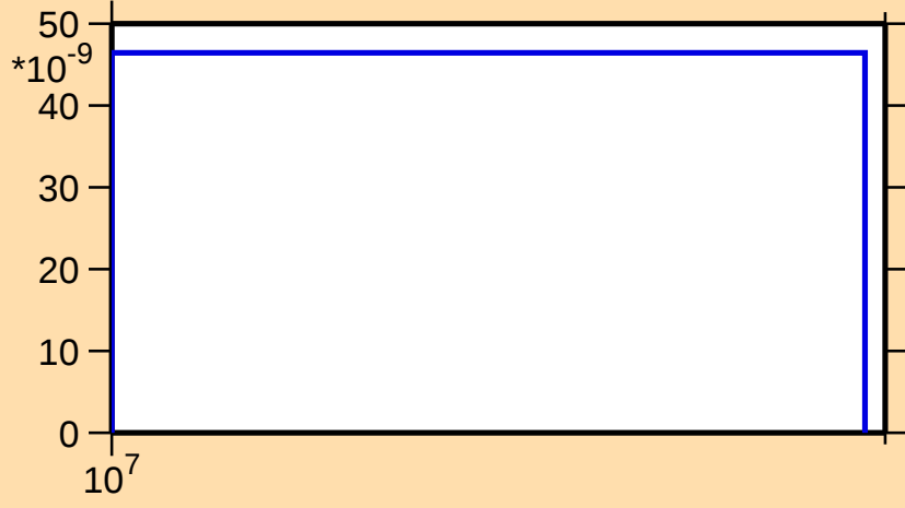
\sigma vs. E for ^{249}\text{Fm}(n,\text{nd})
