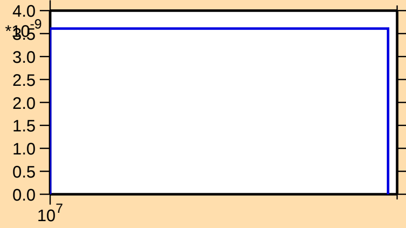
\sigma vs. E for ^{249}\text{Fm}(n,nt)
