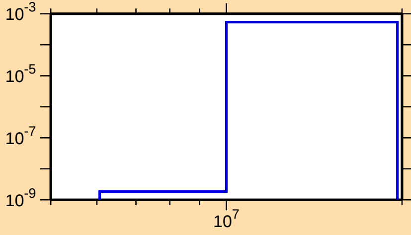
\sigma vs. E for ^{249}\text{Fm}(n,2n\alpha)
