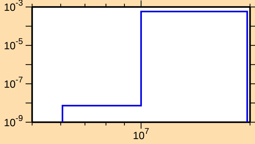
\sigma vs. E for ^{249}\text{Fm}(n,d)
