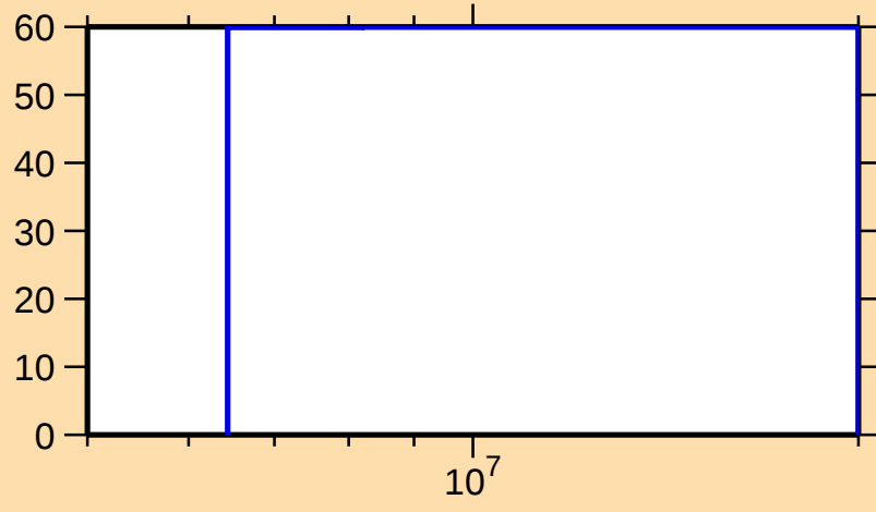
\Delta\sigma/\sigma vs. E for ^{249}\text{Fm}(n,2n)
