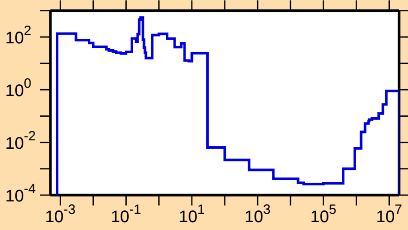
\sigma vs. E for ^{249}\text{Fm}(n,f)
