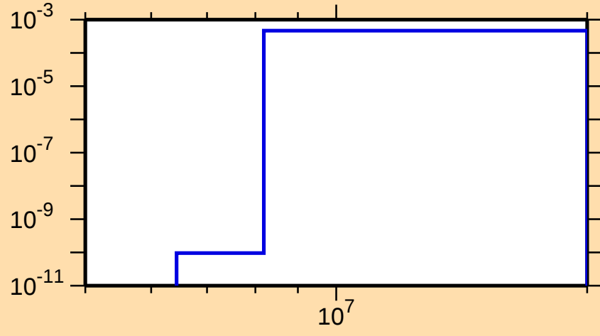
\sigma vs. E for ^{249}\text{Fm}(n,d)
