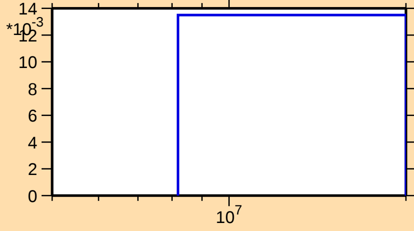
\sigma vs. E for ^{249}\text{Fm}(n,3n)
