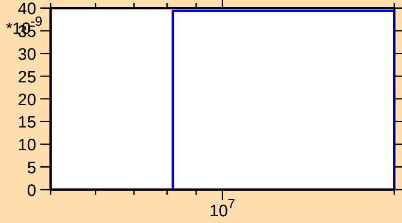
\sigma vs. E for ^{249}\text{Fm}(n,\text{nd})
