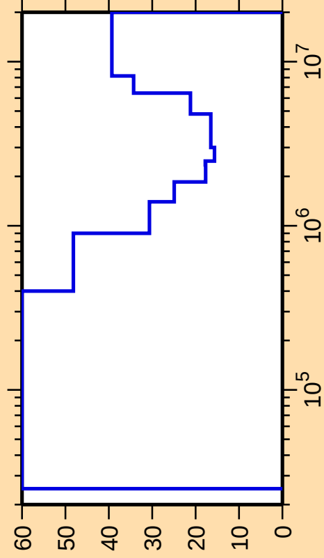
\Delta\sigma/\sigma vs. E for ^{249}\text{Fm}(n,\text{inel.})
