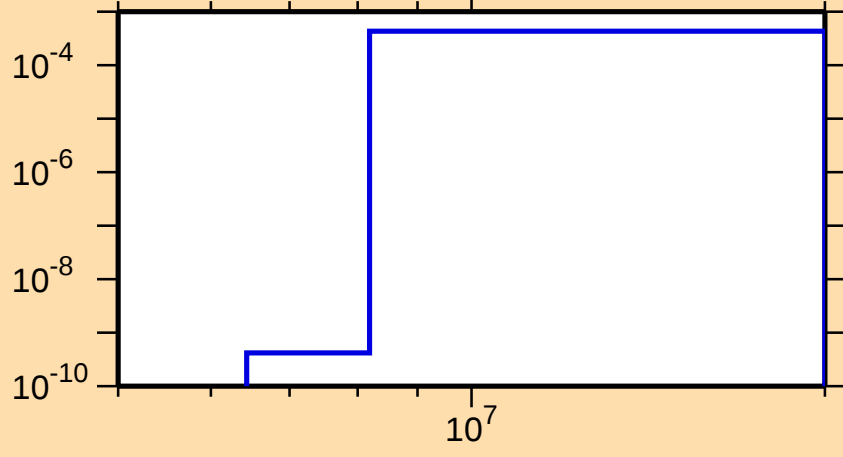
\sigma vs. E for ^{249}\text{Fm}(n,2n\alpha)
