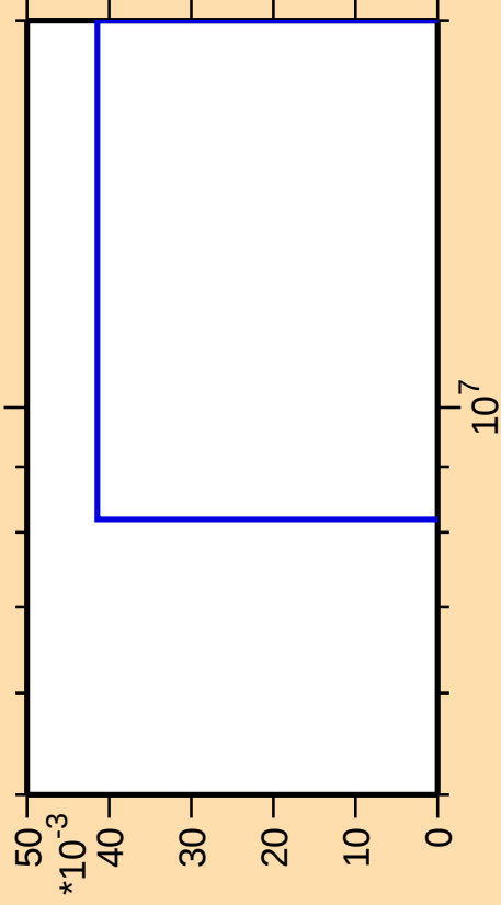
\Delta\sigma/\sigma vs. E for ^{249}\text{Fm}(\text{mt } 34)
