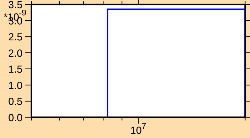
\sigma vs. E for ^{249}\text{Fm}(n,nt)
