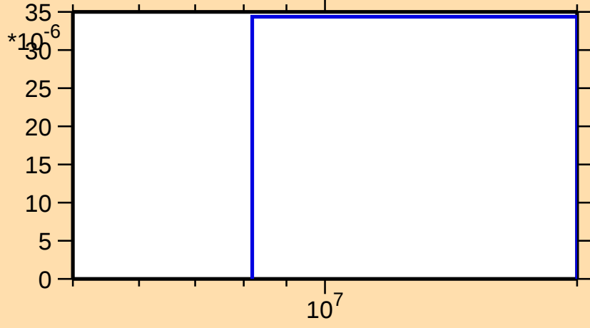
\sigma vs. E for ^{249}\text{Fm}(n,3n\alpha)
