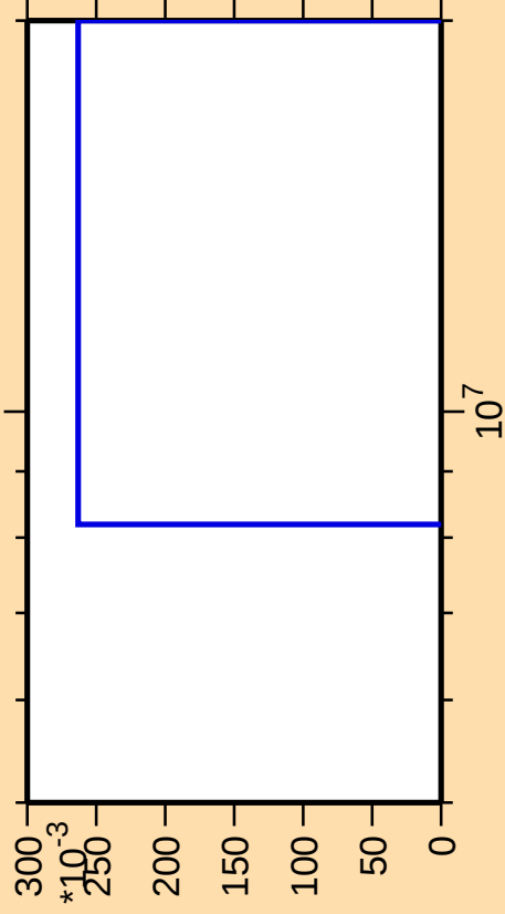
\Delta\sigma/\sigma vs. E for ^{249}\text{Fm}(\text{mt } 45)
