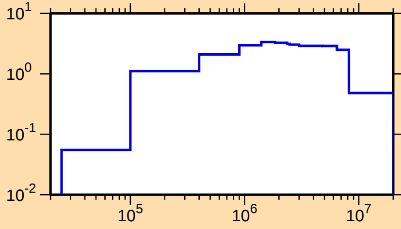
\sigma vs. E for ^{249}\text{Fm}(n,\text{inel.})
