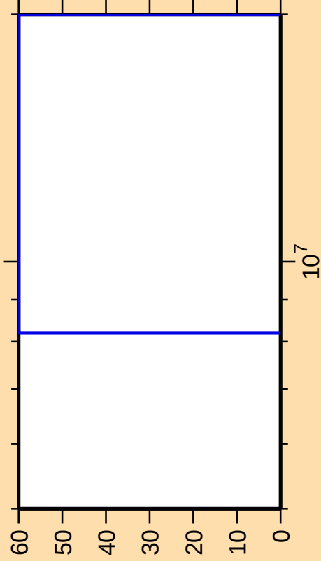
\Delta\sigma/\sigma vs. E for ^{249}\text{Fm}(n,\text{nd})
