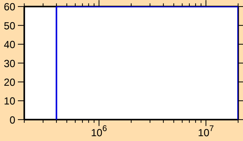
\Delta\sigma/\sigma vs. E for ^{249}\text{Fm}(n,f)
