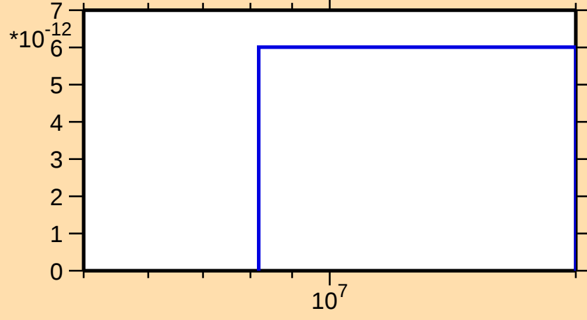
\sigma vs. E for ^{249}\text{Fm}(n,p\alpha)
