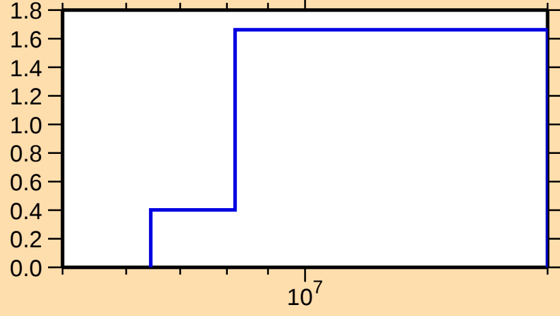
\sigma vs. E for ^{249}\text{Fm}(n,2n)
