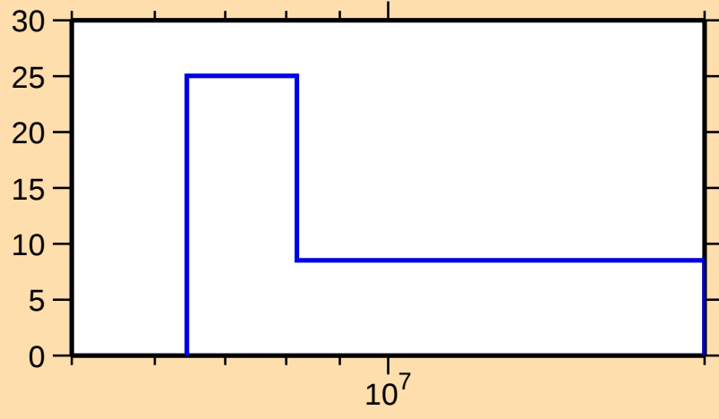
\Delta\sigma/\sigma vs. E for ^{249}\text{Fm}(n,\text{el.})
