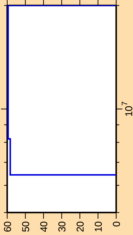
\Delta\sigma/\sigma vs. E for ^{249}\text{Fm}(n,n_1)
