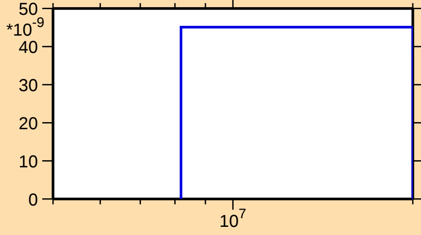
\sigma vs. E for ^{249}\text{Fm}(n,2np)
