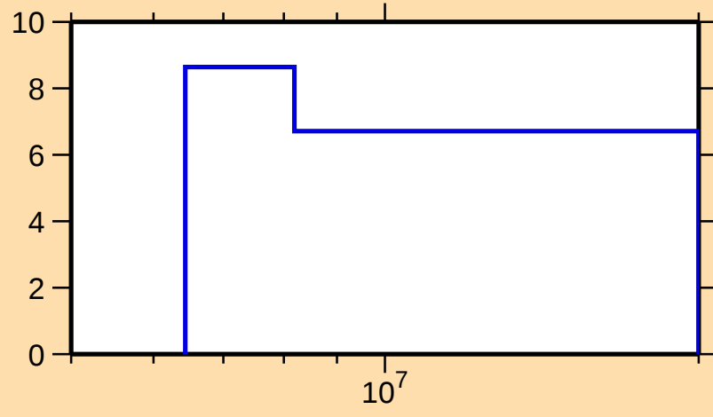
\Delta\sigma/\sigma vs. E for ^{249}\text{Fm}(n,\text{nonel.})
