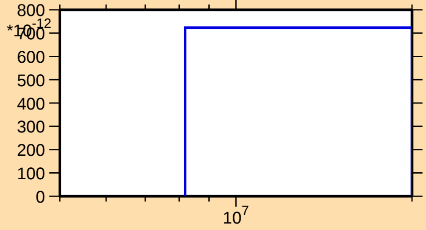
\sigma vs. E for ^{249}\text{Fm}(n,\text{He3})
