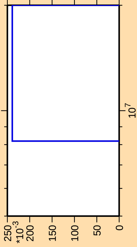
\Delta\sigma/\sigma vs. E for ^{249}\text{Fm}(\text{mt117})
