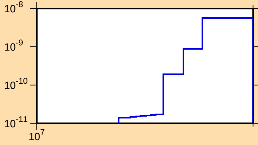
\sigma vs. E for ^{250}\text{Fm}(n,3n\alpha)
