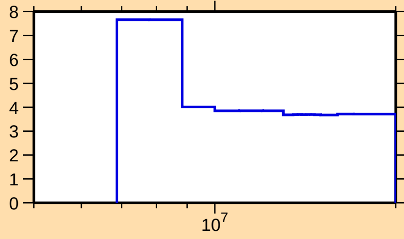
\Delta\sigma/\sigma vs. E for ^{250}\text{Fm}(n,\text{tot.})
