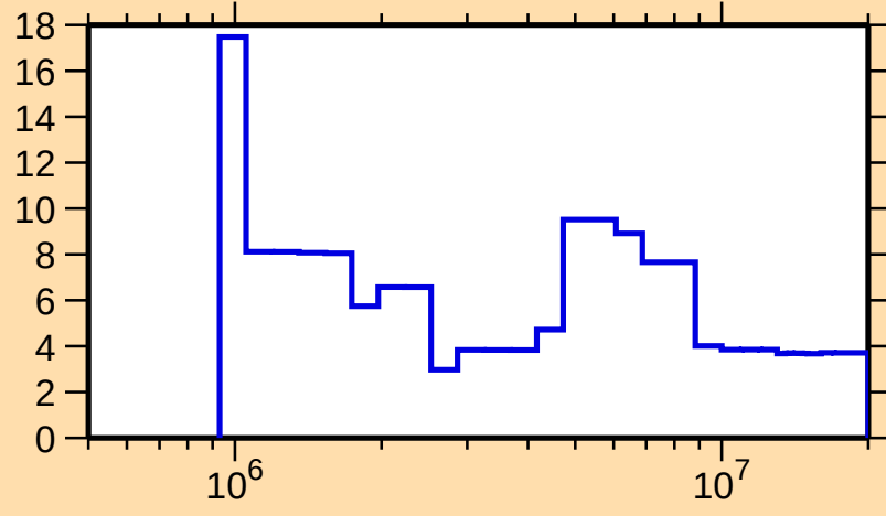
\Delta\sigma/\sigma vs. E for ^{250}\text{Fm}(n,\text{tot.})
