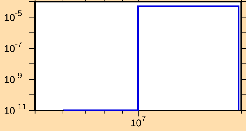
\sigma vs. E for ^{250}\text{Fm}(n,t)
