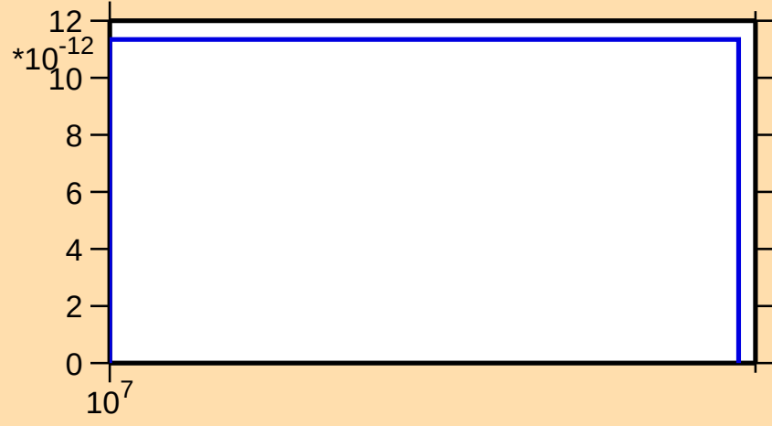
\sigma vs. E for ^{250}\text{Fm}(n,p\alpha)
