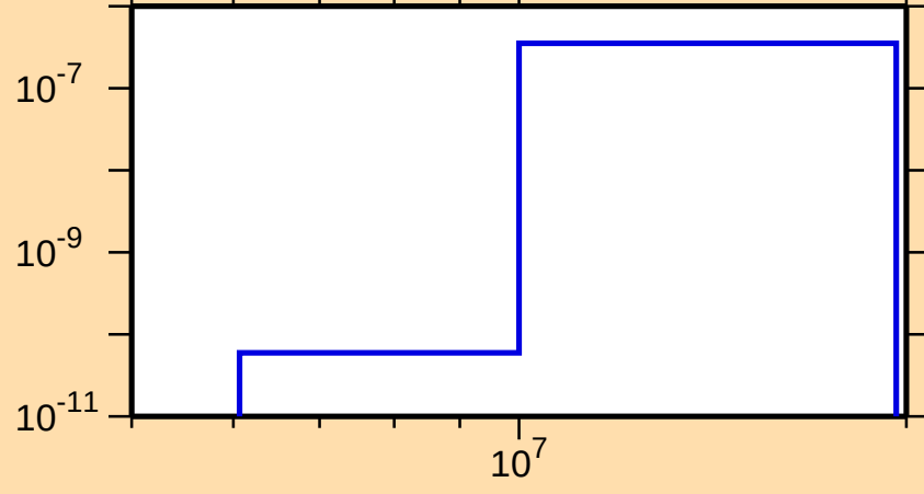
\sigma vs. E for ^{250}\text{Fm}(n,2n\alpha)
