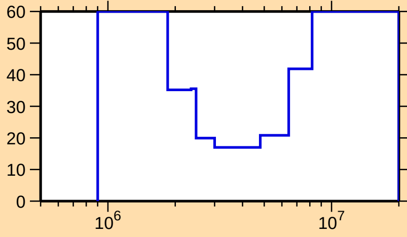
\Delta\sigma/\sigma vs. E for ^{250}\text{Fm}(n,n\text{cont.})
