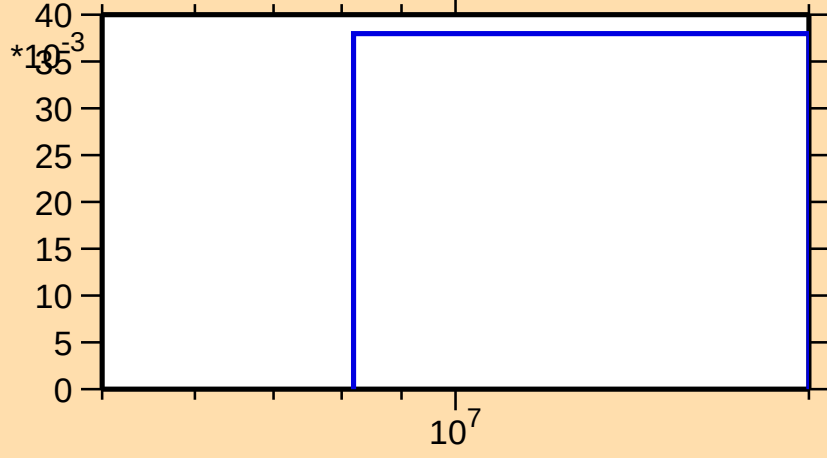
\sigma vs. E for ^{250}\text{Fm}(n,3n)
