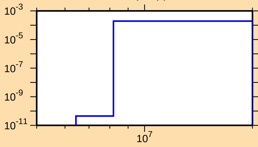
\sigma vs. E for ^{250}\text{Fm}(n,np)
