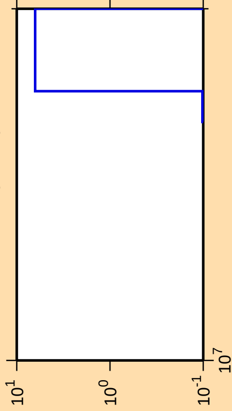
\Delta\sigma/\sigma vs. E for ^{251}\text{Fm}(\text{mt } 34)
