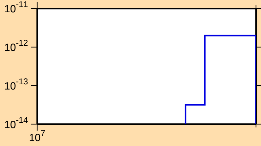
\sigma vs. E for ^{251}\text{Fm}(\text{mt } 34)
