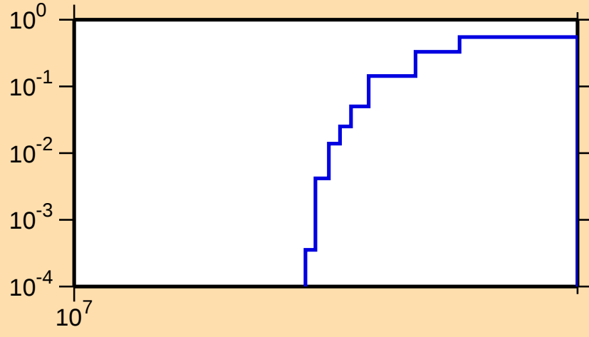
\sigma vs. E for ^{251}\text{Fm}(n,3n)
