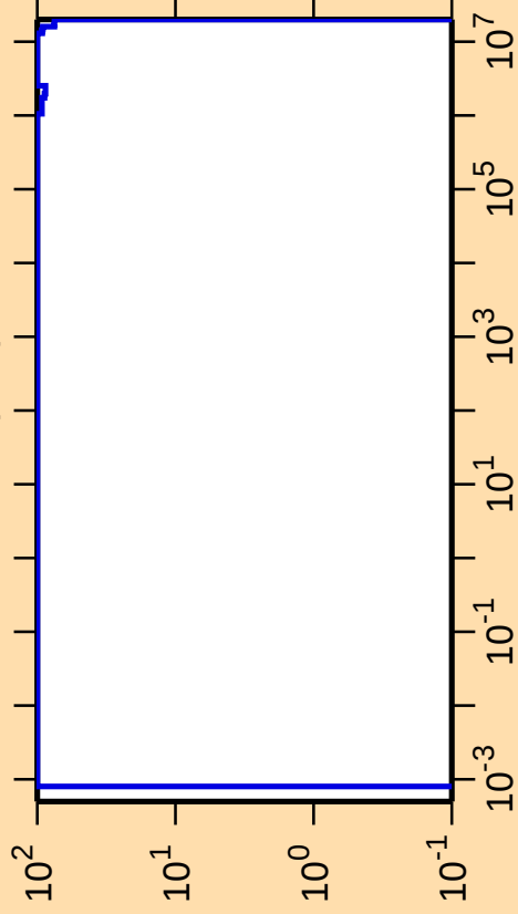
\Delta\sigma/\sigma vs. E for ^{251}\text{Fm}(n,\alpha)
