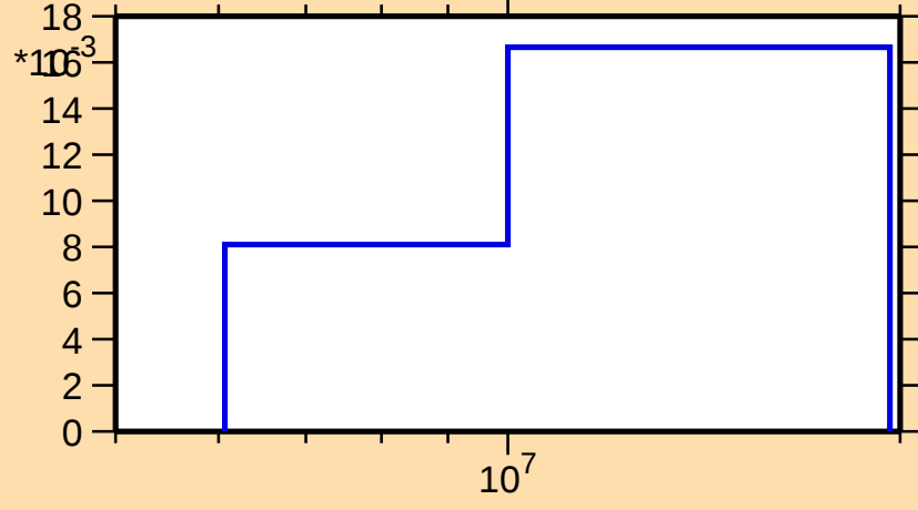
\sigma vs. E for ^{251}\text{Fm}(n,2n\alpha)
