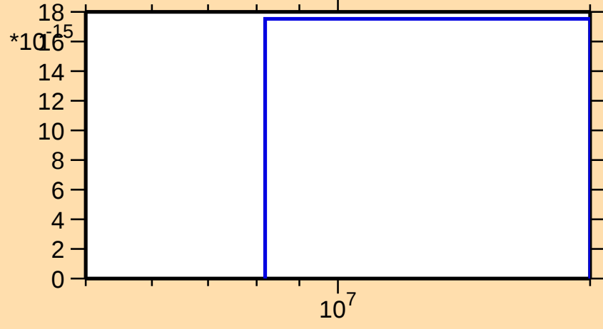
\sigma vs. E for ^{251}\text{Fm}(\text{mt } 34)
