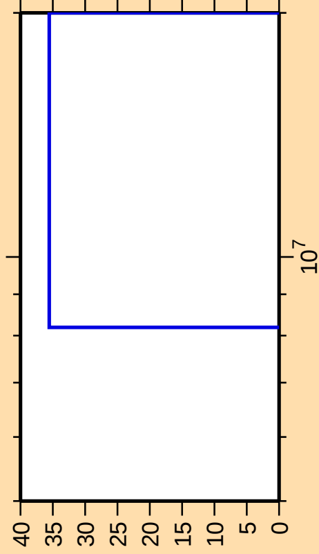
\Delta\sigma/\sigma vs. E for ^{251}\text{Fm}(n,p\alpha)
