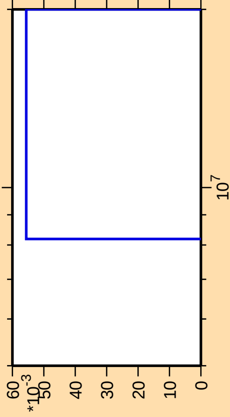
\Delta\sigma/\sigma vs. E for ^{251}\text{Fm}(\text{mt } 34)
