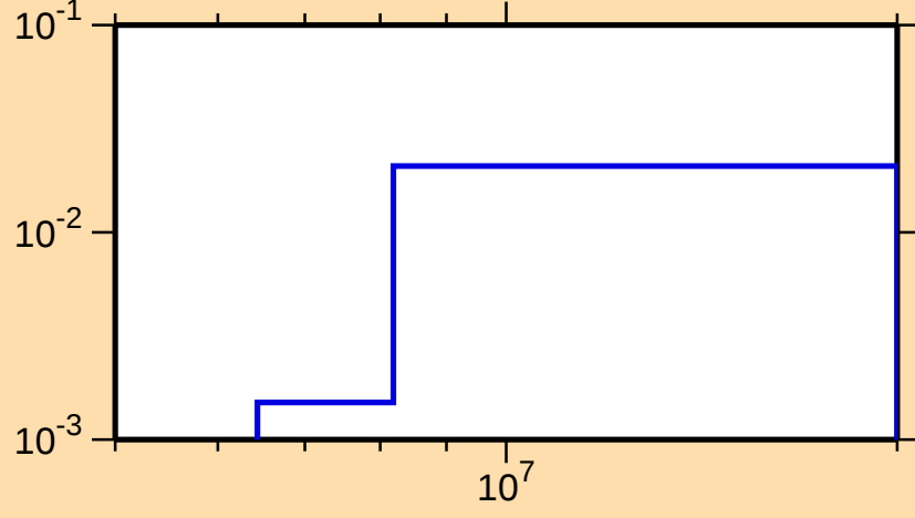
\sigma vs. E for ^{251}\text{Fm}(n,2n\alpha)
