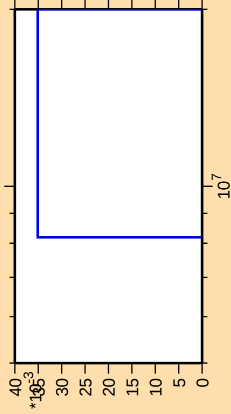
\Delta\sigma/\sigma vs. E for ^{251}\text{Fm}(\text{mt117})
