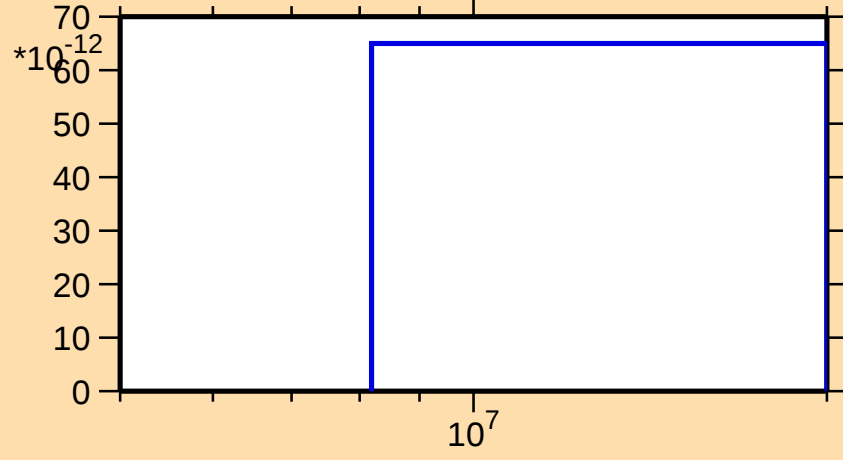
\sigma vs. E for ^{251}\text{Fm}(n,\text{He}3)
