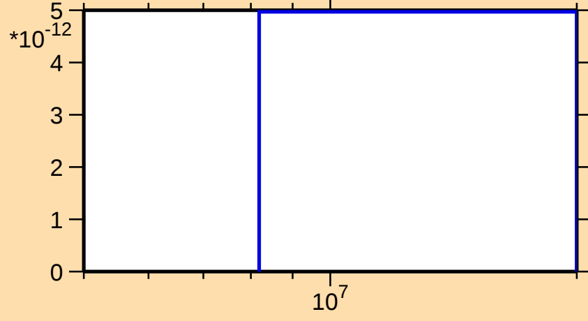
\sigma vs. E for ^{251}\text{Fm}(n,p\alpha)
