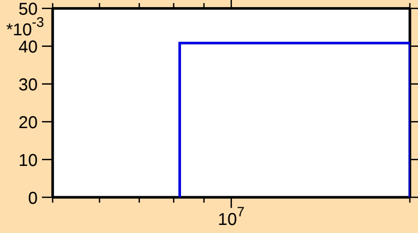
\sigma vs. E for ^{251}\text{Fm}(n,3n)
