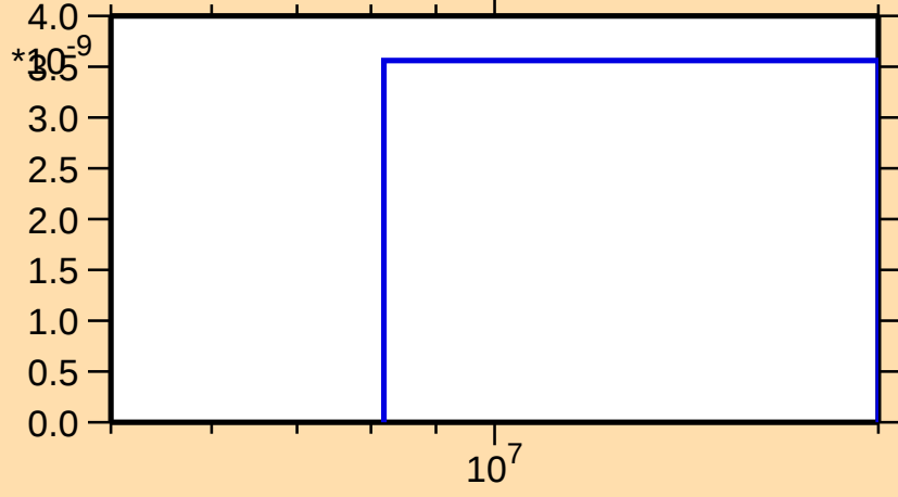
\sigma vs. E for ^{251}\text{Fm}(n,nt)
