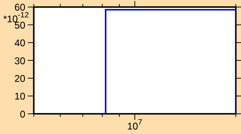
\sigma vs. E for ^{251}\text{Fm}(n,3n\alpha)
