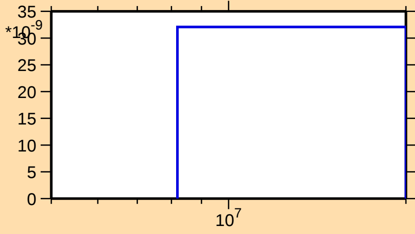
\sigma vs. E for ^{251}\text{Fm}(n,\text{nd})
