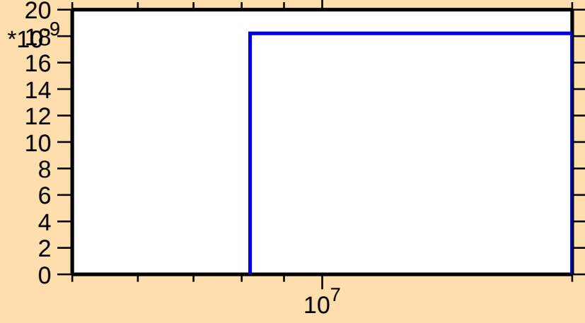
\sigma vs. E for ^{251}\text{Fm}(n,2np)
