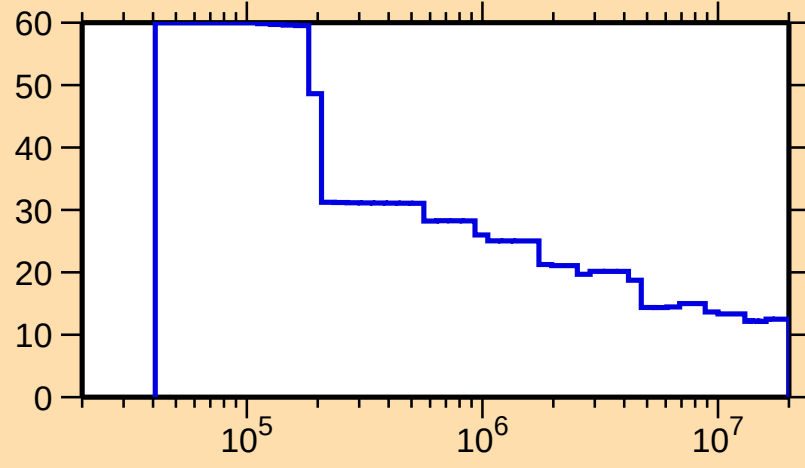
\Delta\sigma/\sigma vs. E for ^{254}\text{Fm}(n,\text{nonel.})
