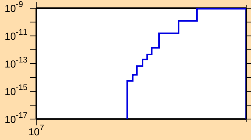
\sigma vs. E for ^{254}\text{Fm}(n,3n\alpha)
