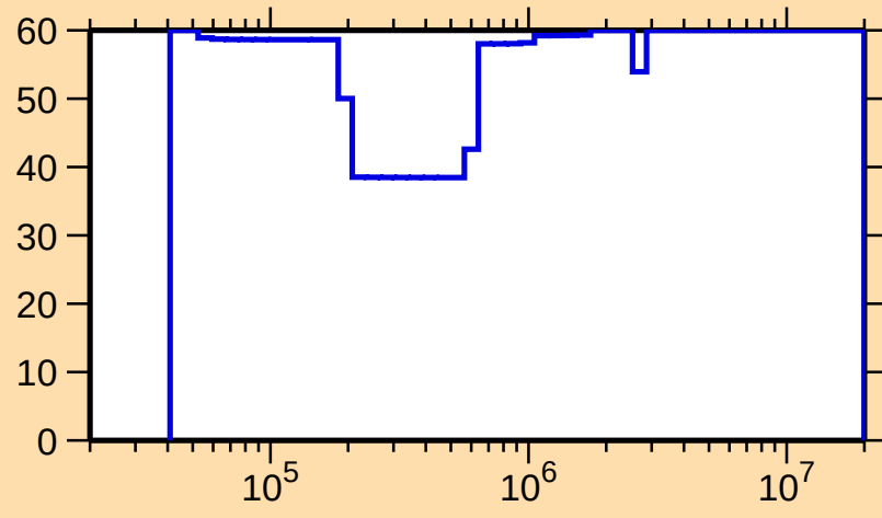
\Delta\sigma/\sigma vs. E for ^{254}\text{Fm}(n, n_1)
