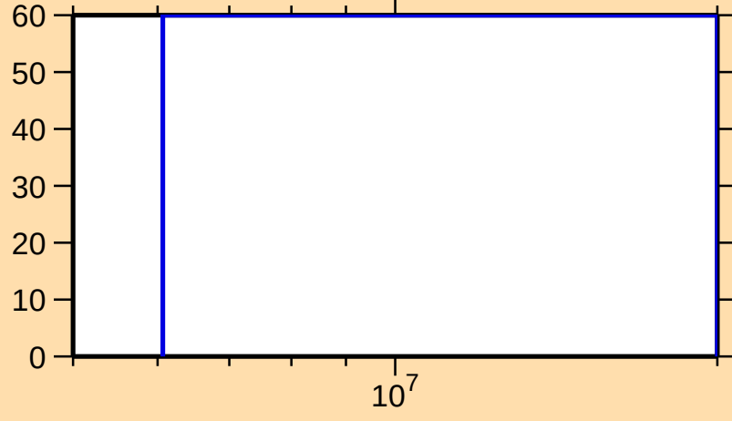
\Delta\sigma/\sigma vs. E for ^{254}\text{Fm}(n,2n)
