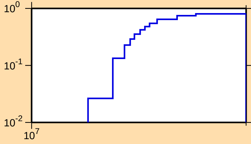
\sigma vs. E for ^{254}\text{Fm}(n,3n)
