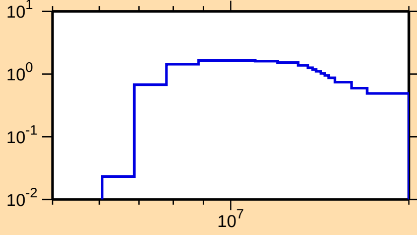
\sigma vs. E for ^{254}\text{Fm}(n,2n)
