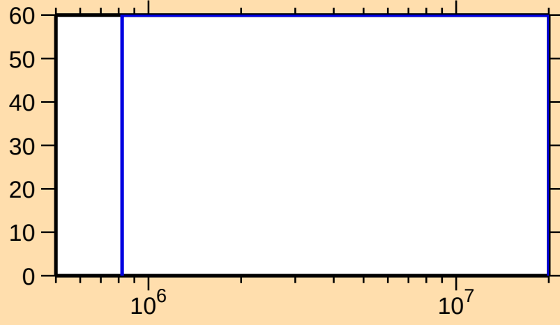
\Delta\sigma/\sigma vs. E for ^{254}\text{Fm}(n,f)
