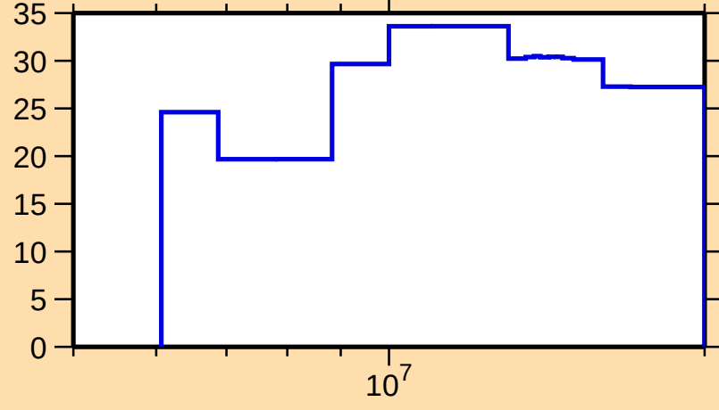
\Delta\sigma/\sigma vs. E for ^{254}\text{Fm}(n,\text{el.})
