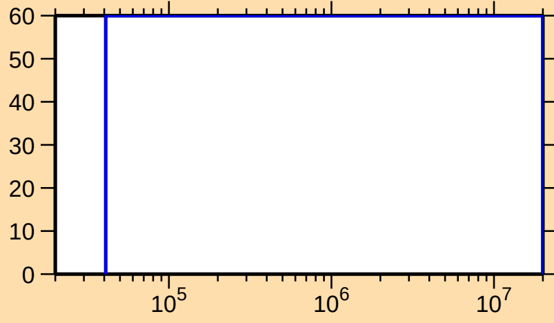
\Delta\sigma/\sigma vs. E for ^{254}\text{Fm}(n,f)
