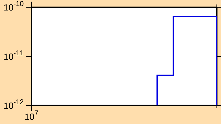
\sigma vs. E for ^{254}\text{Fm}(n,\text{He3})
