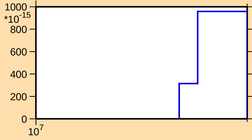
\sigma vs. E for ^{254}\text{Fm}(n,p\alpha)
