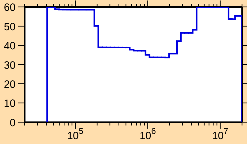
\Delta\sigma/\sigma vs. E for ^{254}\text{Fm}(n,\text{inel.})
