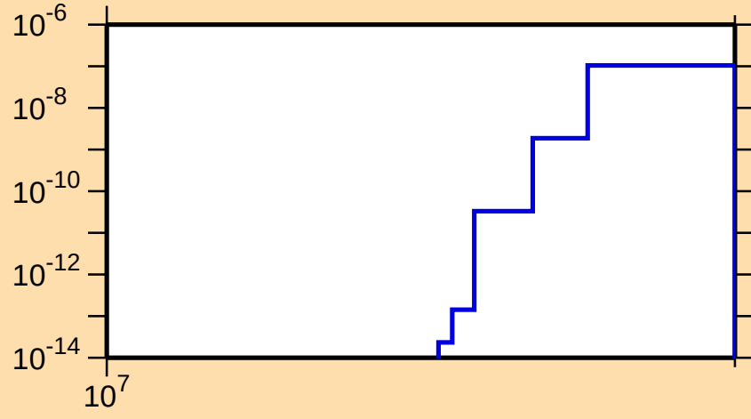
\sigma vs. E for ^{254}\text{Fm}(n,2np)
