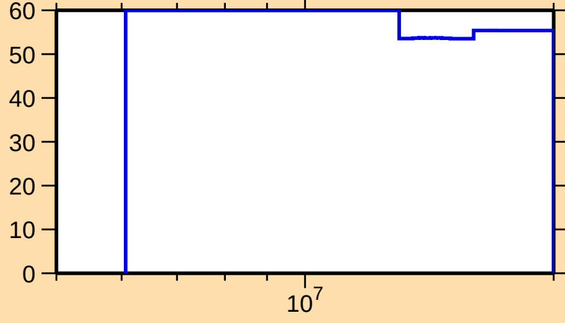
\Delta\sigma/\sigma vs. E for ^{254}\text{Fm}(n,\text{inel.})
