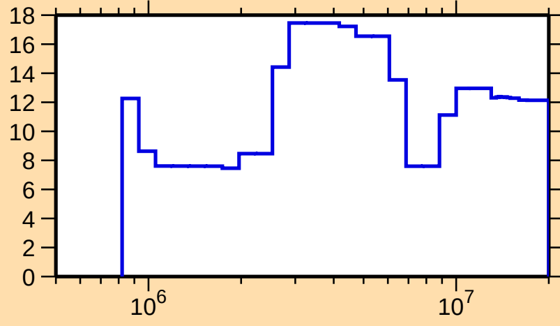
\Delta\sigma/\sigma vs. E for ^{254}\text{Fm}(n,\text{tot.})
