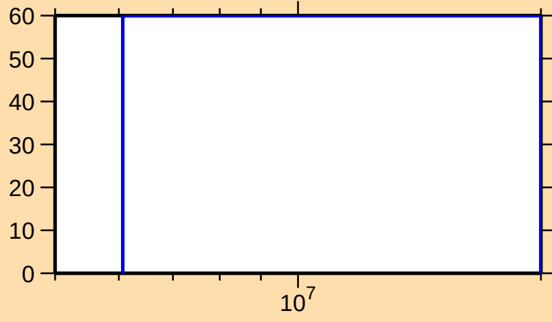
\Delta\sigma/\sigma vs. E for ^{254}\text{Fm}(n,2n)
