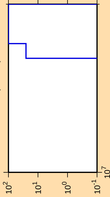
\Delta\sigma/\sigma vs. E for ^{254}\text{Fm}(n,\text{He3})
