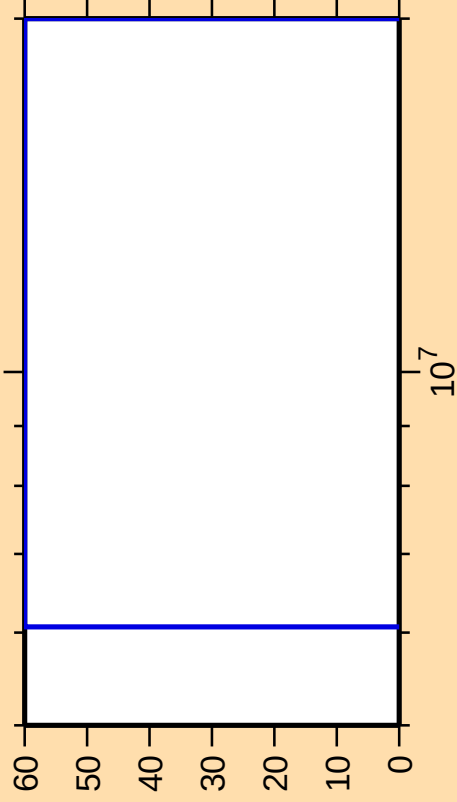
\Delta\sigma/\sigma vs. E for ^{254}\text{Fm}(n,n_1)
