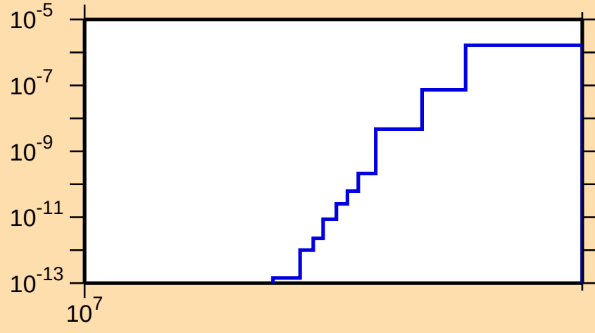
\sigma vs. E for ^{254}\text{Fm}(n,nt)
