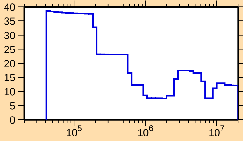
\Delta\sigma/\sigma vs. E for ^{254}\text{Fm}(n,\text{tot.})
