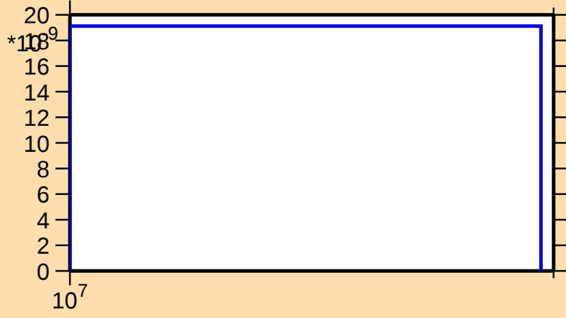
\sigma vs. E for ^{254}\text{Fm}(n,nt)
