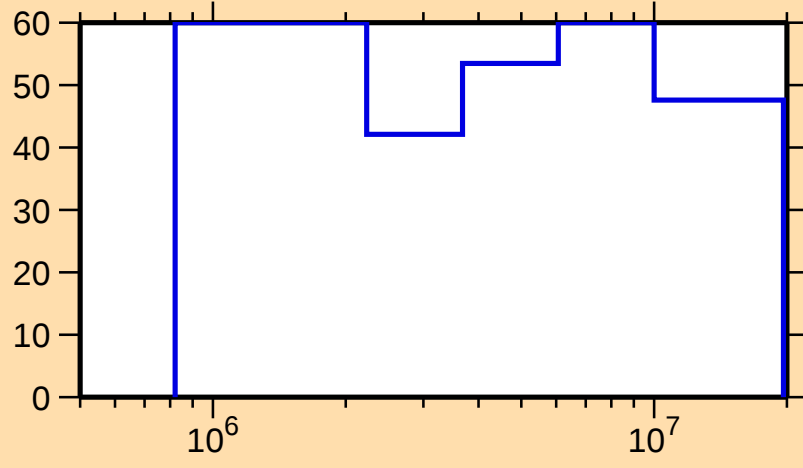
\Delta\sigma/\sigma vs. E for ^{254}\text{Fm}(n,n\text{cont.})
