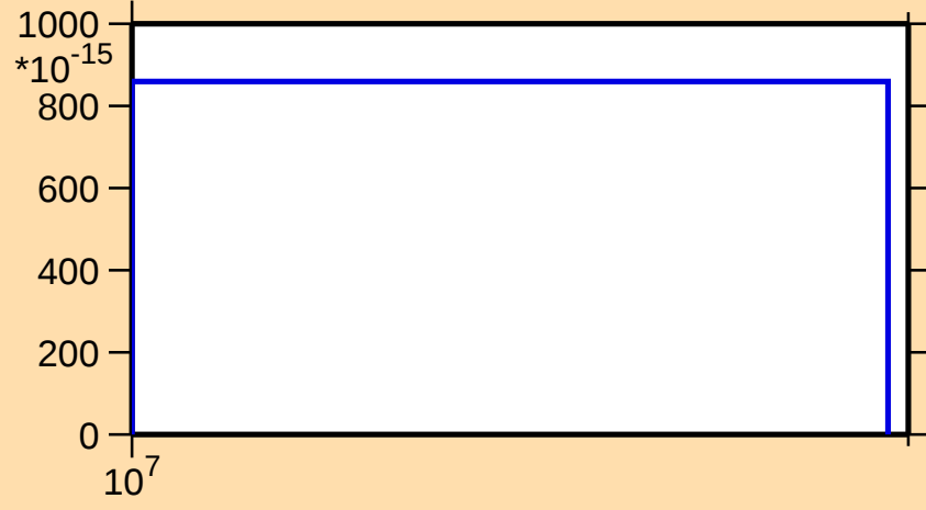
\sigma vs. E for ^{254}\text{Fm}(n,\text{He3})
