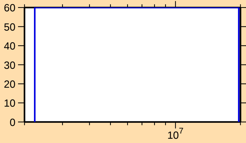
\Delta\sigma/\sigma vs. E for ^{254}\text{Fm}(n,n_1)
