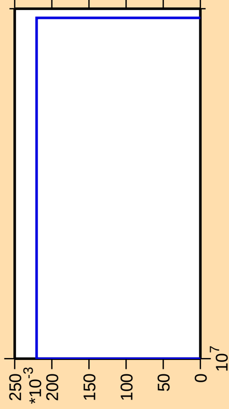
\Delta\sigma/\sigma vs. E for ^{254}\text{Fm}(n,p\alpha)
