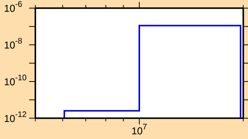
\sigma vs. E for ^{254}\text{Fm}(n,2n\alpha)
