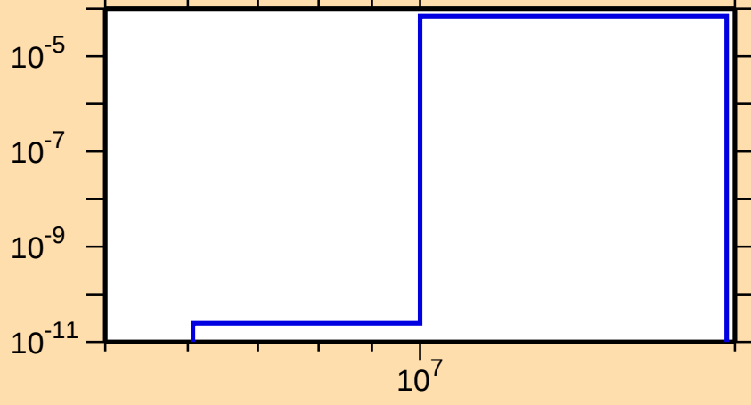
\sigma vs. E for ^{254}\text{Fm}(n,np)
