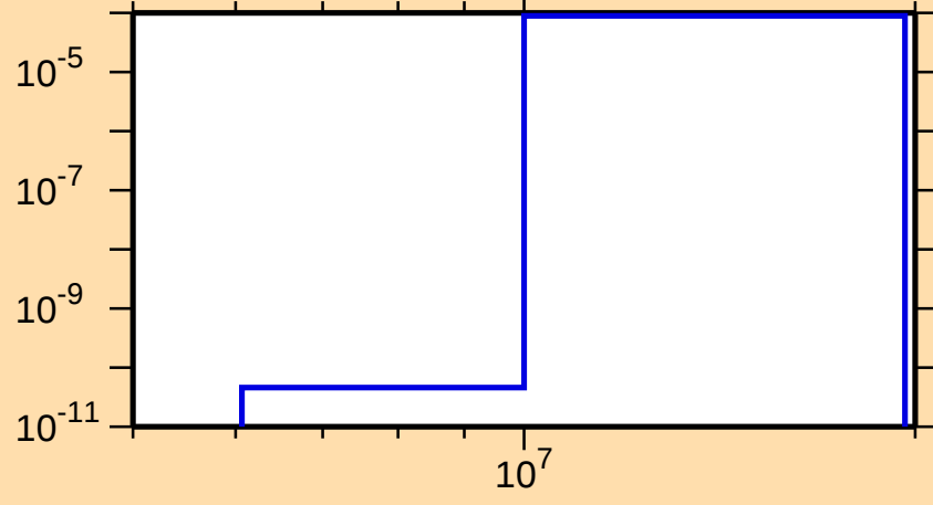
\sigma vs. E for ^{254}\text{Fm}(n,d)
