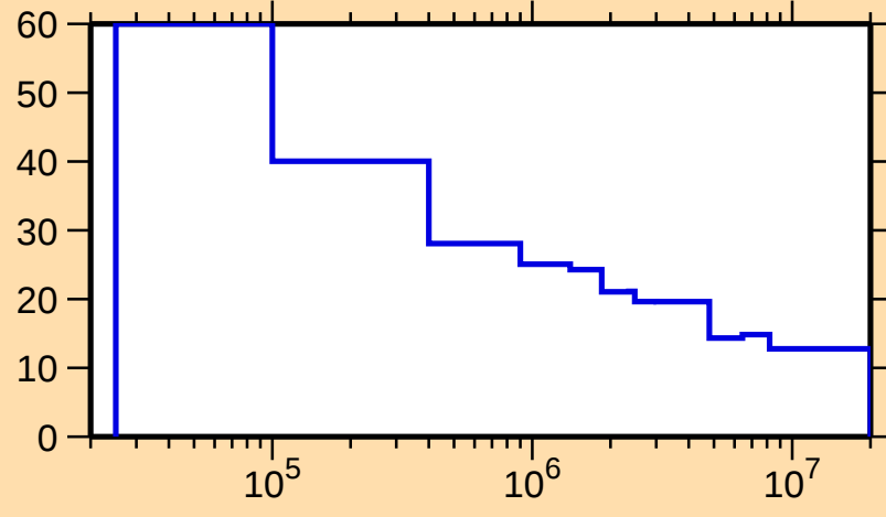
\Delta\sigma/\sigma vs. E for ^{254}\text{Fm}(n,\text{nonel.})
