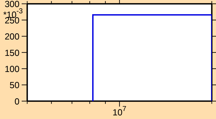
\sigma vs. E for ^{254}\text{Fm}(n,3n)
