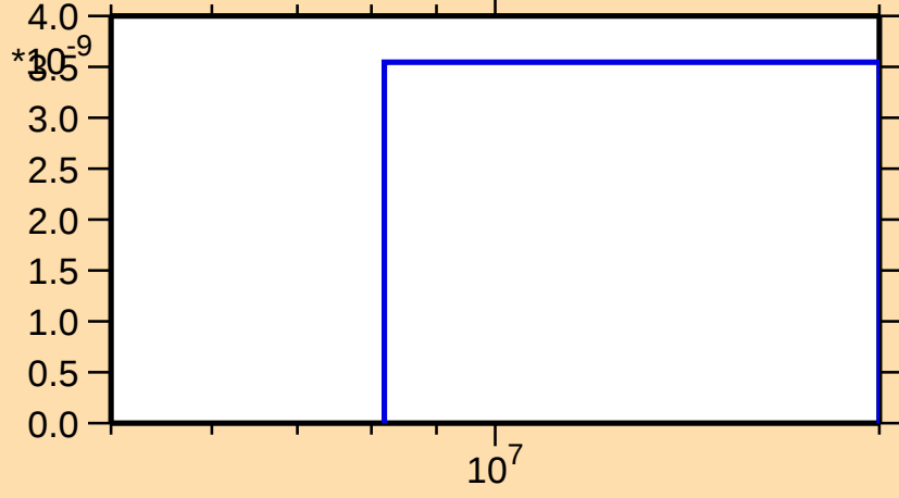
\sigma vs. E for ^{254}\text{Fm}(n,\text{nd})
