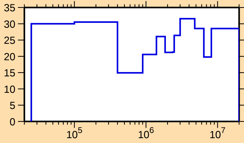
\Delta\sigma/\sigma vs. E for ^{254}\text{Fm}(n,\text{el.})
