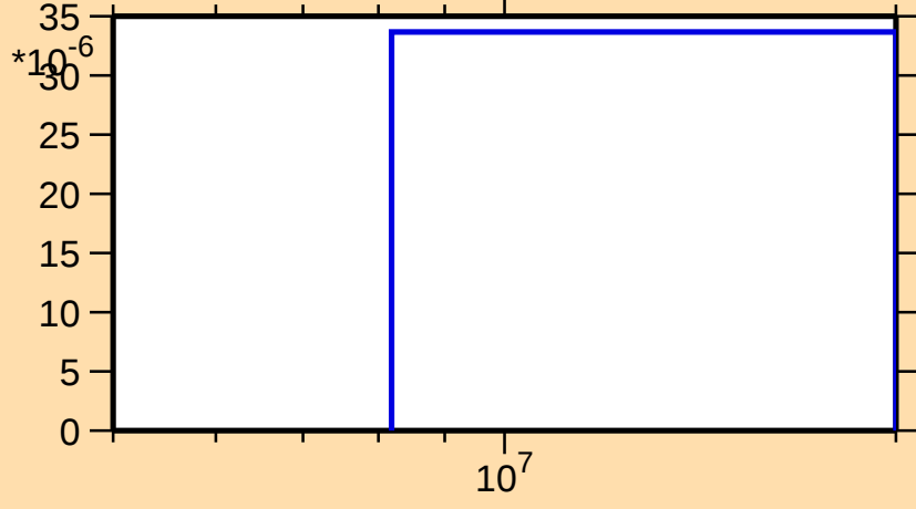
\sigma vs. E for ^{254}\text{Fm}(n,t)
