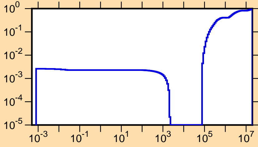
\mu vs. E for ^{256}\text{Fm}(\text{mt251})
