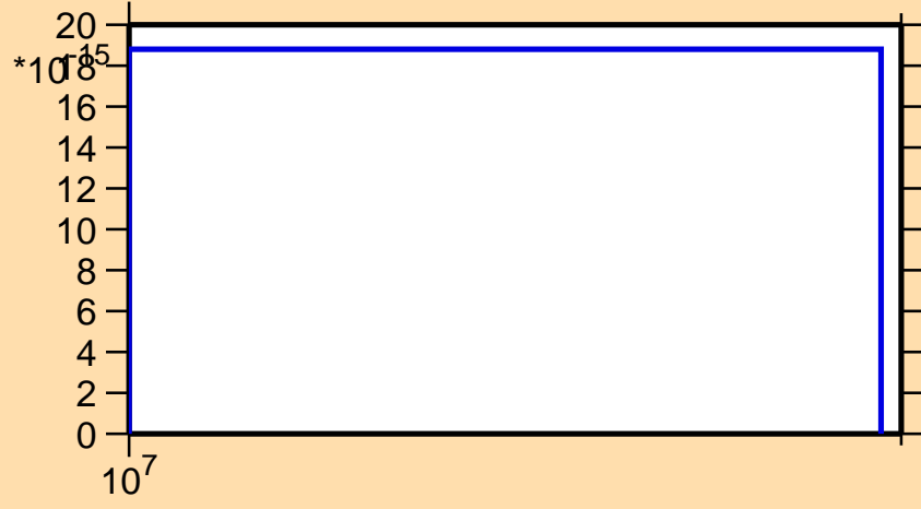
\sigma vs. E for ^{221}\text{Fr} (mt 42)
