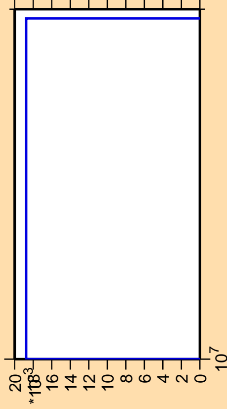
\Delta\sigma/\sigma vs. E for ^{221}\text{Fr} (mt 42)
