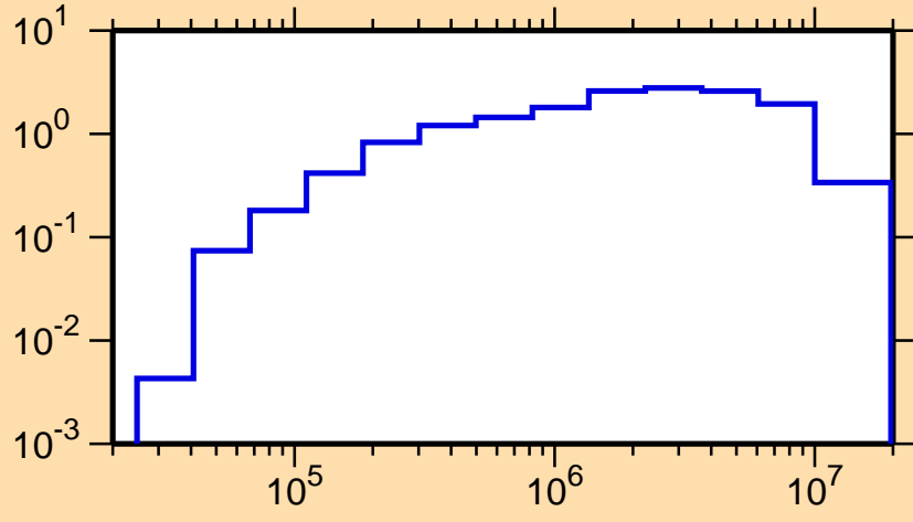
\sigma vs. E for ^{221}\text{Fr}(n,\text{inel.})
