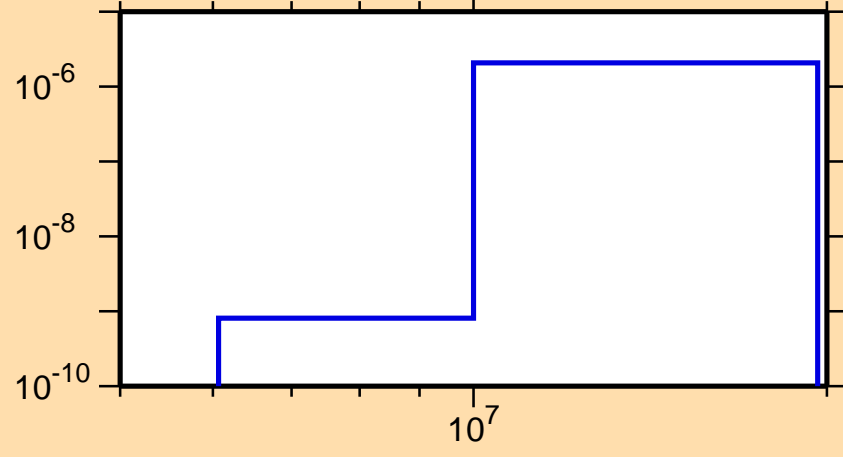
\sigma vs. E for ^{221}\text{Fr}(n,2n\alpha)
