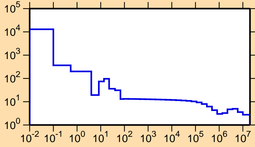
\sigma vs. E for ^{221}\text{Fr}(n,\text{el.})
