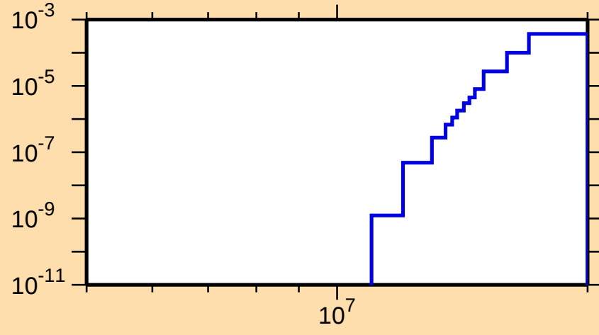
\sigma vs. E for ^{232}\text{Fr}(n,np)
