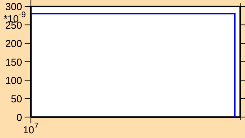
\sigma vs. E for ^{232}\text{Fr}(n,\text{nt})
