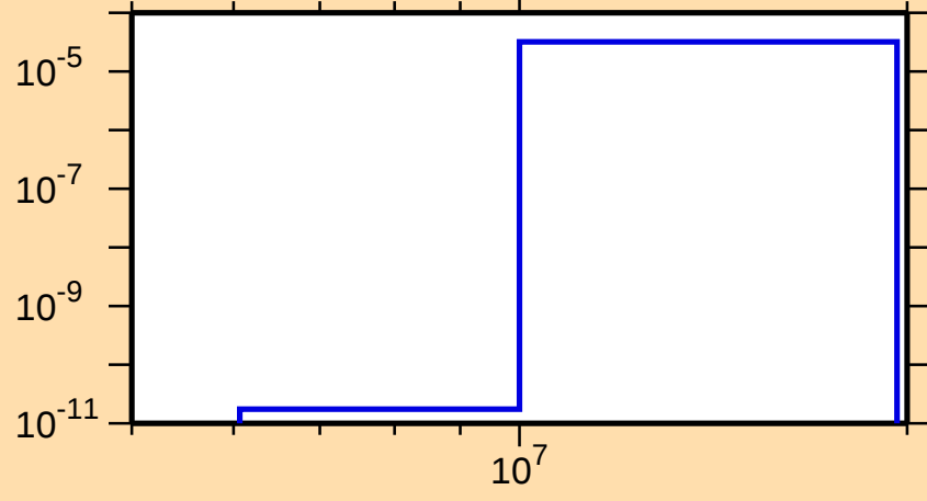
\sigma vs. E for ^{232}\text{Fr}(n,t)
