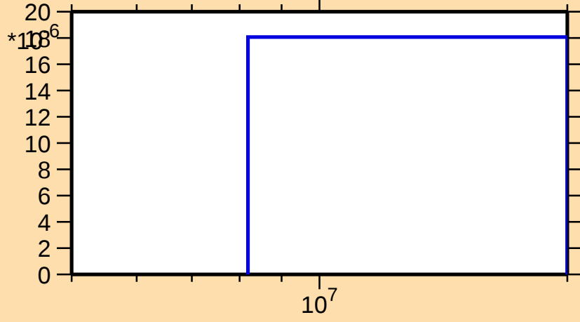
\sigma vs. E for ^{232}\text{Fr}(n,d)
