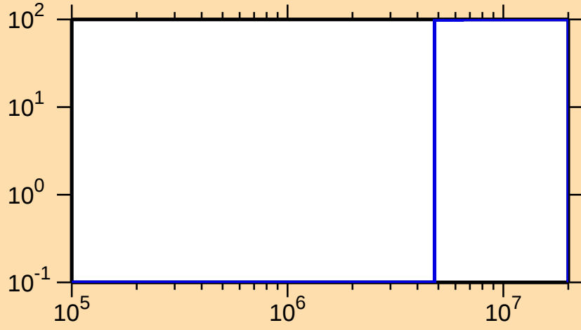
\Delta\sigma/\sigma vs. E for ^{232}\text{Fr}(n,\text{f})
