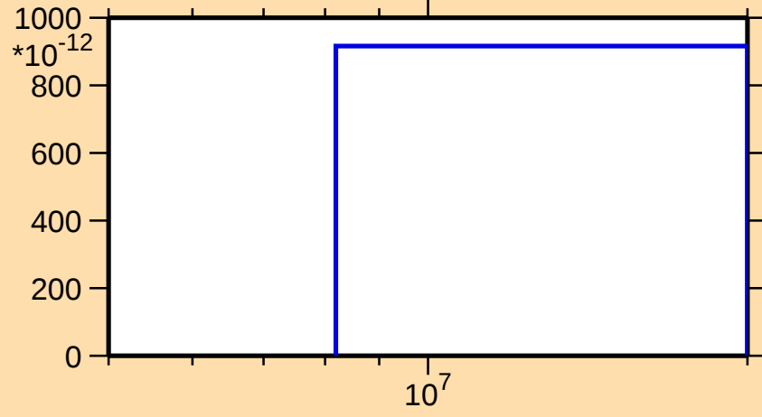
\sigma vs. E for ^{232}\text{Fr}(n,2n\alpha)
