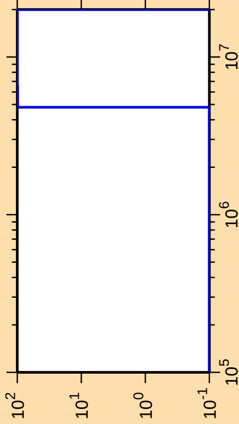
\Delta\sigma/\sigma vs. E for ^{232}\text{Fr}(n,f)
