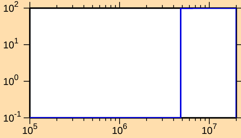
\Delta\sigma/\sigma vs. E for ^{232}\text{Fr}(n,f)
