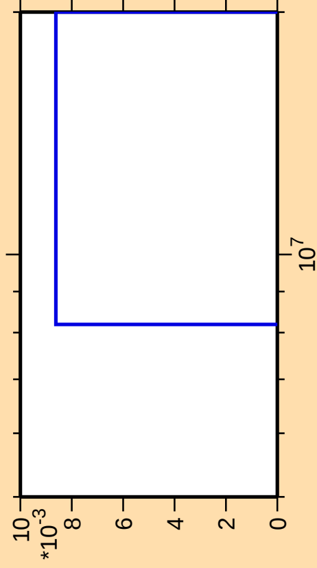
\Delta\sigma/\sigma vs. E for ^{232}\text{Fr}(n,3n\alpha)
