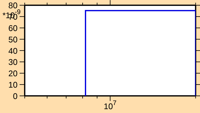
\sigma vs. E for ^{232}\text{Fr}(n,\text{nd})
