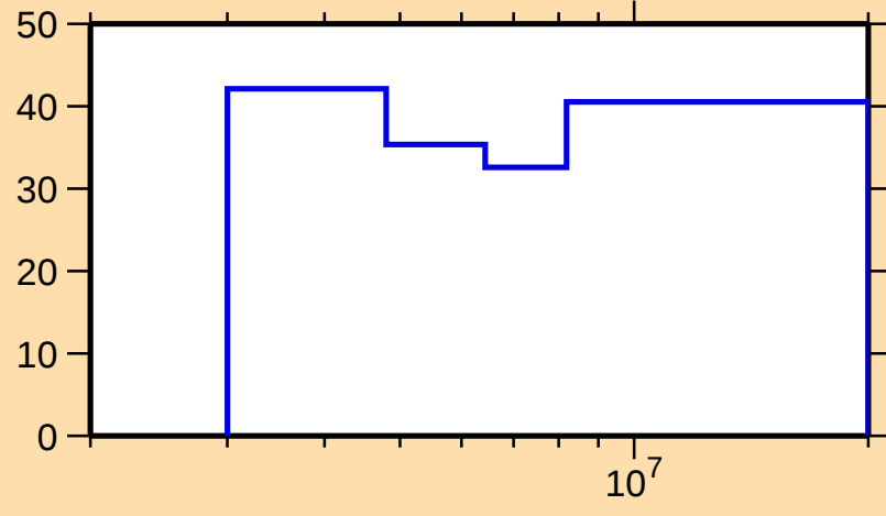
\Delta\sigma/\sigma vs. E for ^{232}\text{Fr}(n,\text{tot.})
