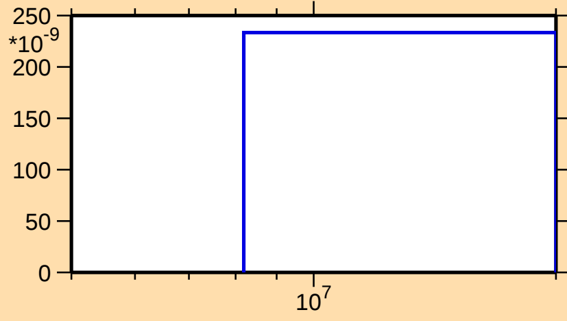
\sigma vs. E for ^{232}\text{Fr}(n,nt)
