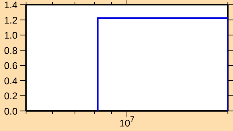
\sigma vs. E for ^{232}\text{Fr}(n,3n)
