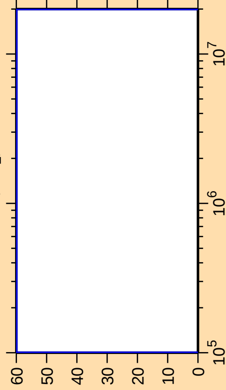
\Delta\sigma/\sigma vs. E for ^{232}\text{Fr}(n,n_1)
