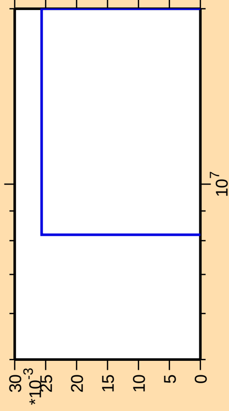
\Delta\sigma/\sigma vs. E for ^{232}\text{Fr}(\text{mt 11})
