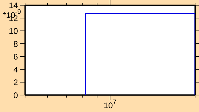
\sigma vs. E for ^{232}\text{Fr}(n,2np)
