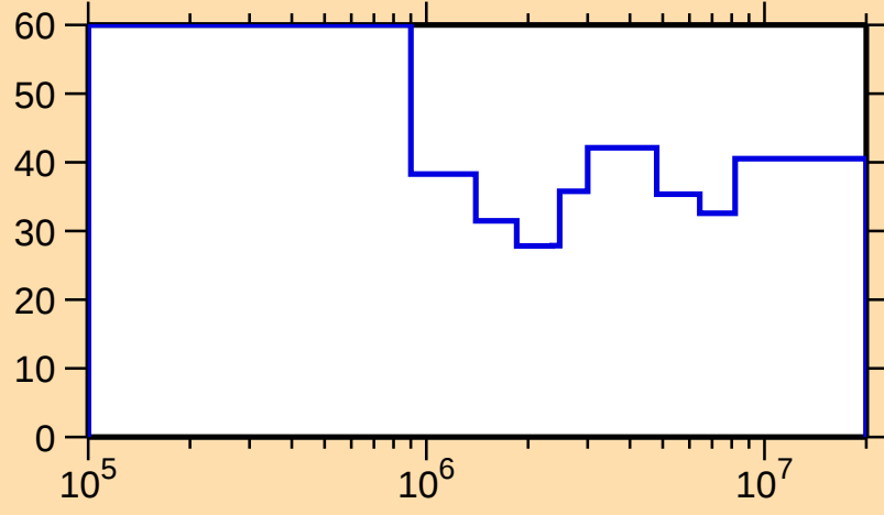
\Delta\sigma/\sigma vs. E for ^{232}\text{Fr}(n,\text{tot.})
