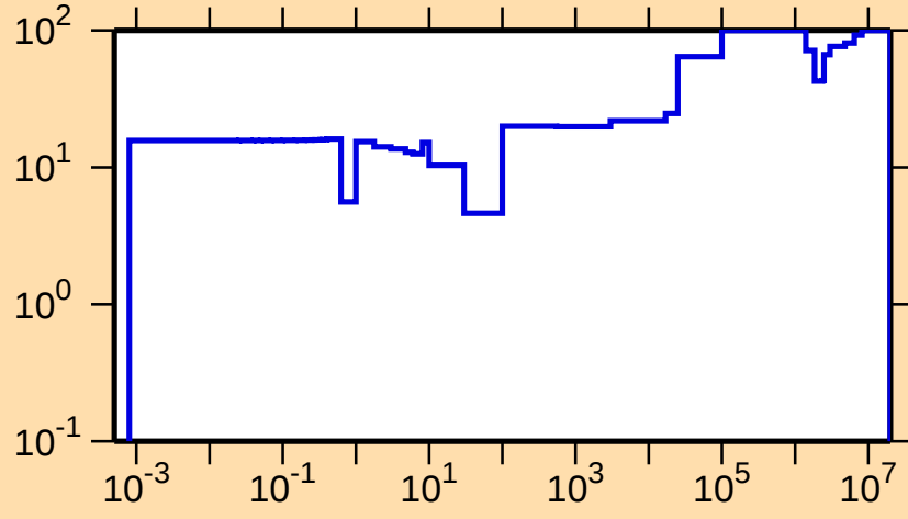
\Delta\sigma/\sigma vs. E for ^{232}\text{Fr}(n,\text{el.})
