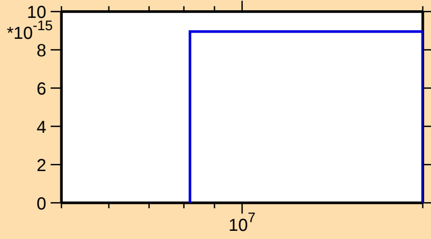
\sigma vs. E for ^{232}\text{Fr}(n,3n\alpha)
