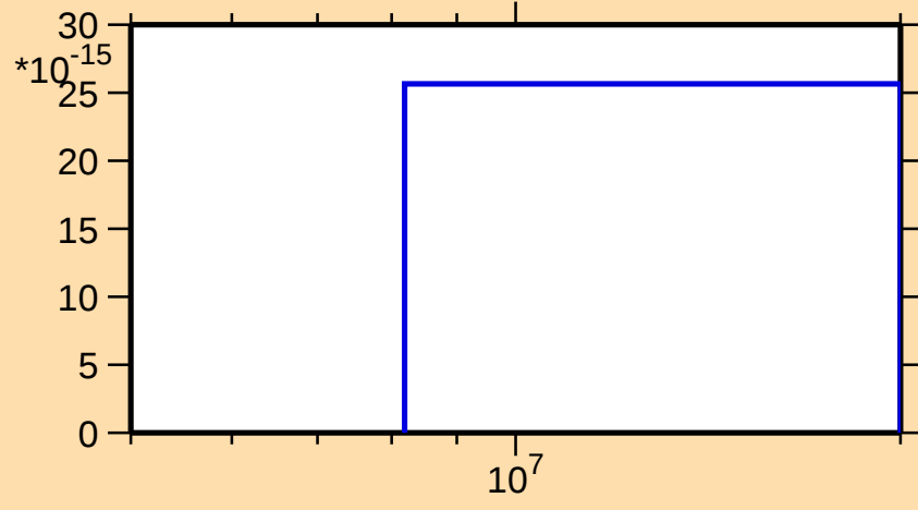
\sigma vs. E for ^{232}\text{Fr}(\text{mt 11})
