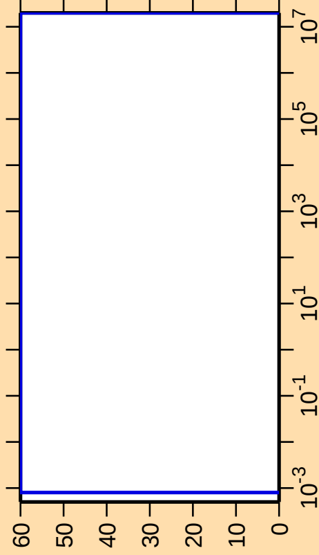
\Delta\sigma/\sigma vs. E for ^{232}\text{Fr}(n,\text{nonel.})
