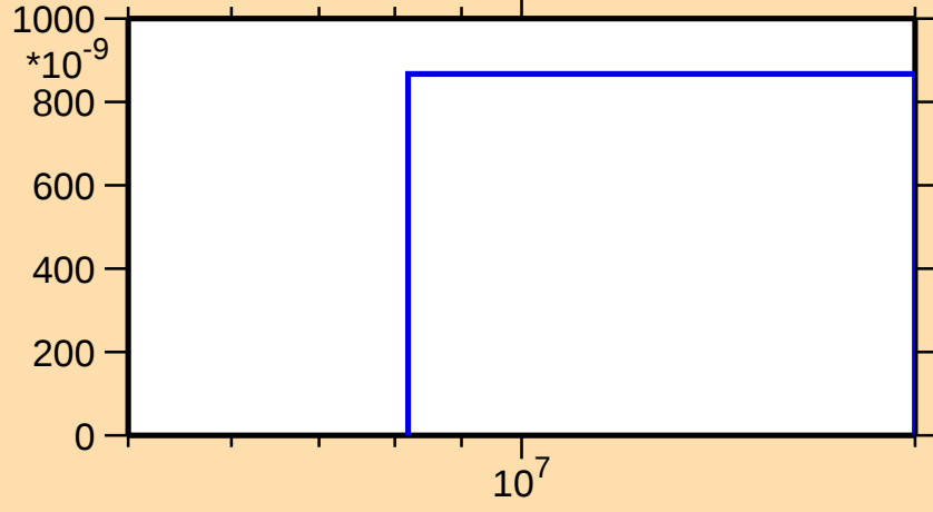
\sigma vs. E for ^{232}\text{Fr}(n,n\alpha)
