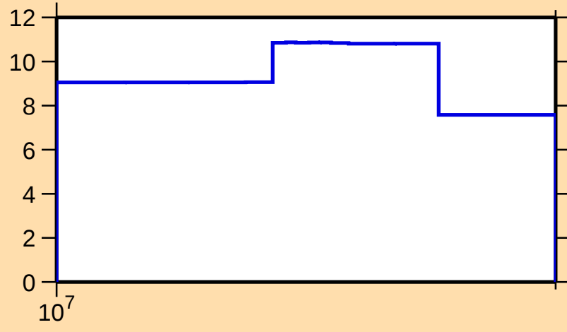
\Delta\sigma/\sigma vs. E for ^{64}\text{Ga}(n,\text{el.})
