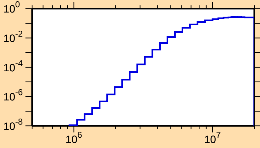
\sigma vs. E for ^{64}\text{Ga}(n,p\alpha)
