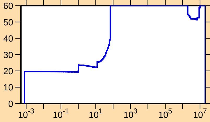
\Delta\sigma/\sigma vs. E for ^{64}\text{Ga}(n,\gamma)
