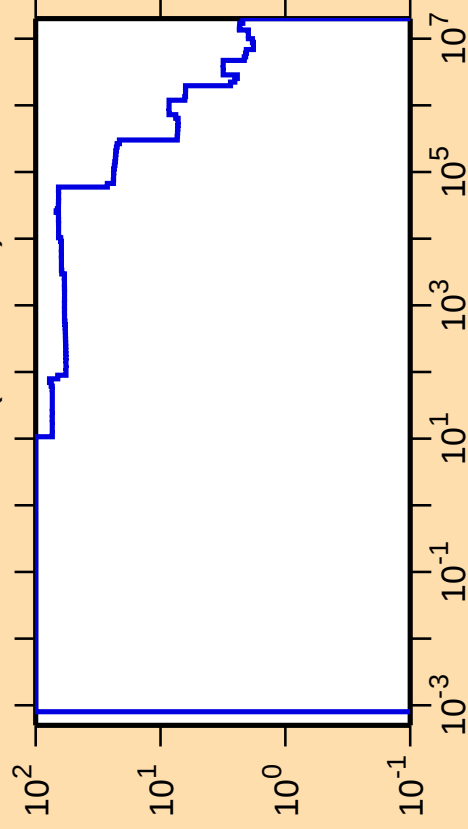
\Delta\sigma/\sigma vs. E for ^{64}\text{Ga}(n,\text{nonel.})
