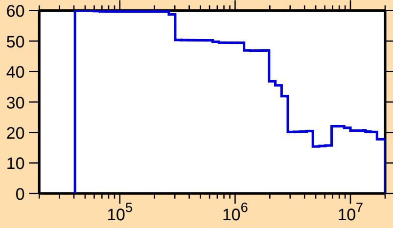
\Delta\sigma/\sigma vs. E for ^{64}\text{Ga}(n,n_1)
