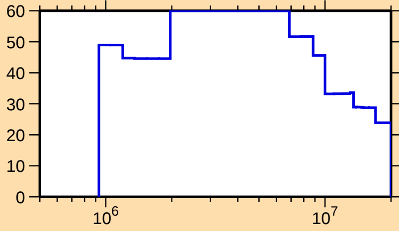
\Delta\sigma/\sigma vs. E for ^{64}\text{Ga}(n,\text{inel.})
