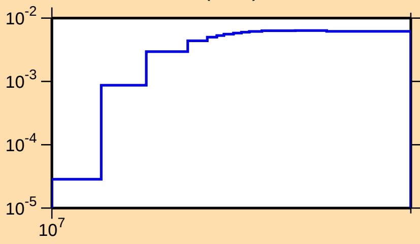
\sigma vs. E for ^{64}\text{Ga}(n,2n)
