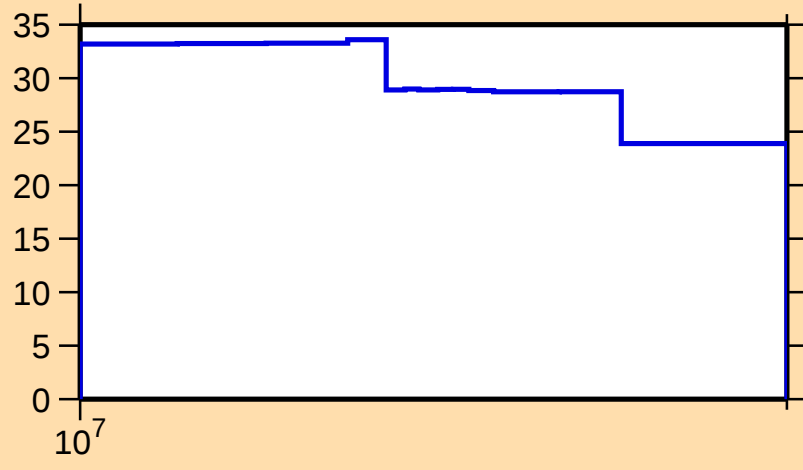
\Delta\sigma/\sigma vs. E for ^{64}\text{Ga}(n,\text{inel.})
