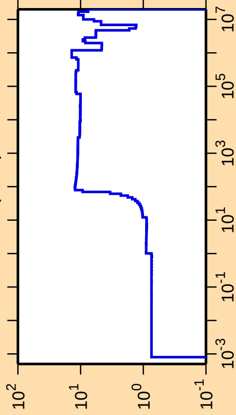
\Delta\sigma/\sigma vs. E for ^{64}\text{Ga}(n,\text{el.})
