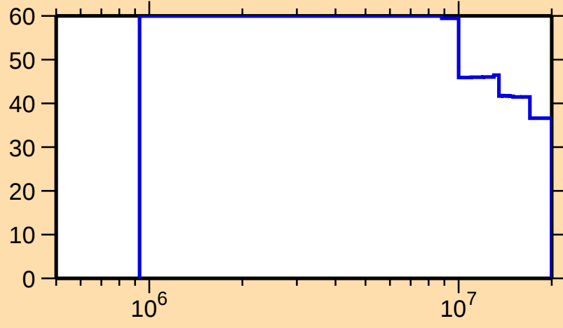
\Delta\sigma/\sigma vs. E for ^{64}\text{Ga}(n,n\text{cont.})
