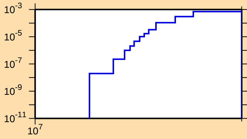
\sigma vs. E for ^{64}\text{Ga}(n,\text{nd})
