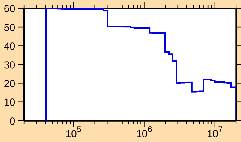
\Delta\sigma/\sigma vs. E for ^{64}\text{Ga}(n, n_1)
