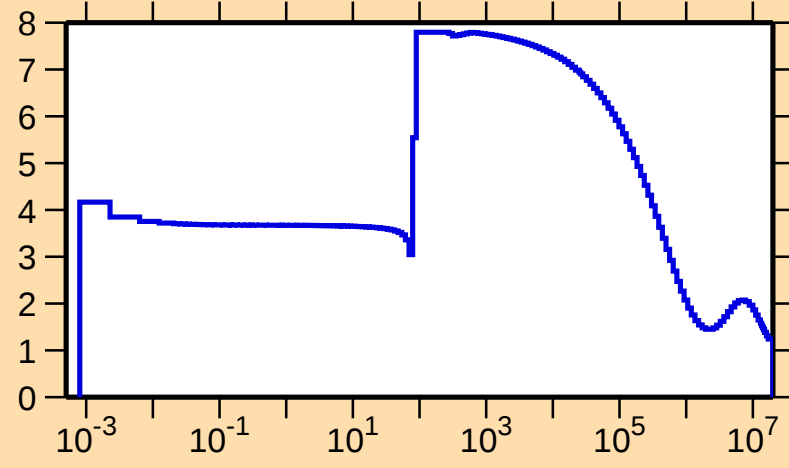
\sigma vs. E for ^{64}\text{Ga}(n,\text{el.})
