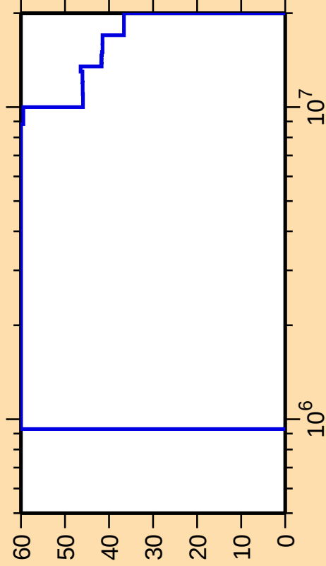
\Delta\sigma/\sigma vs. E for ^{64}\text{Ga}(n,\text{ncont.})
