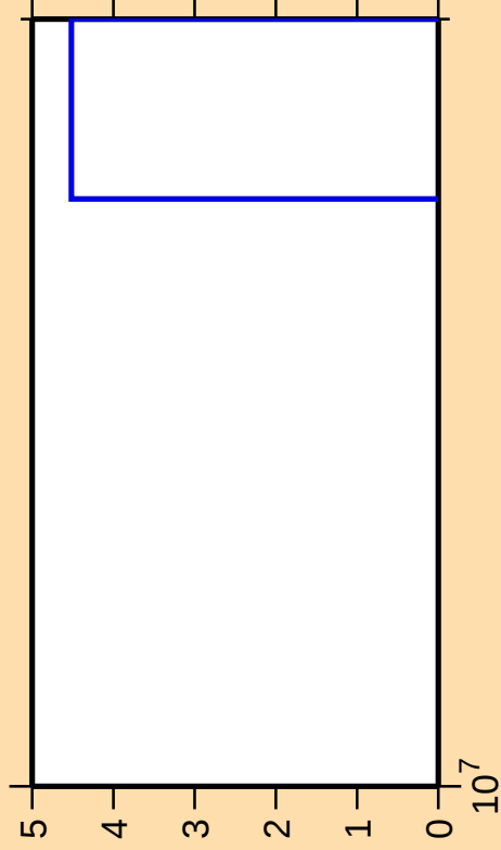
\Delta\sigma/\sigma vs. E for ^{64}\text{Ga}(n,\text{nt})
