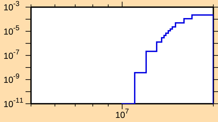
\sigma vs. E for ^{64}\text{Ga}(\text{mt117})
