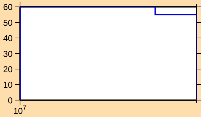
\Delta\sigma/\sigma vs. E for ^{64}\text{Ga}(n,2n)
