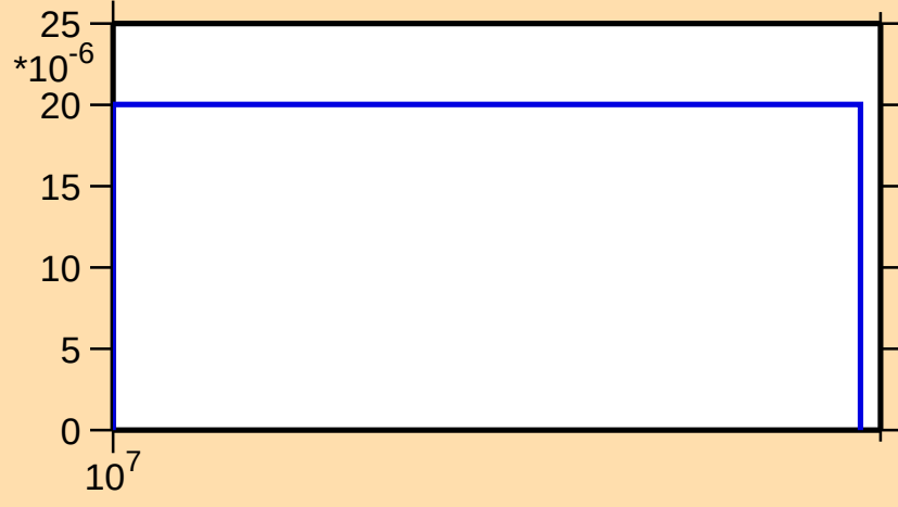
\sigma vs. E for ^{70}\text{Ga}(n,2np)
