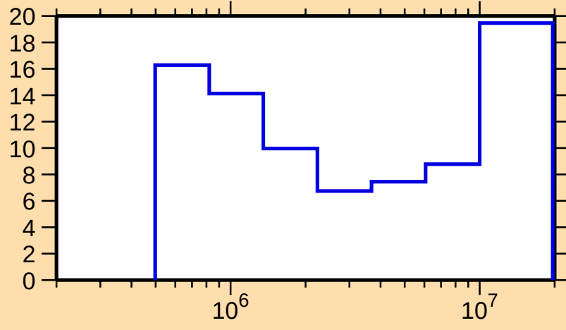
\Delta\sigma/\sigma vs. E for ^{70}\text{Ga}(\text{n,el.})
