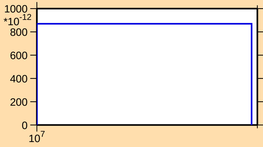
\sigma vs. E for ^{70}\text{Ga}(n,\text{nt})
