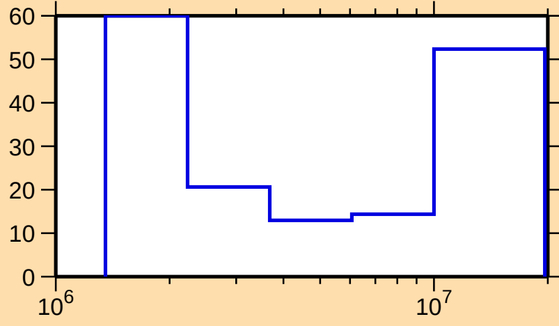
\Delta\sigma/\sigma vs. E for ^{70}\text{Ga}(n,n\text{cont.})
