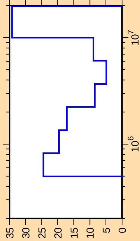
\Delta\sigma/\sigma vs. E for ^{70}\text{Ga}(\text{n,inel.})
