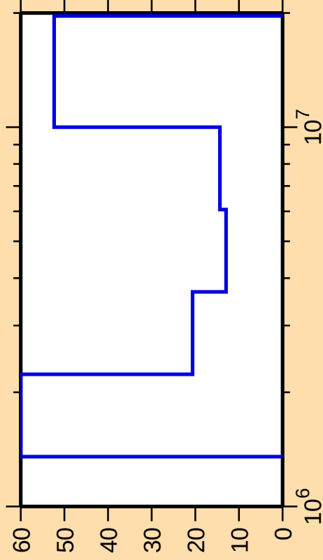
\Delta\sigma/\sigma vs. E for ^{70}\text{Ga}(n,\text{ncont.})
