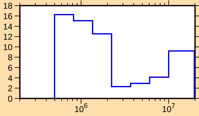
\Delta\sigma/\sigma vs. E for ^{70}\text{Ga}(n,\text{tot.})
