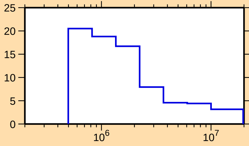
\Delta\sigma/\sigma vs. E for ^{70}\text{Ga}(\text{n,nonel.})
