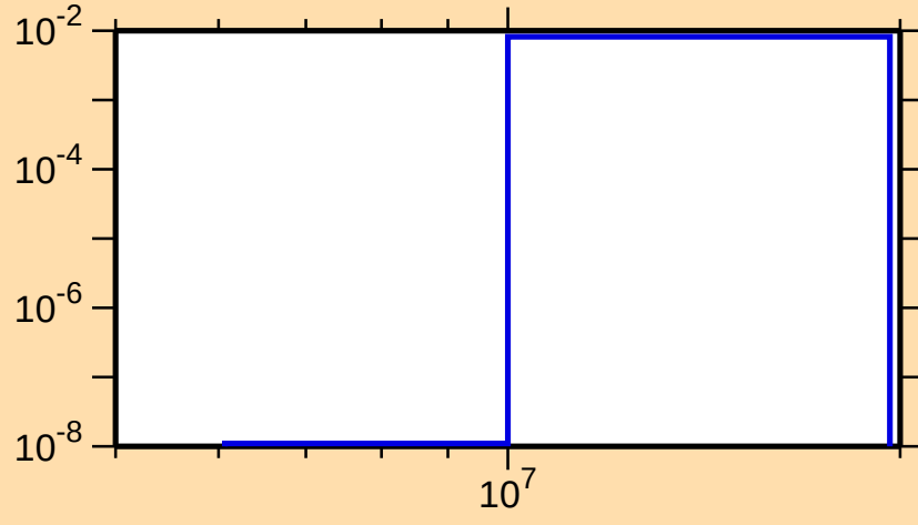
\sigma vs. E for ^{70}\text{Ga}(n,n\alpha)
