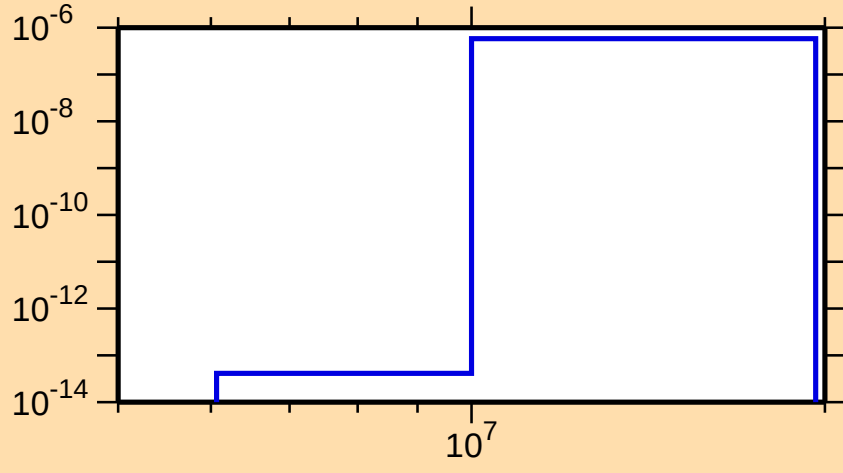
\sigma vs. E for ^{70}\text{Ga}(n,p\alpha)
