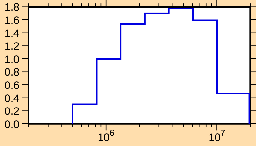
\sigma vs. E for ^{70}\text{Ga}(\text{n,inel.})
