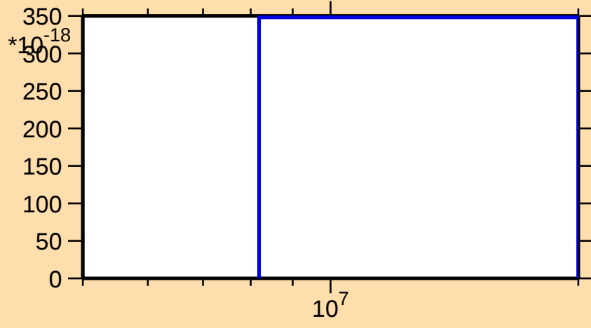
\sigma vs. E for ^{70}\text{Ga}(n,\text{pd})
