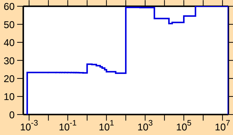
\Delta\sigma/\sigma vs. E for ^{70}\text{Ga}(n,\gamma)
