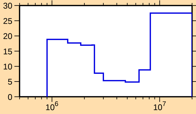
\Delta\sigma/\sigma vs. E for ^{70}\text{Ga}(n,\text{inel.})
