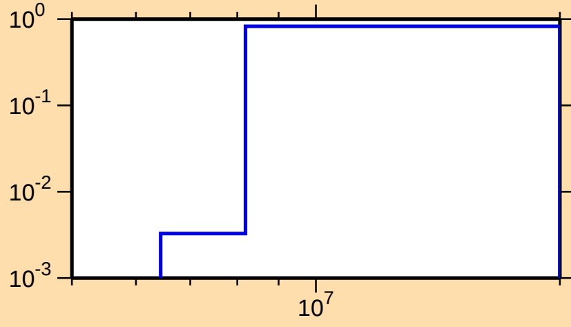
\sigma vs. E for ^{70}\text{Ga}(n,2n)
