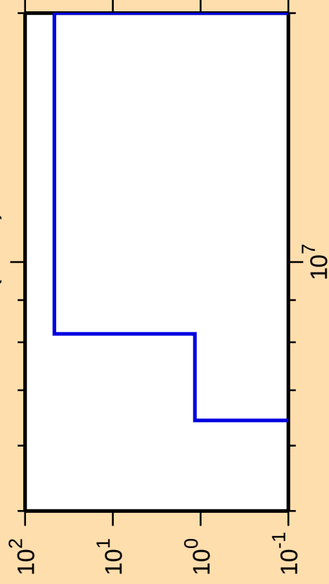
\Delta\sigma/\sigma vs. E for ^{70}\text{Ga}(n,n\alpha)
