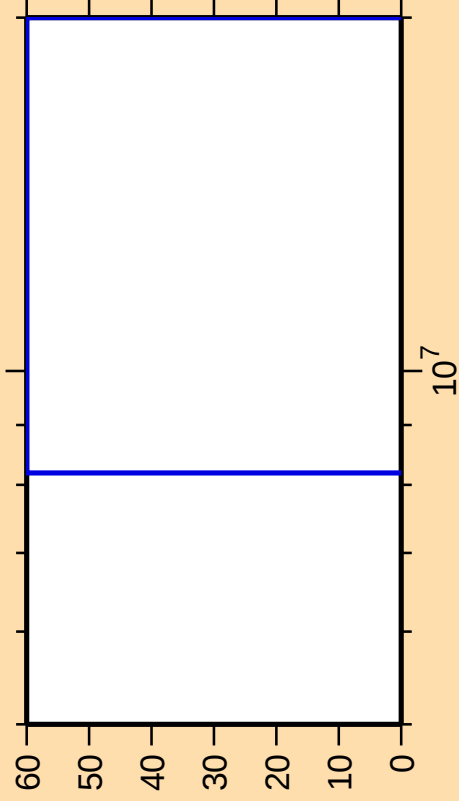
\Delta\sigma/\sigma vs. E for ^{70}\text{Ga}(n,2np)
