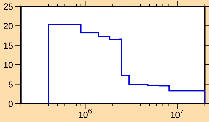
\Delta\sigma/\sigma vs. E for ^{70}\text{Ga}(n,\text{nonel.})
