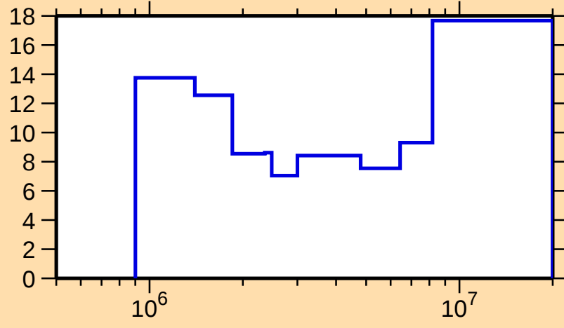
\Delta\sigma/\sigma vs. E for ^{70}\text{Ga}(n,\text{el.})
