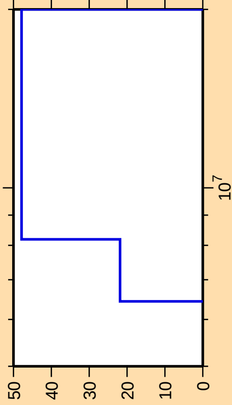
\Delta\sigma/\sigma vs. E for ^{70}\text{Ga}(n,np)
