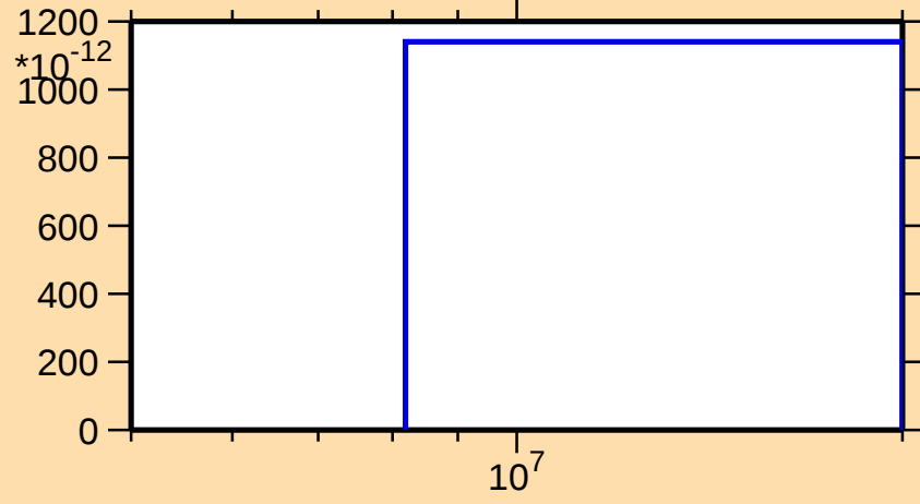
\sigma vs. E for ^{70}\text{Ga}(n,\text{nt})
