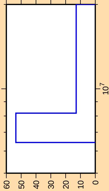
\Delta\sigma/\sigma vs. E for ^{70}\text{Ga}(n,2n)
