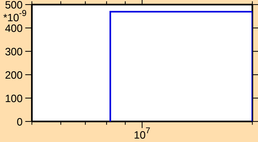
\sigma vs. E for ^{70}\text{Ga}(n,p\alpha)
