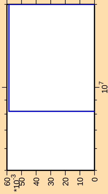
\Delta\sigma/\sigma vs. E for ^{70}\text{Ga}(\text{mt117})
