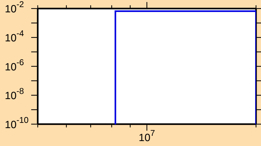
\sigma vs. E for ^{70}\text{Ga}(n,n\alpha)
