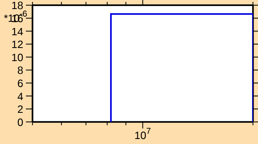
\sigma vs. E for ^{70}\text{Ga}(n,2np)
