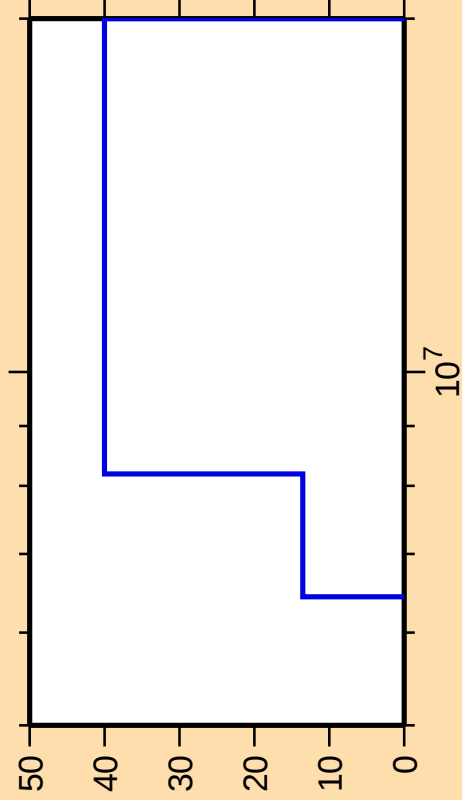
\Delta\sigma/\sigma vs. E for ^{70}\text{Ga}(n,n\text{cont.})
