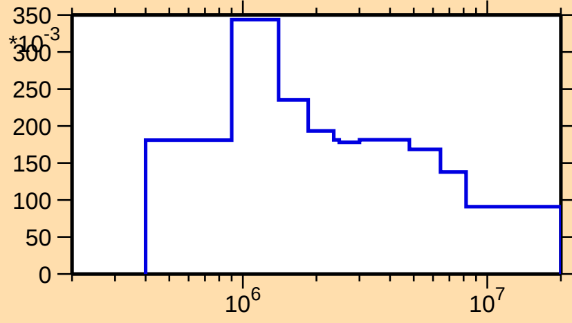
\sigma vs. E for ^{70}\text{Ga}(n,n_1)
