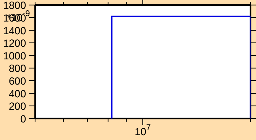
\sigma vs. E for ^{70}\text{Ga}(n,3n)
