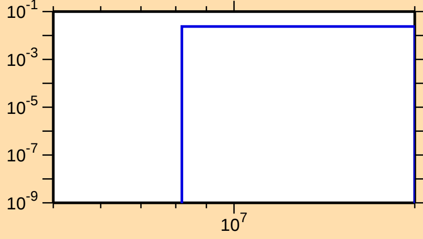
\sigma vs. E for ^{70}\text{Ga}(n,np)
