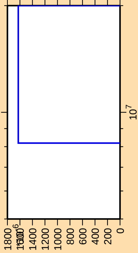
\Delta\sigma/\sigma vs. E for ^{70}\text{Ga}(n,\text{pd})
