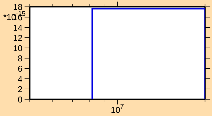
\sigma vs. E for ^{70}\text{Ga}(\text{mt117})
