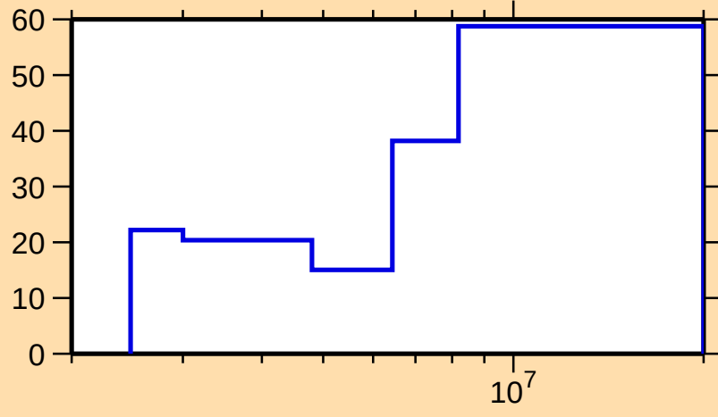
\Delta\sigma/\sigma vs. E for ^{76}\text{Ga}(n,n\text{cont.})
