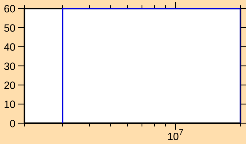
\Delta\sigma/\sigma vs. E for ^{76}\text{Ga}(n,p)
