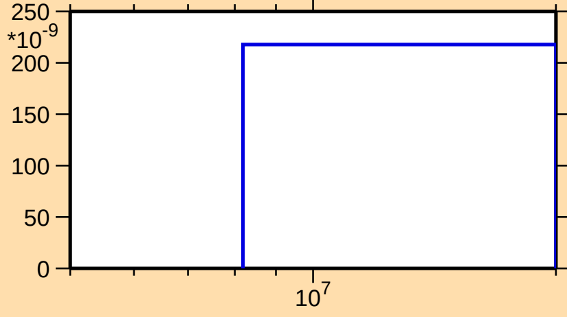
\sigma vs. E for ^{76}\text{Ga}(n,\text{nd})
