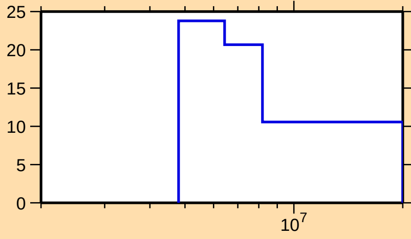
\Delta\sigma/\sigma vs. E for ^{76}\text{Ga}(n,2n)
