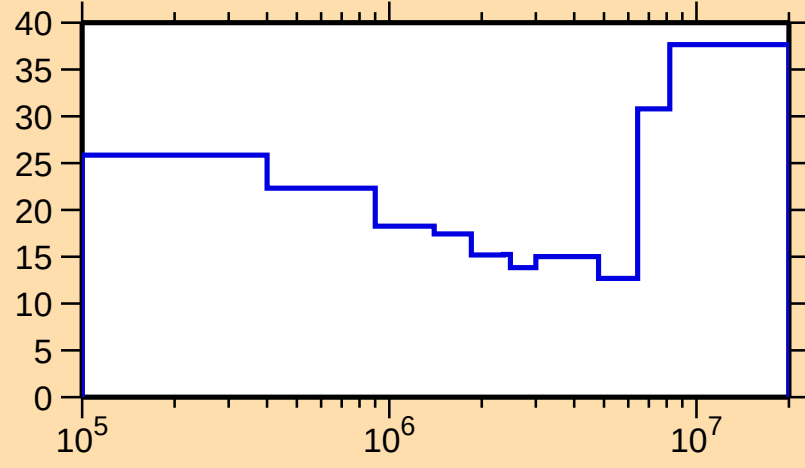
\Delta\sigma/\sigma vs. E for ^{76}\text{Ga}(n,\text{inel.})
