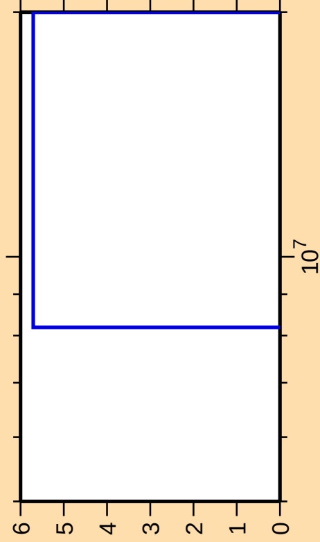
\Delta\sigma/\sigma vs. E for ^{76}\text{Ga}(n,2n\alpha)
