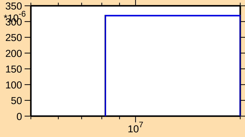
\sigma vs. E for ^{76}\text{Ga}(n,d)
