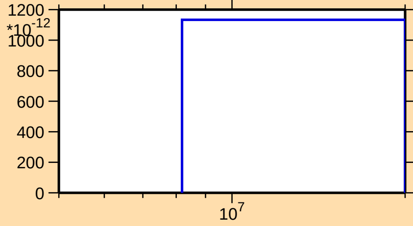
\sigma vs. E for ^{76}\text{Ga}(n,\text{nt})
