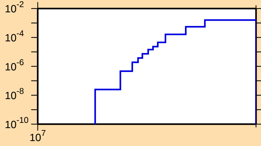
\sigma vs. E for ^{77}\text{Ga}(n,np)
