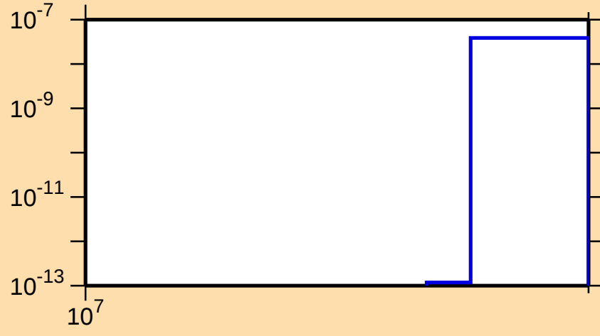
\sigma vs. E for ^{77}\text{Ga}(n,\text{nd})
