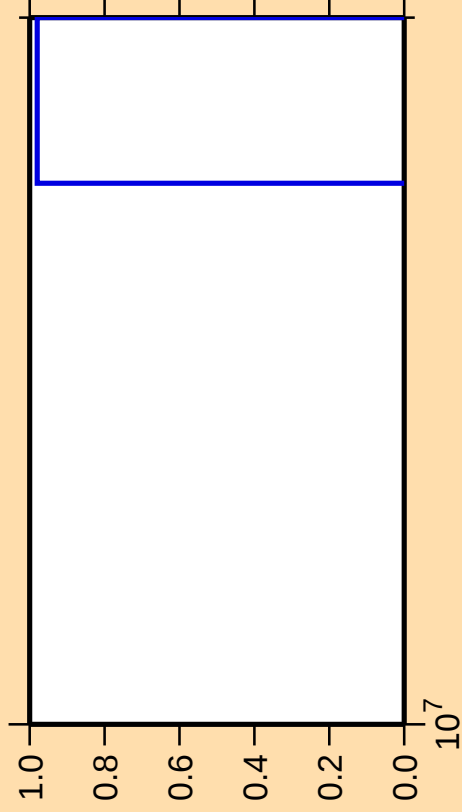
\Delta\sigma/\sigma vs. E for ^{77}\text{Ga}(n,2np)
