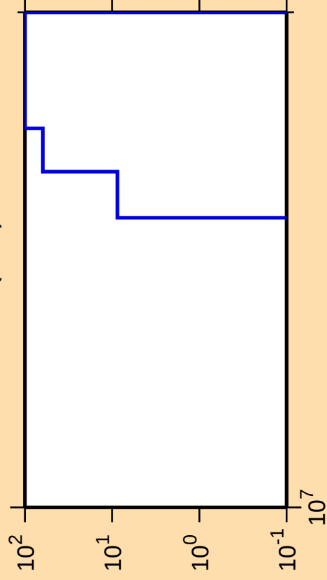
\Delta\sigma/\sigma vs. E for ^{77}\text{Ga}(n,\text{nt})
