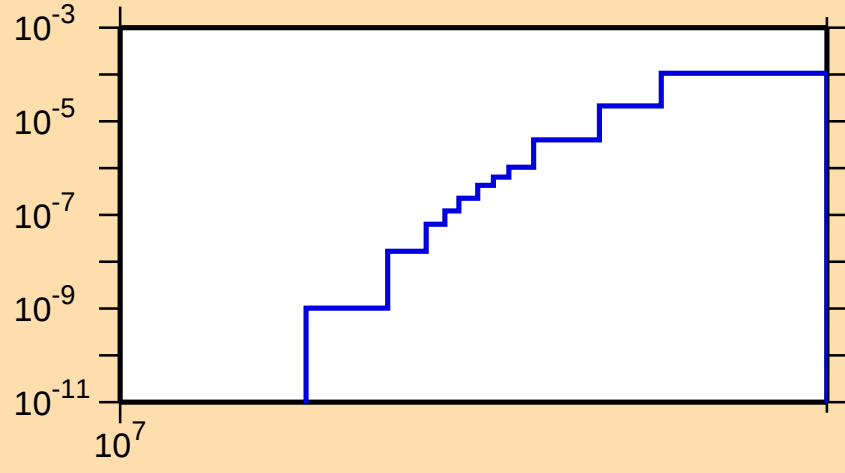
\sigma vs. E for ^{77}\text{Ga}(n,t)
