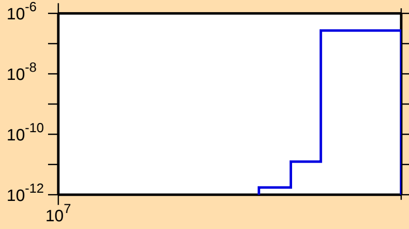
\sigma vs. E for ^{77}\text{Ga}(n,\text{nt})
