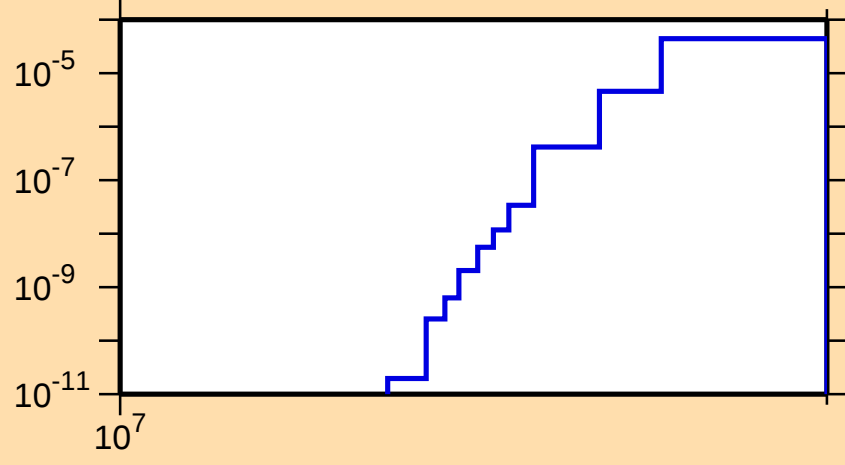
\sigma vs. E for ^{77}\text{Ga}(n,n\alpha)
