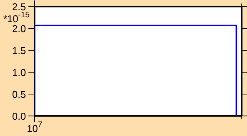
\sigma vs. E for ^{77}\text{Ga}(n,2np)
