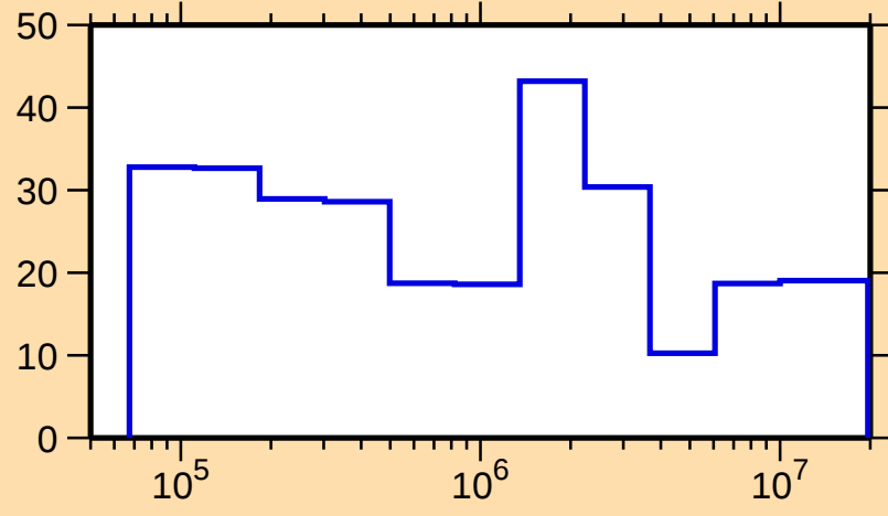
\Delta\sigma/\sigma vs. E for ^{77}\text{Ga}(\text{n,el.})
