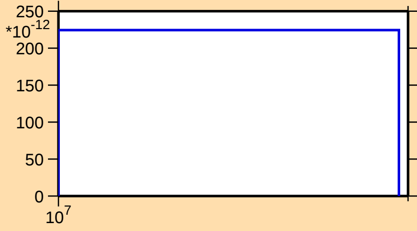
\sigma vs. E for ^{77}\text{Ga}(n,\text{nd})
