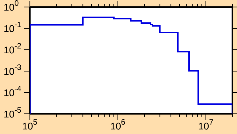
\sigma vs. E for ^{77}\text{Ga}(n,n_2)
