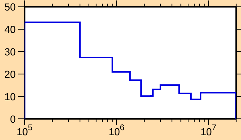
\Delta\sigma/\sigma vs. E for ^{77}\text{Ga}(\text{n,nonel.})
