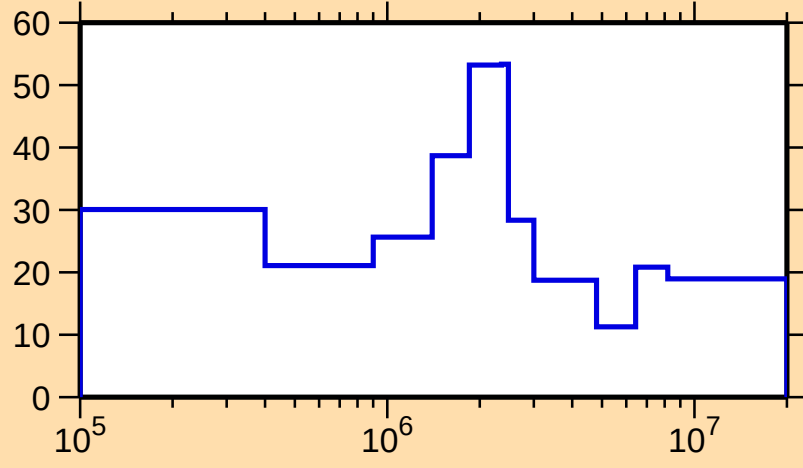
\Delta\sigma/\sigma vs. E for ^{77}\text{Ga}(\text{n,el.})
