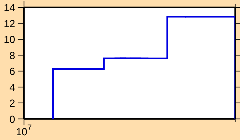
\Delta\sigma/\sigma vs. E for ^{135}\text{Gd}(n,\text{el.})
