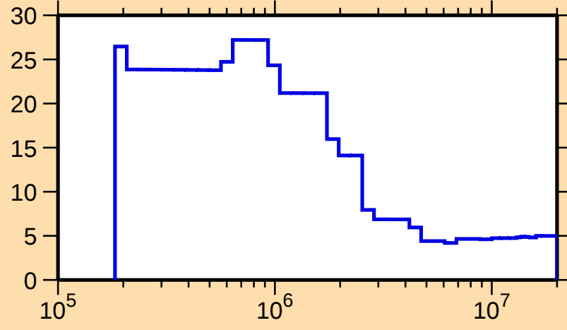
\Delta\sigma/\sigma vs. E for ^{135}\text{Gd}(n,\text{nonel.})
