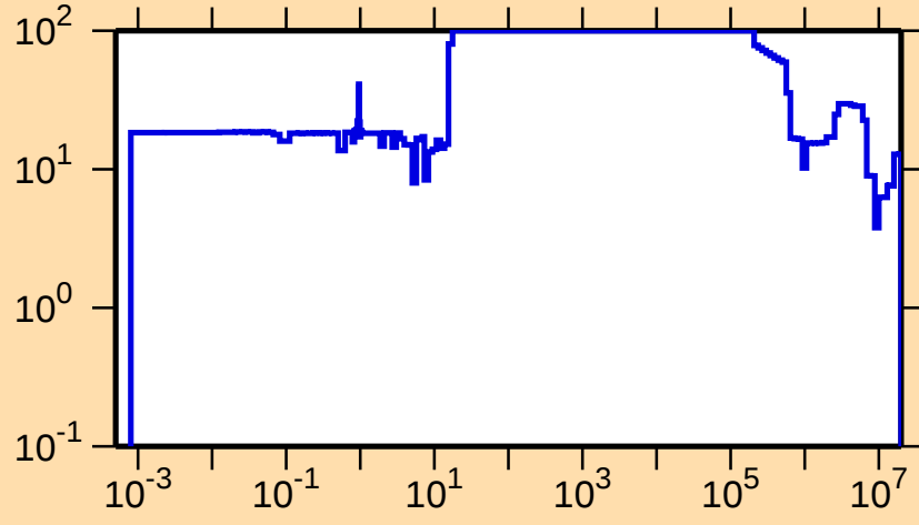
\Delta\sigma/\sigma vs. E for ^{135}\text{Gd}(n,\text{el.})
