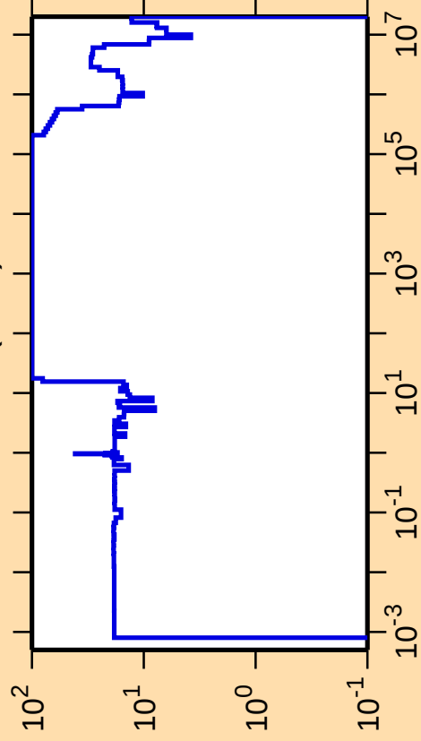
\Delta\sigma/\sigma vs. E for ^{135}\text{Gd}(n,\text{el.})
