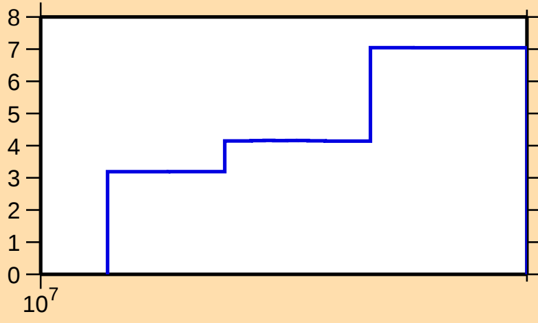
\Delta\sigma/\sigma vs. E for ^{135}\text{Gd}(n,\text{tot.})
