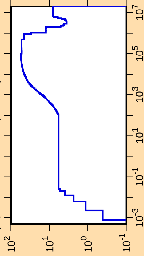
\Delta\mu/\mu vs. E for ^{137}\text{Gd}(\text{mt251})
