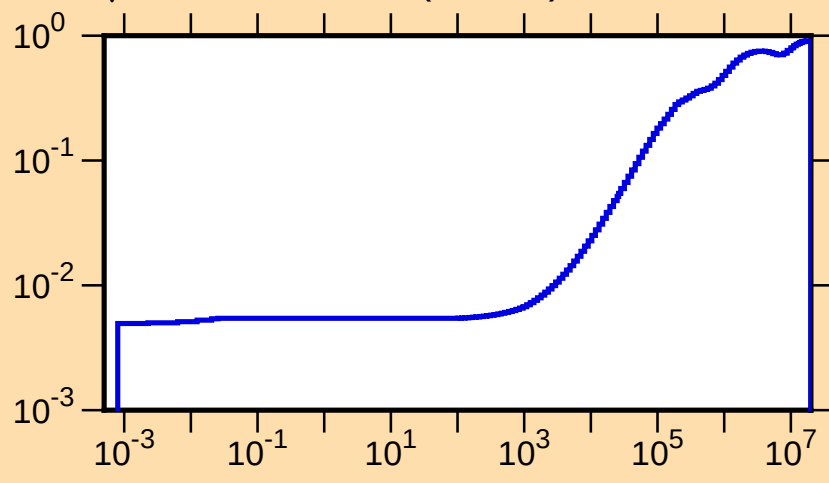
\mu vs. E for ^{137}\text{Gd}(\text{mt251})
