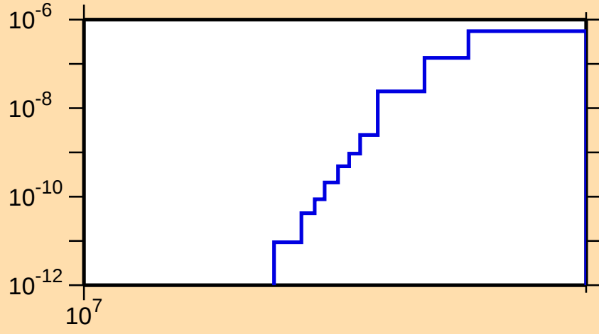
\sigma vs. E for ^{137}\text{Gd}(n,2n\alpha)
