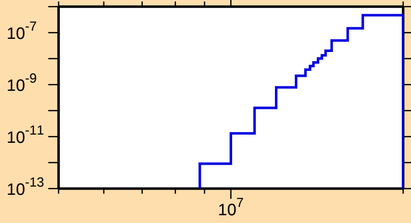
\sigma vs. E for ^{137}\text{Gd}(\text{mt117})
