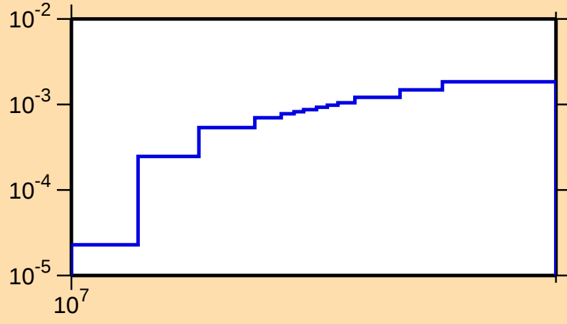
\sigma vs. E for ^{137}\text{Gd}(n,2n)
