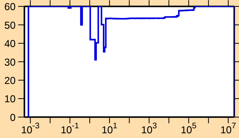
\Delta\sigma/\sigma vs. E for ^{137}\text{Gd}(n,\gamma)
