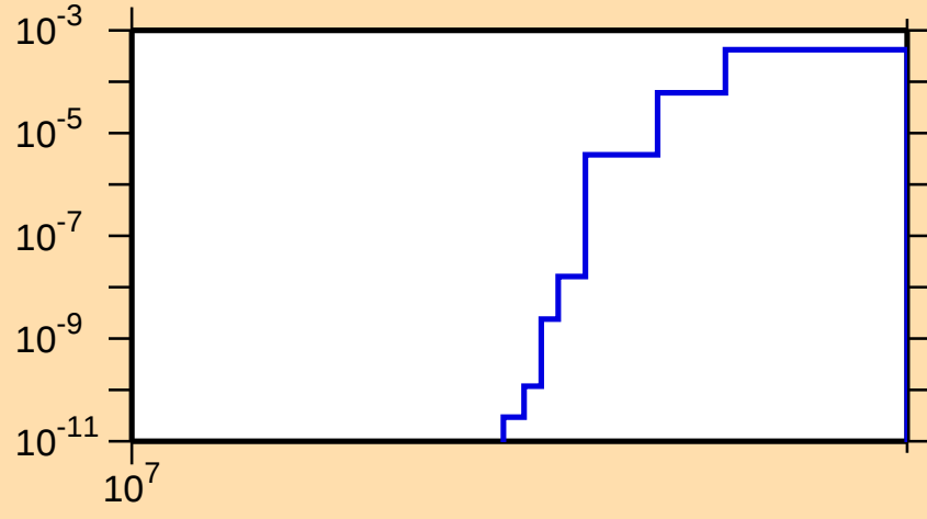
\sigma vs. E for ^{137}\text{Gd}(n,2np)
