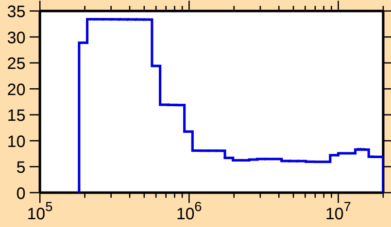
\Delta\sigma/\sigma vs. E for ^{137}\text{Gd}(n,\text{nonel.})
