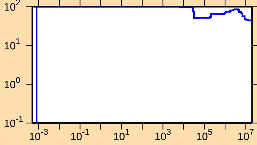
\Delta\sigma/\sigma vs. E for ^{137}\text{Gd}(n,p)
