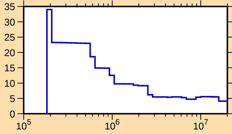
\Delta\sigma/\sigma vs. E for ^{137}\text{Gd}(n,\text{tot.})
