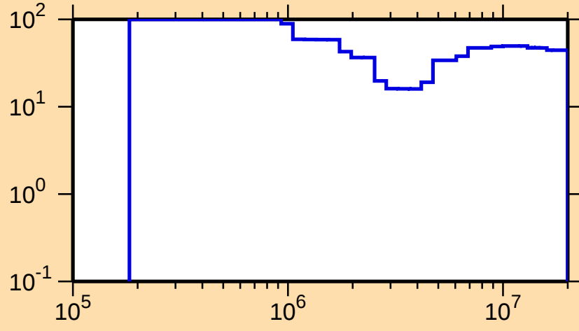
\Delta\sigma/\sigma vs. E for ^{137}\text{Gd}(n,\text{inel.})
