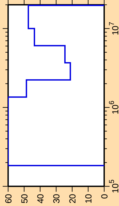
\Delta\sigma/\sigma vs. E for ^{137}\text{Gd}(n,\text{inel.})
