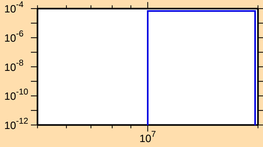
\sigma vs. E for ^{137}\text{Gd}(n,\text{pt})
