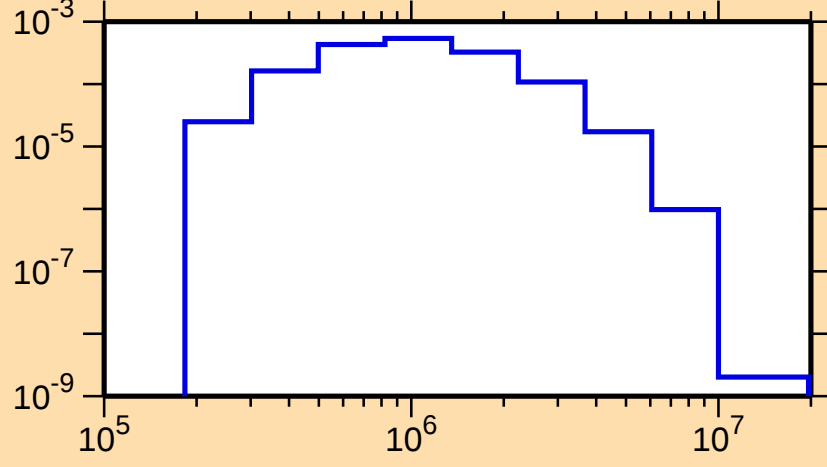
\sigma vs. E for ^{137}\text{Gd}(n,n_1)
