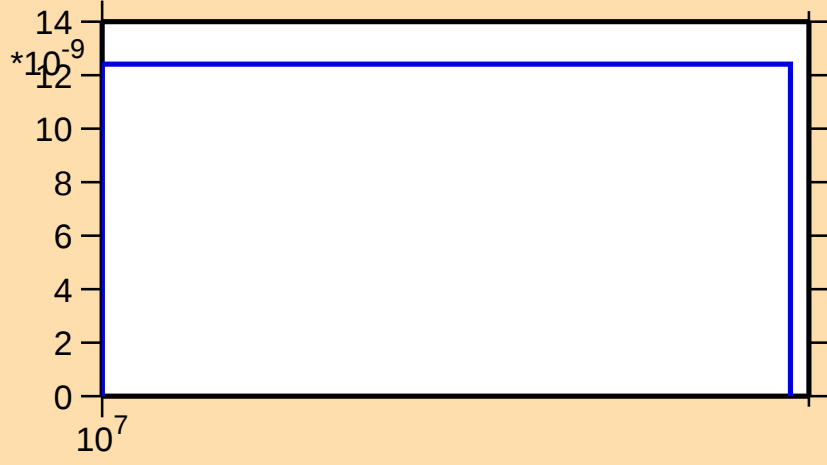
\sigma vs. E for ^{137}\text{Gd}(n,\text{nd})
