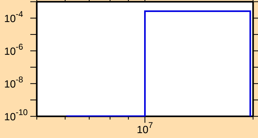
\sigma vs. E for ^{137}\text{Gd}(n,t)
