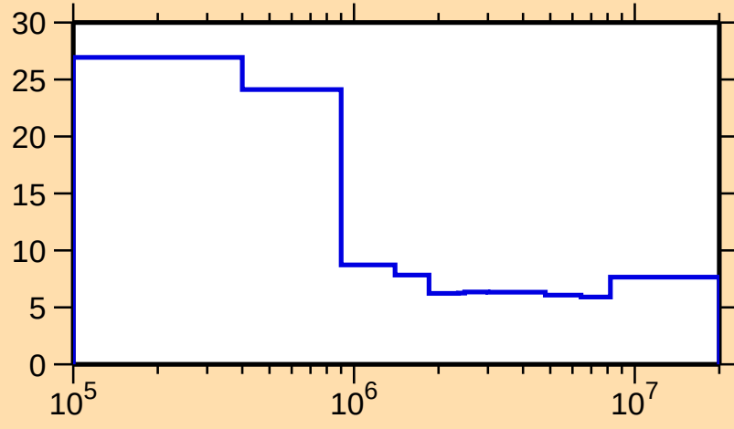
\Delta\sigma/\sigma vs. E for ^{137}\text{Gd}(n,\text{nonel.})
