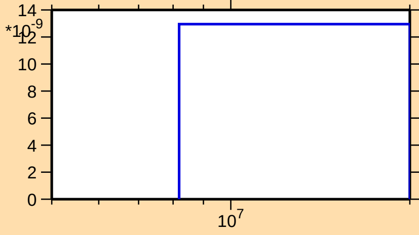
\sigma vs. E for ^{137}\text{Gd}(n,2n\alpha)
