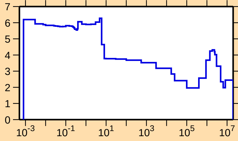
\sigma vs. E for ^{137}\text{Gd}(n,\text{el.})
