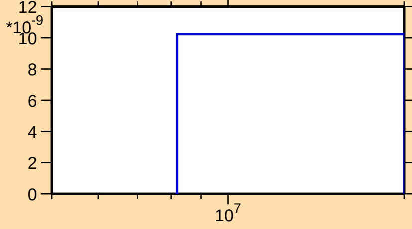
\sigma vs. E for ^{137}\text{Gd}(n,\text{nd})
