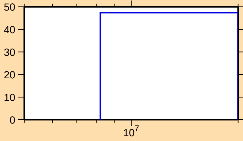
\Delta\sigma/\sigma vs. E for ^{137}\text{Gd}(n,\text{inel.})
