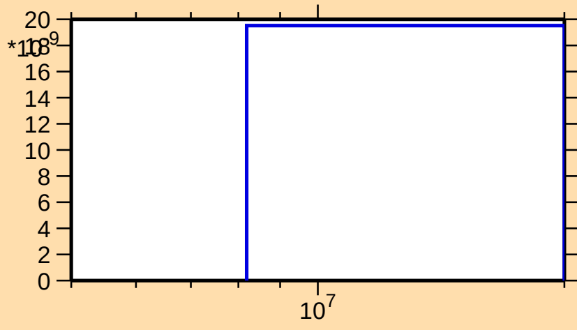
\sigma vs. E for ^{137}\text{Gd}(\text{mt117})
