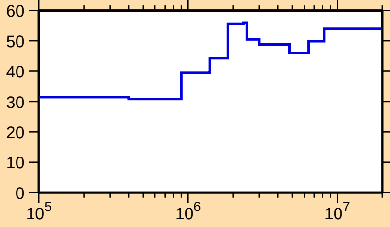
\Delta\sigma/\sigma vs. E for ^{137}\text{Gd}(n,n_1)
