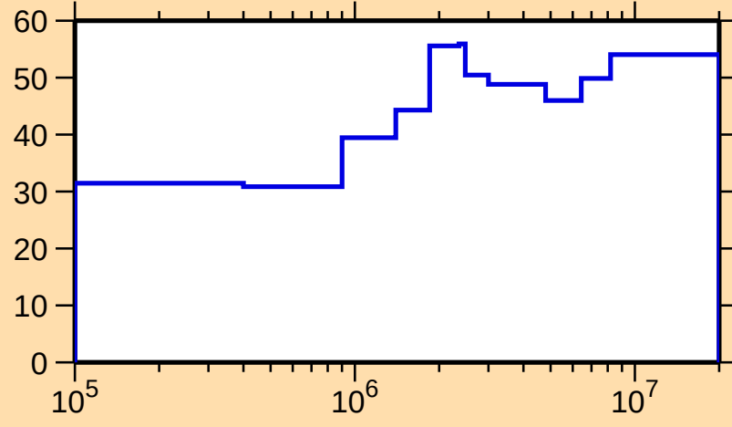
\Delta\sigma/\sigma vs. E for ^{137}\text{Gd}(n,n_1)
