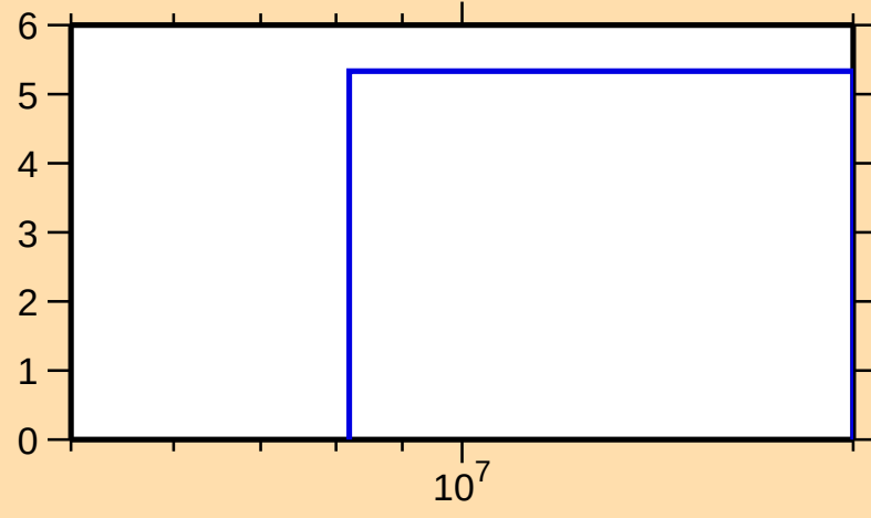
\Delta\sigma/\sigma vs. E for ^{137}\text{Gd}(n,\text{tot.})
