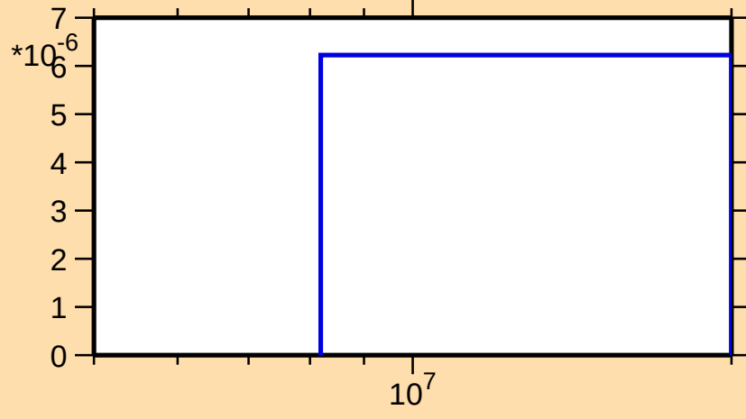
\sigma vs. E for ^{137}\text{Gd}(n,2np)
