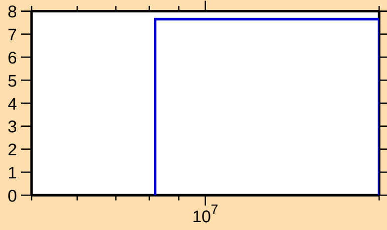
\Delta\sigma/\sigma vs. E for ^{137}\text{Gd}(n,\text{nonel.})
