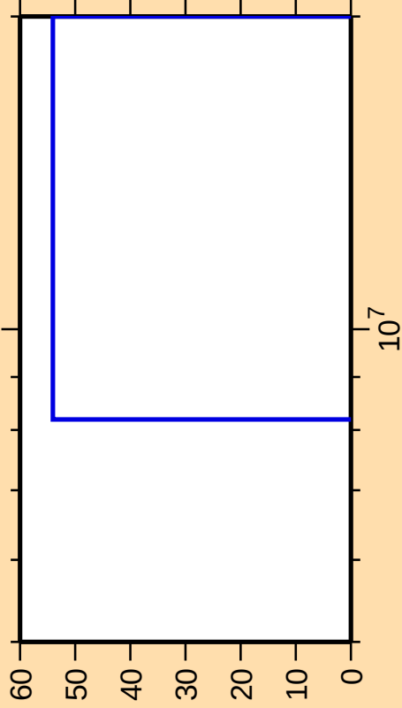
\Delta\sigma/\sigma vs. E for ^{137}\text{Gd}(n,n_1)
