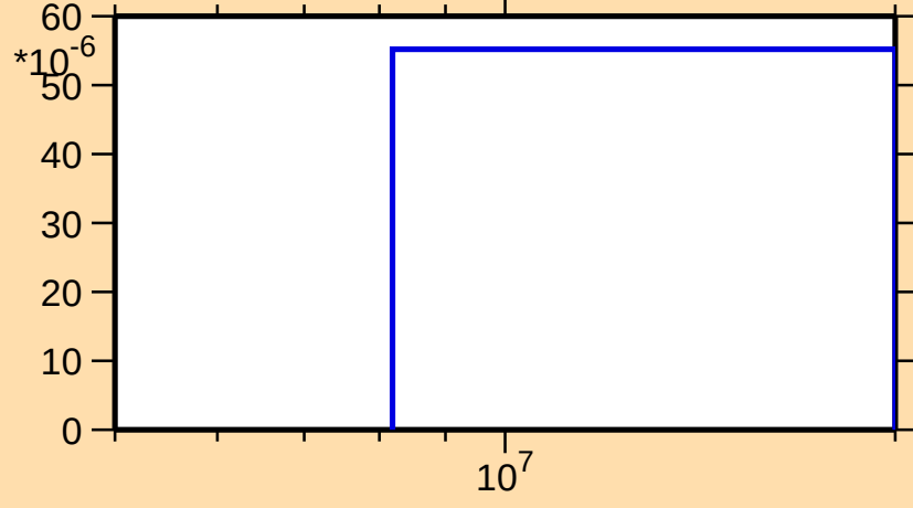
\sigma vs. E for ^{137}\text{Gd}(n,\text{pt})
