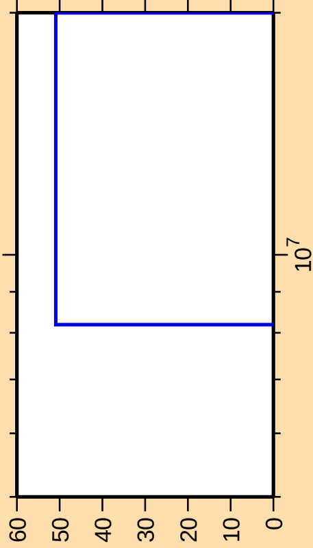
\Delta\sigma/\sigma vs. E for ^{137}\text{Gd}(n,2np)
