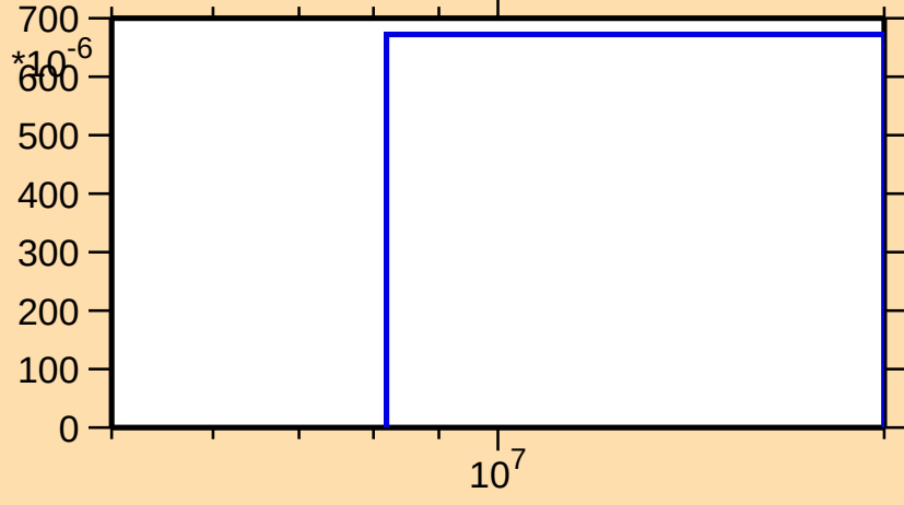
\sigma vs. E for ^{137}\text{Gd}(n,2n)
