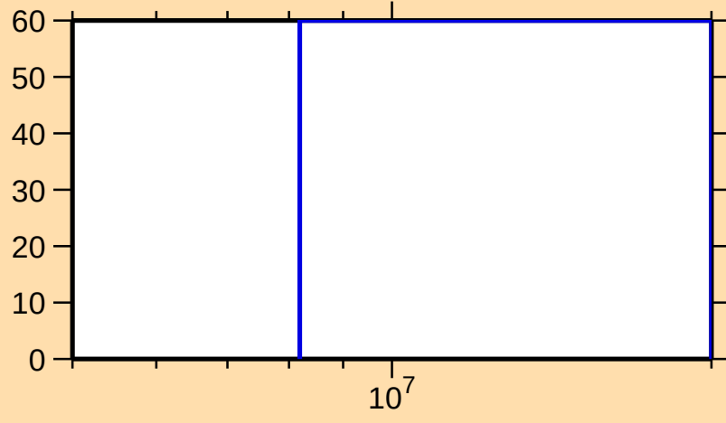
\Delta\sigma/\sigma vs. E for ^{137}\text{Gd}(n,2n)
