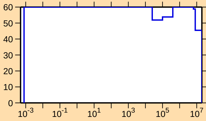
\Delta\sigma/\sigma vs. E for ^{137}\text{Gd}(n,p)
