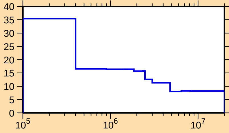
\Delta\sigma/\sigma vs. E for ^{137}\text{Gd}(n,\text{el.})
