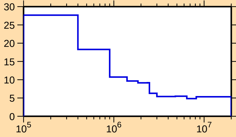
\Delta\sigma/\sigma vs. E for ^{137}\text{Gd}(n,\text{tot.})
