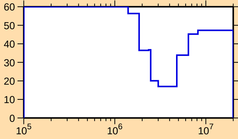
\Delta\sigma/\sigma vs. E for ^{137}\text{Gd}(n,n\text{cont.})
