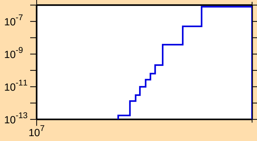
\sigma vs. E for ^{143}\text{Gd}(n,\text{pt})
