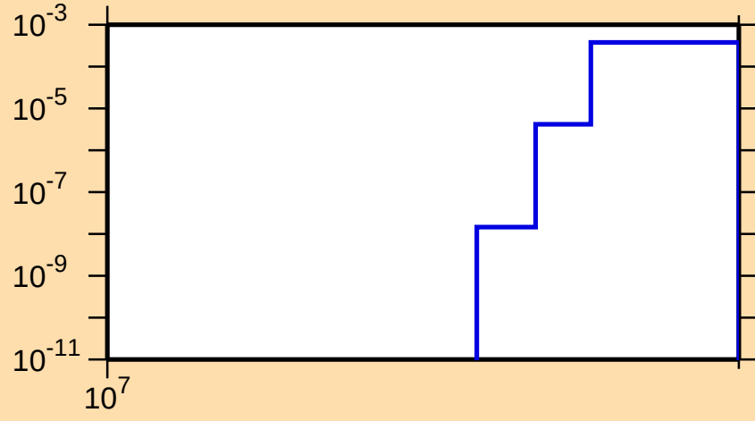
\sigma vs. E for ^{143}\text{Gd}(n,2np)
