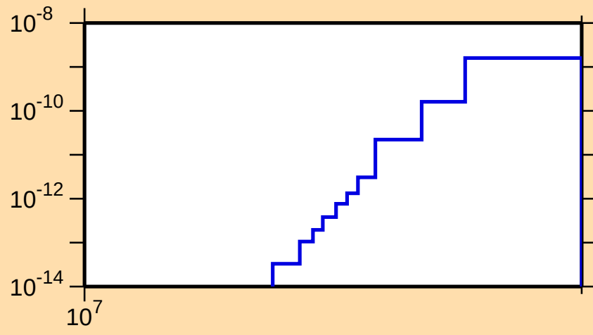
\sigma vs. E for ^{143}\text{Gd}(\text{mt117})
