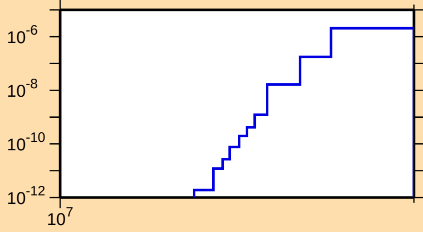
\sigma vs. E for ^{143}\text{Gd}(n,2n\alpha)
