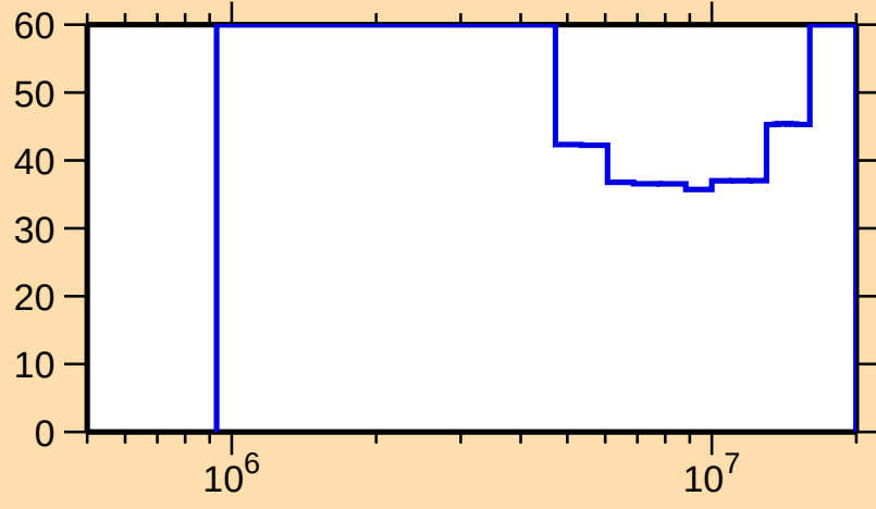
\Delta\sigma/\sigma vs. E for ^{143}\text{Gd}(n,n\text{cont.})
