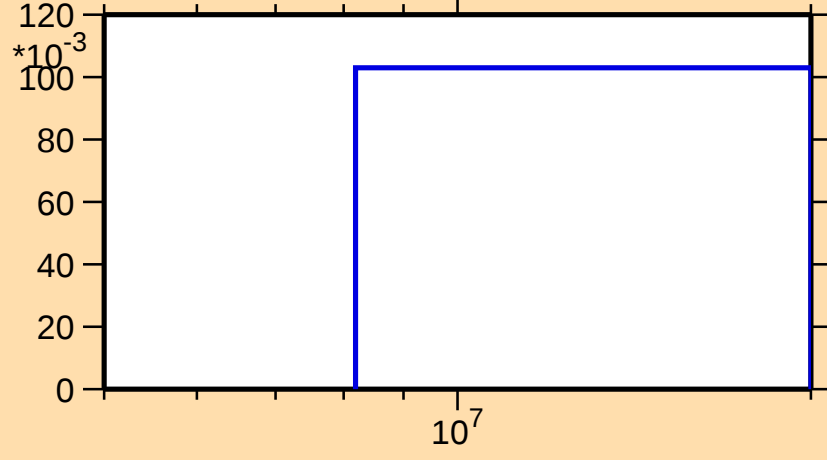
\sigma vs. E for ^{143}\text{Gd}(n,2n)
