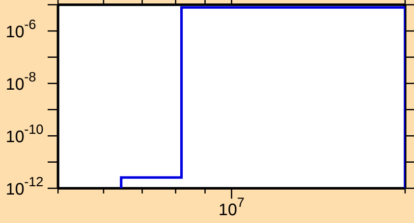
\sigma vs. E for ^{143}\text{Gd}(n,\text{He3})
