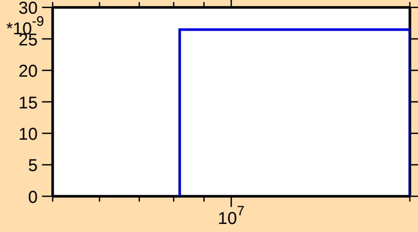
\sigma vs. E for ^{143}\text{Gd}(n,\text{nd})
