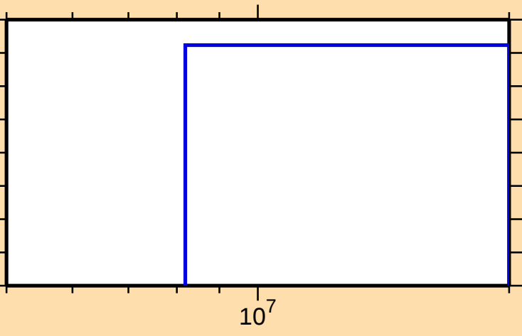
\sigma vs. E for ^{143}\text{Gd}(n,t)
