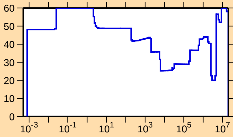
\Delta\sigma/\sigma vs. E for ^{144}\text{Gd}(n,p)
