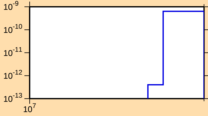
\sigma vs. E for ^{144}\text{Gd}(n,\text{pt})
